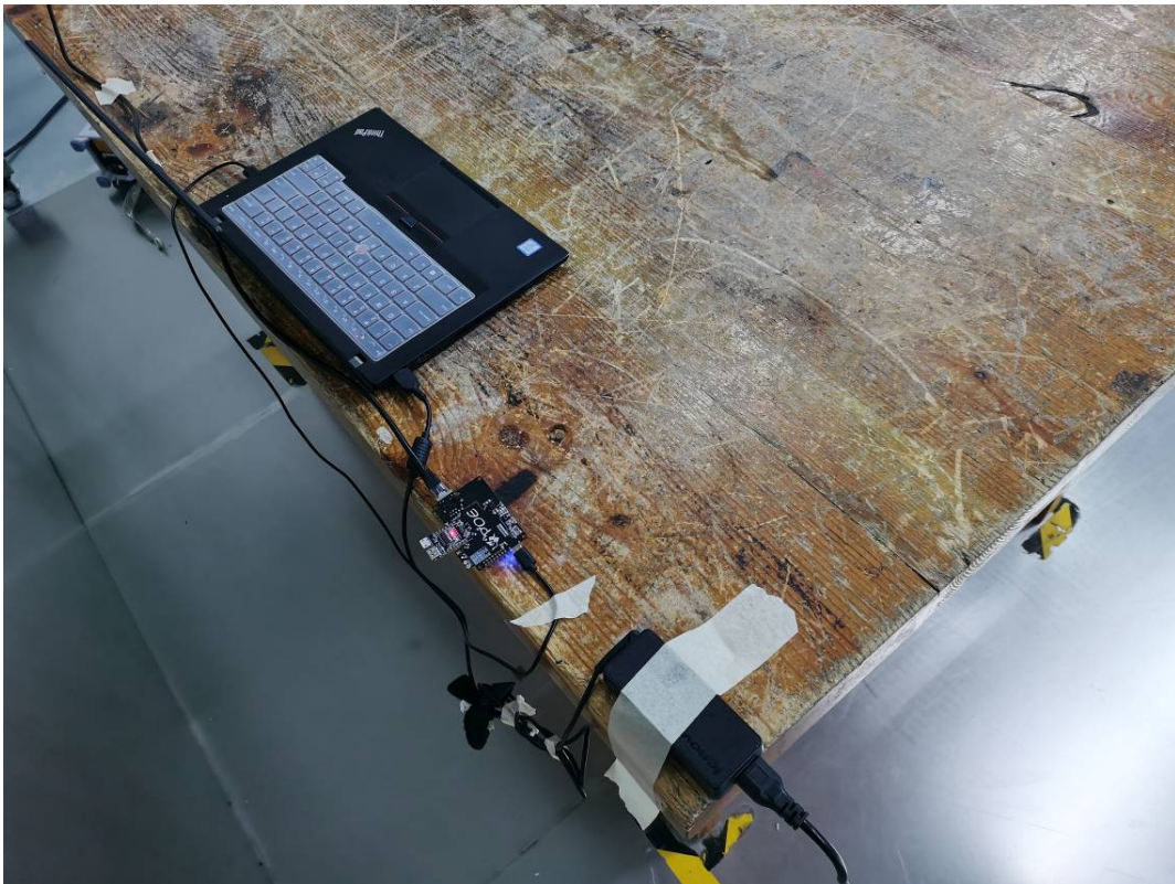
Conducted Emissions Side View-Type C
