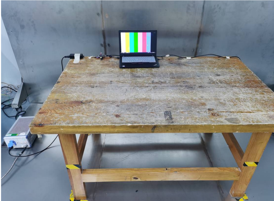
Conducted Emissions Side View-Type C
