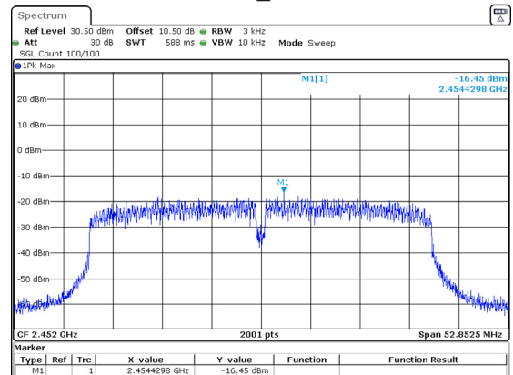
802.11n40_2452MHz
