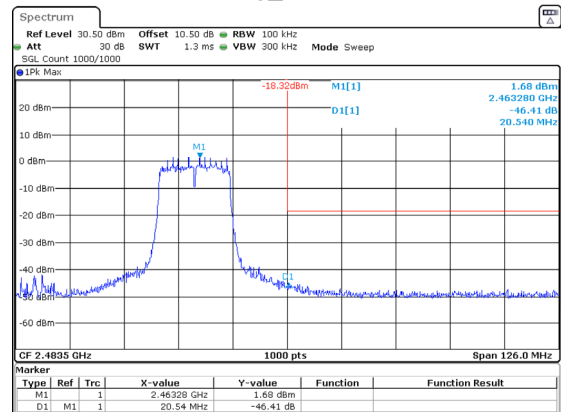
802.11g_2462MHz
