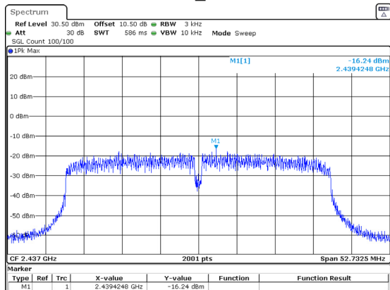
802.11n40_2437MHz
