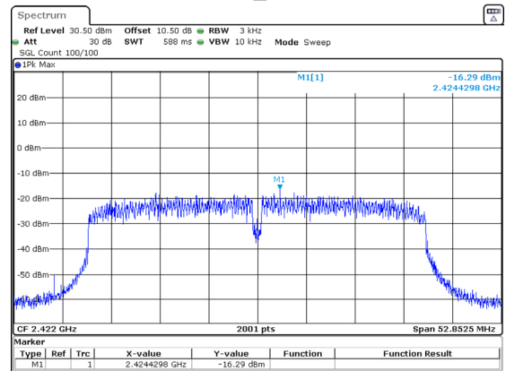
802.11n40_2422MHz
