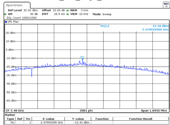
BLE_2M_High_Channel
