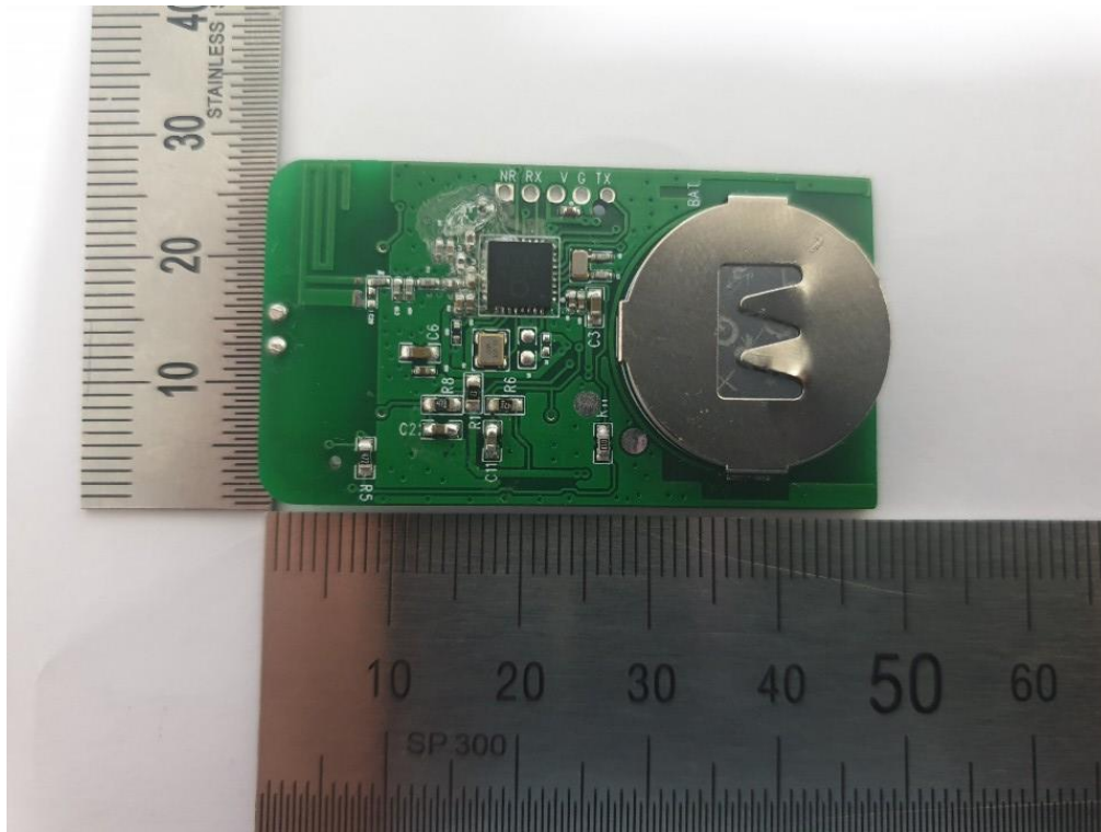
Rear mainboard of Internal Photo
