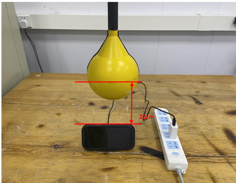
Test Position E - Exposure photo from top surface (20cm) (TM1)
