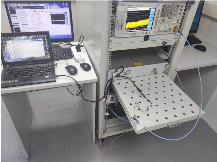
Conducted Test-BT
