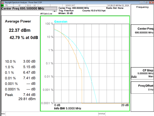
Band71_5MHz_16QAM_RB25_0_CH133447
