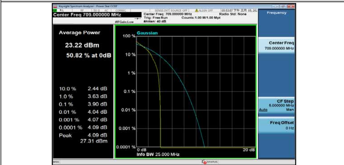
Band17-10MHz-QPSK-23780-50RB#0
