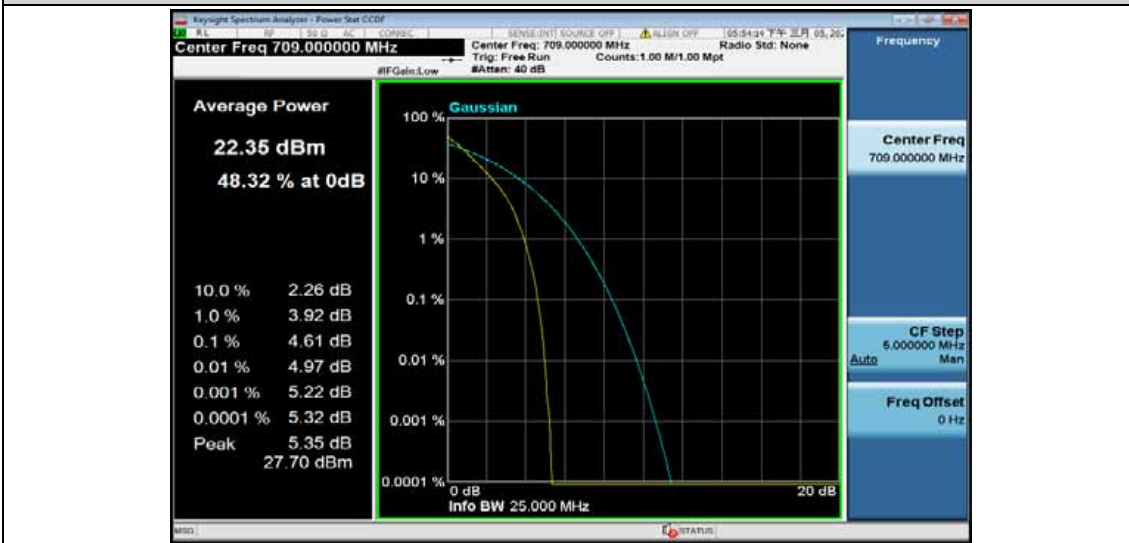
Band17-10MHz-QPSK-23790-1RB#0
