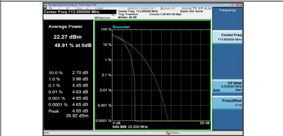
Band17-5MHz-16QAM-23825-25RB#0
