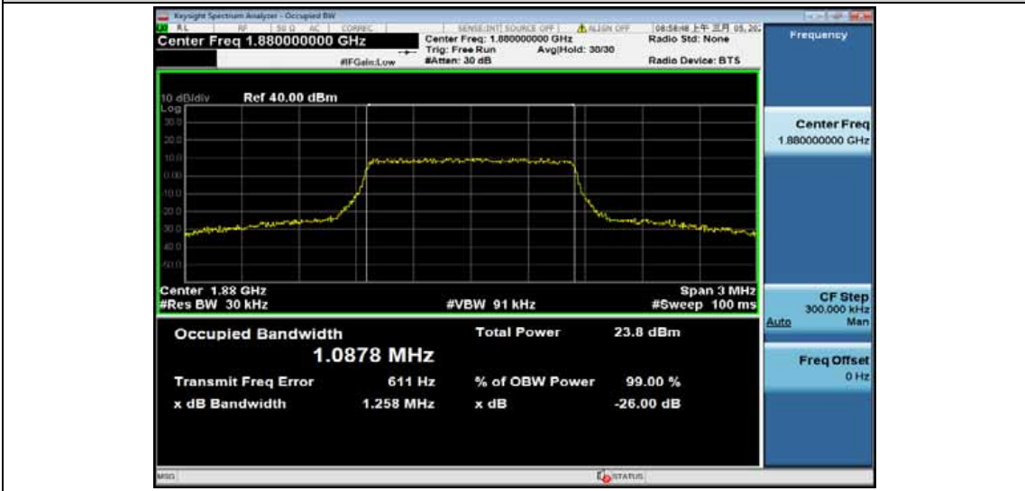
Band2-1.4MHz-16QAM-19193-6RB#0-1.0903
