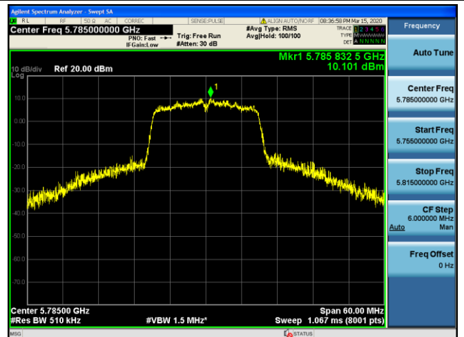
Channel 157 / 5785 MHz
