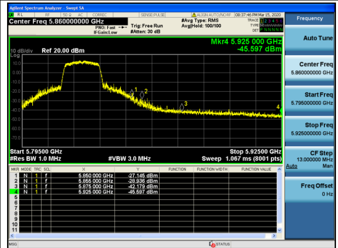
Channel 165 / 5825 MHz – Peak
