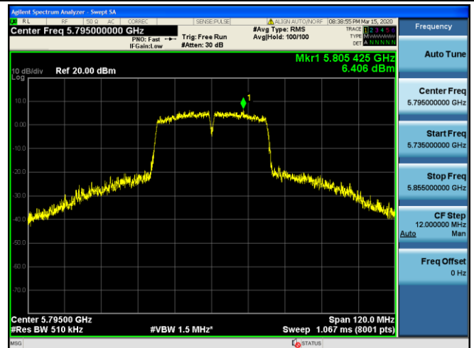
Channel 159 / 5795 MHz
