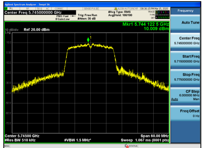
Channel 149 / 5745 MHz
