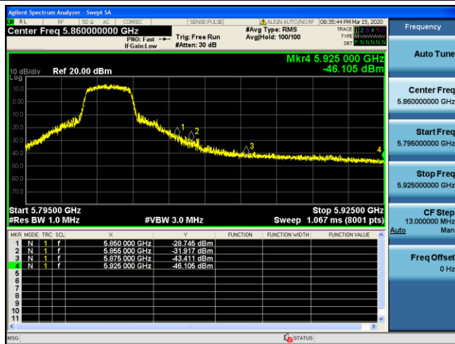
Channel 165 / 5825 MHz – Peak
