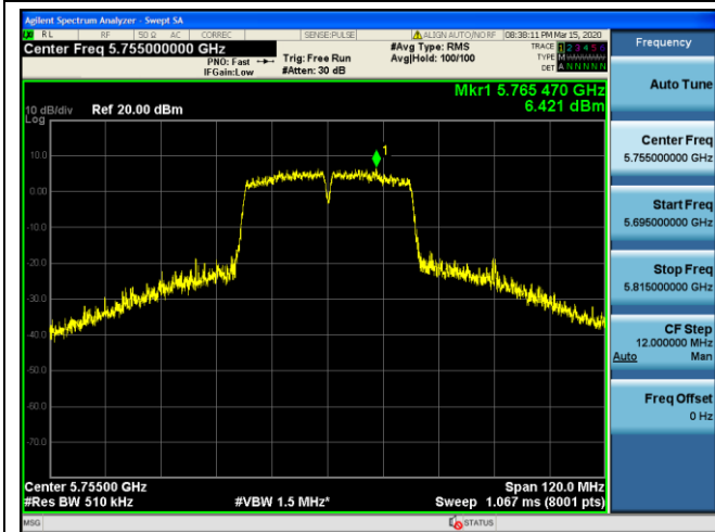
Channel 151 / 5755 MHz
