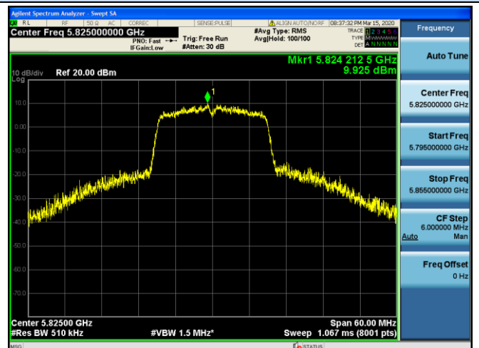
Channel 165 / 5825 MHz
