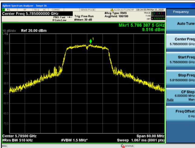
Channel 157 / 5785 MHz
