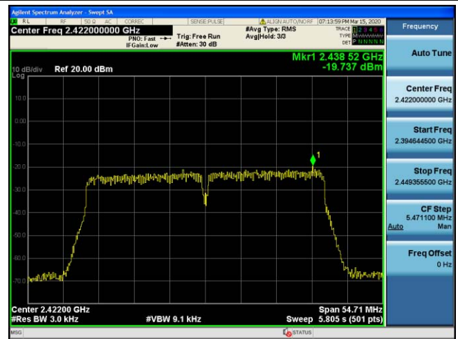
Channel 3 / 2422 MHz
