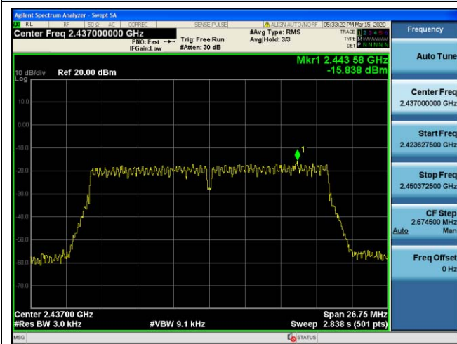
Channel 6 / 2437 MHz
