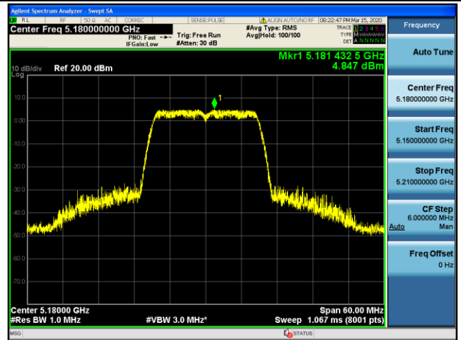
Channel 36 / 5180 MHz
