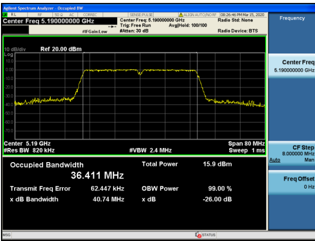
Channel 38 / 5190 MHz
