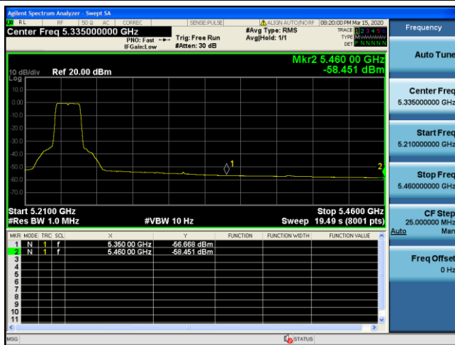
Channel 48 / 5240 MHz – Average
