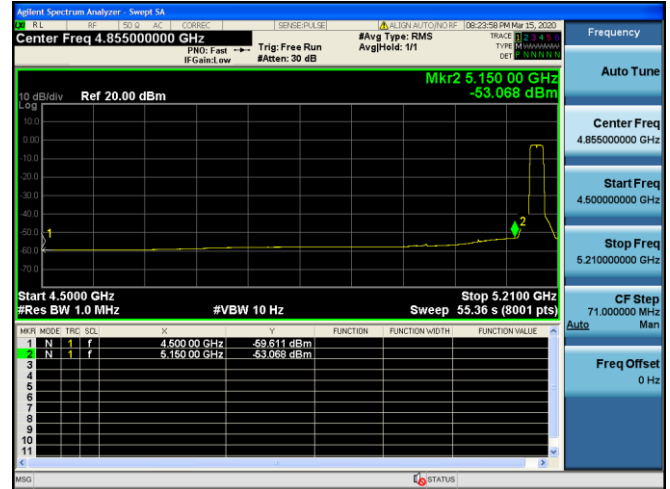
Channel 36 / 5180 MHz – Average
