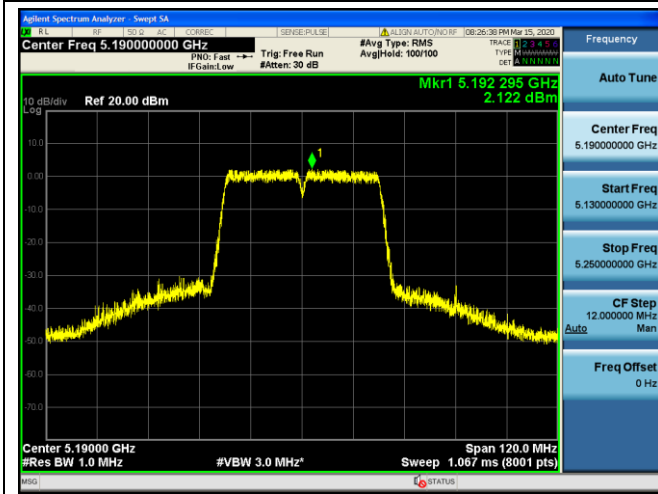
Channel 38 / 5190 MHz
