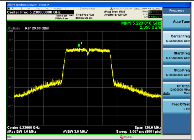
Channel 46 / 5230 MHz
