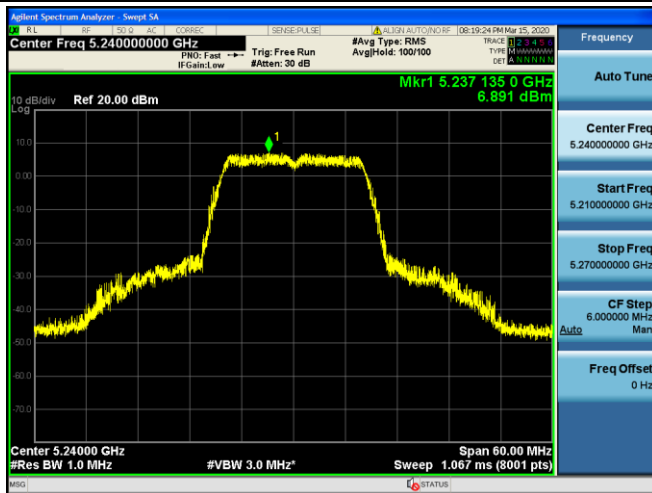
Channel 48 / 5240 MHz
