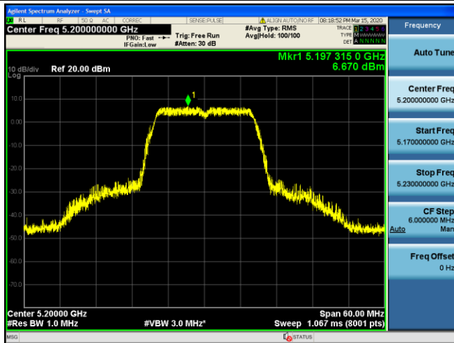
Channel 40 / 5200 MHz
