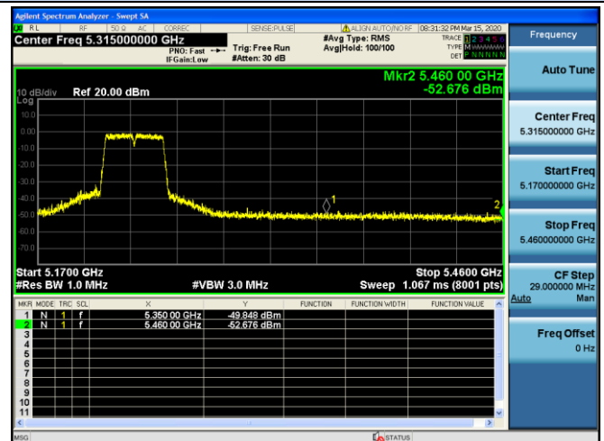
Channel 46 / 5230 MHz – Peak
