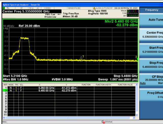
Channel 48 / 5240 MHz – Peak
