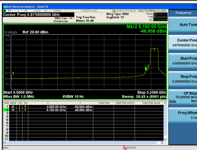
Channel 36 / 5190 MHz – Average
