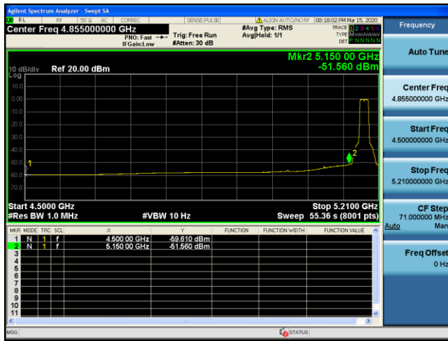
Channel 36 / 5180 MHz – Average
