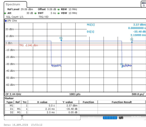
NTNV-BLE_1M-Ant1-2440
