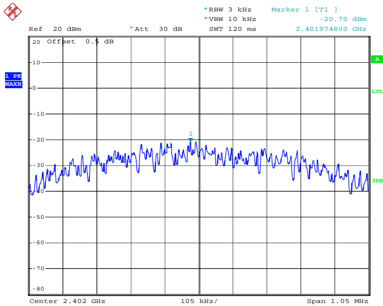
1M Power Spectral Density, Low Channel
