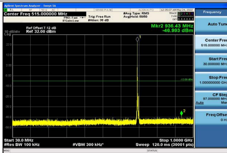
Band12-5MHz-16QAM-23035-1RB#0-30~1000MHz
