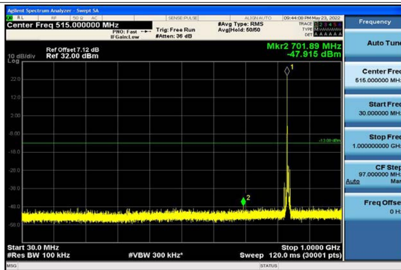
Band5-5MHz-16QAM-20525-1RB#0-30~1000MHz
