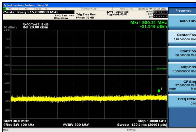
Band7-5MHz-QPSK-21100-1RB#0-30~1000MHz
