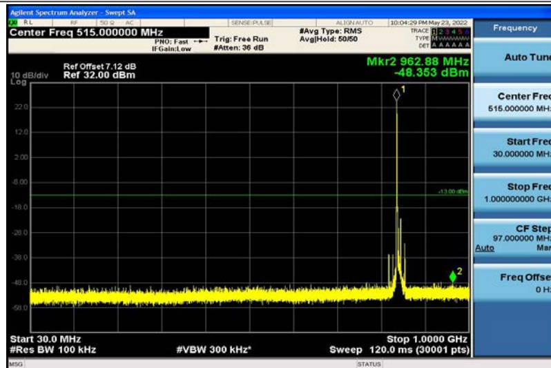
Band5-10MHz-QPSK-20600-1RB#0-30~1000MHz
