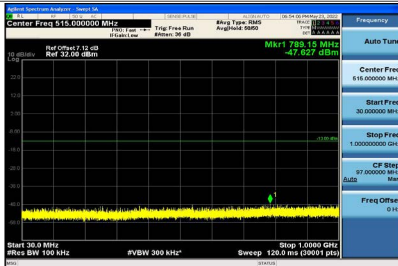
Band4-1.4MHz-16QAM-20393-1RB#0-30~1000MHz
