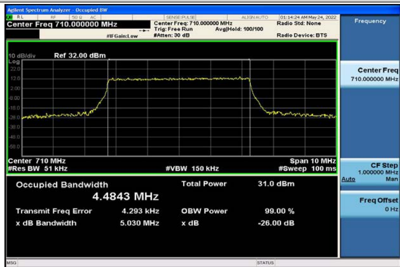
Band17-5MHz-QPSK-23790-25RB#0-4.4843
