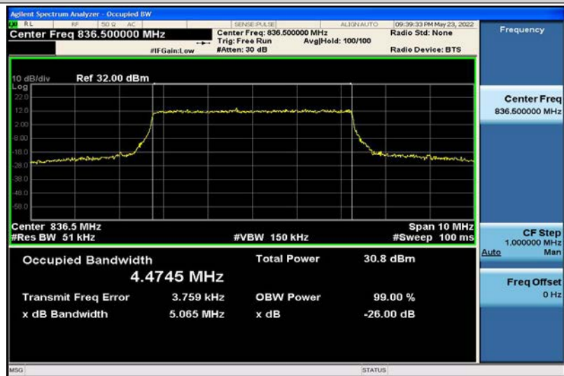
Band5-5MHz-QPSK-20525-25RB#0-4.4745
