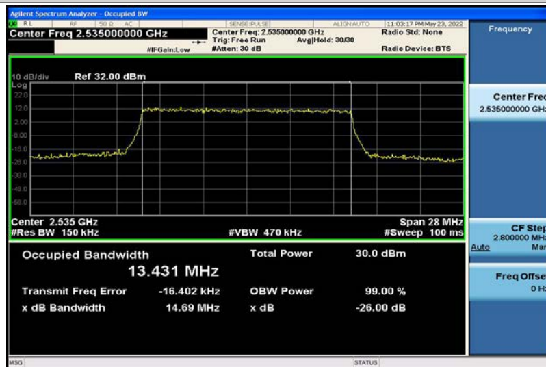
Band7-15MHz-16QAM-21100-75RB#0-13.431
