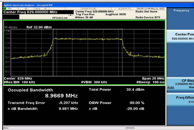
Band5-10MHz-QPSK-20450-50RB#0-8.9669
