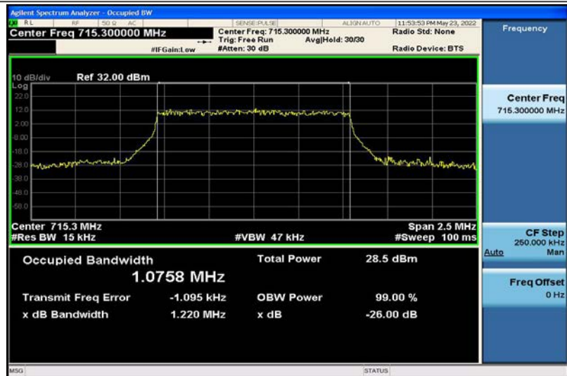
Band12-1.4MHz-16QAM-23173-6RB#0-1.0758
