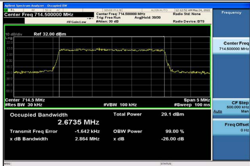
Band12-3MHz-16QAM-23165-15RB#0-2.6735
