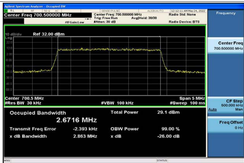
Band12-3MHz-16QAM-23025-15RB#0-2.6716
