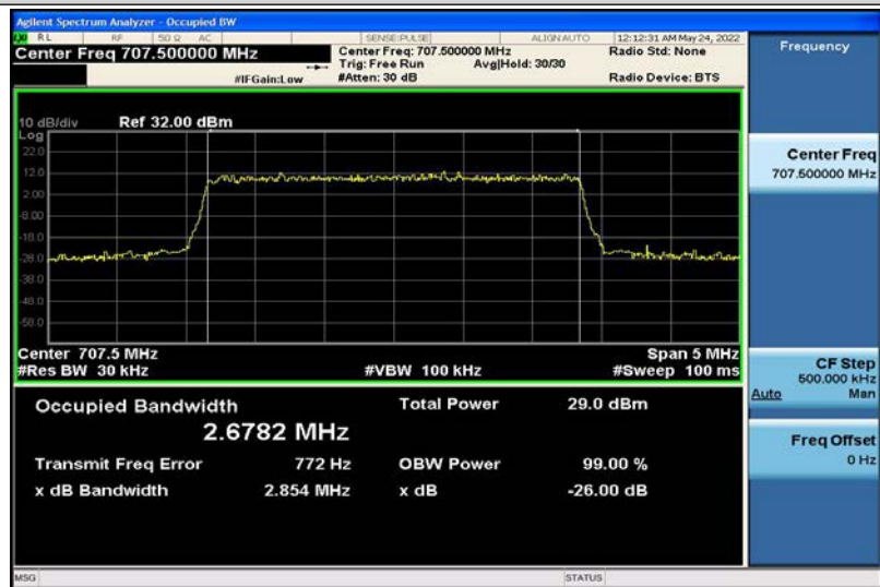
Band12-3MHz-16QAM-23095-15RB#0-2.6782
