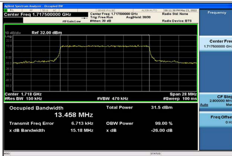
Band4-15MHz-QPSK-20025-75RB#0-13.458
