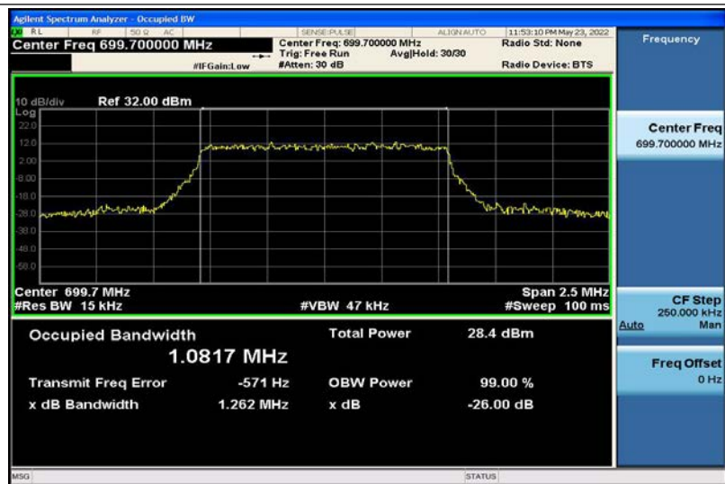
Band12-1.4MHz-16QAM-23017-6RB#0-1.0817
