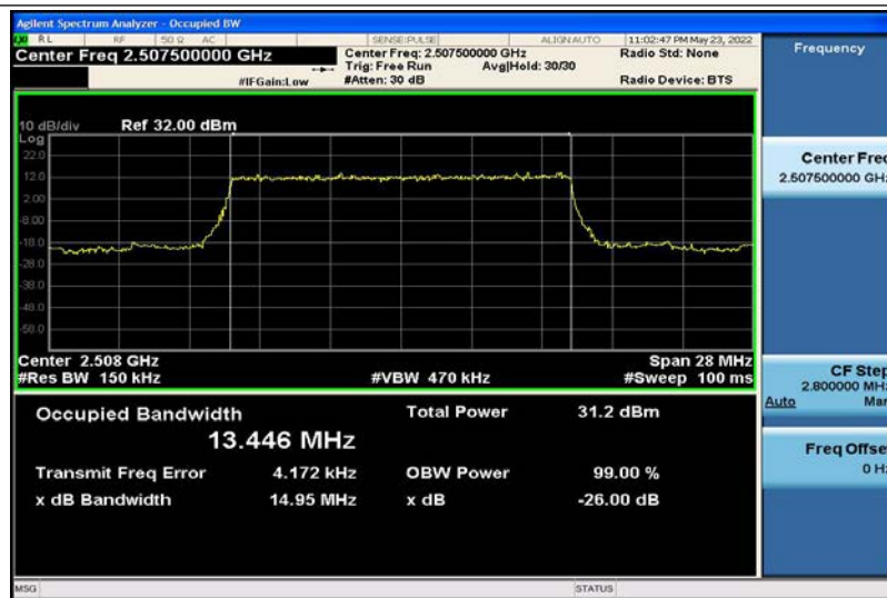
Band7-15MHz-QPSK-20825-75RB#0-13.446
