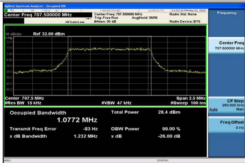
Band12-1.4MHz-16QAM-23095-6RB#0-1.0772
