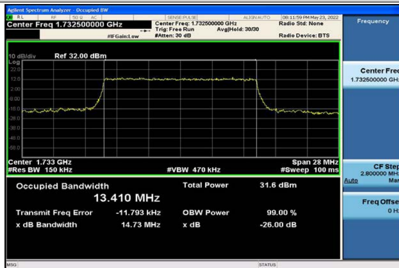
Band4-15MHz-QPSK-20175-75RB#0-13.410
