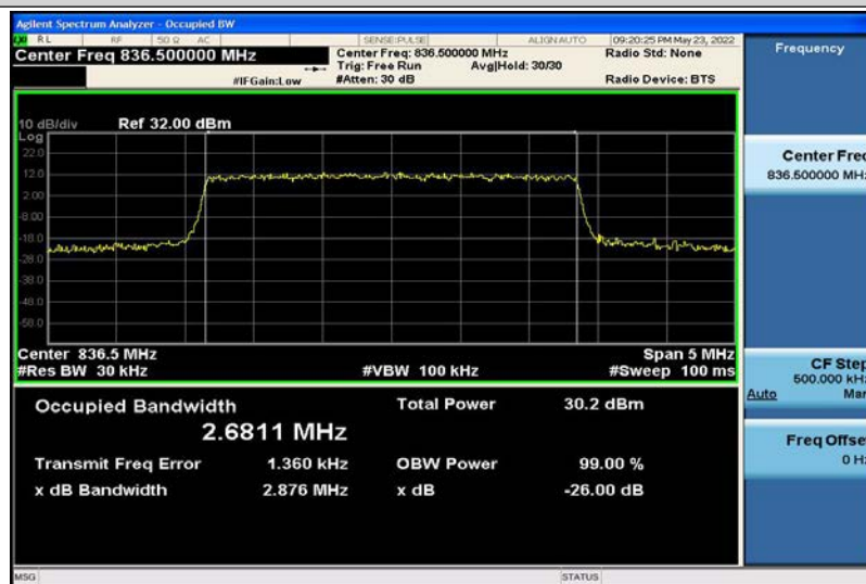
Band5-3MHz-QPSK-20525-15RB#0-2.6811
