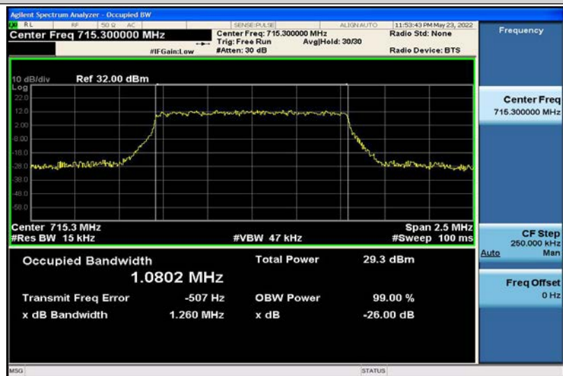
Band12-1.4MHz-QPSK-23173-6RB#0-1.0802
