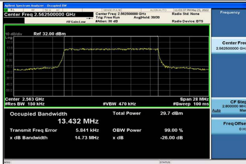
Band7-15MHz-16QAM-21375-75RB#0-13.432
