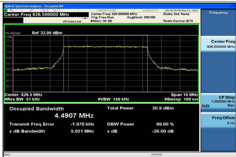
Band5-5MHz-QPSK-20425-25RB#0-4.4907
