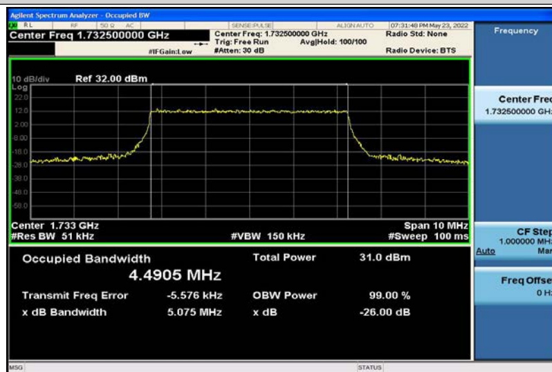
Band4-5MHz-QPSK-20175-25RB#0-4.4905
