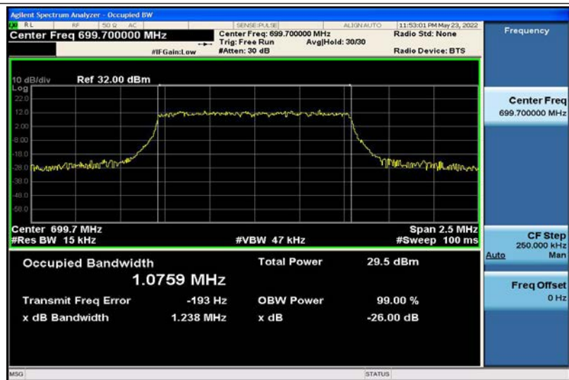
Band12-1.4MHz-QPSK-23017-6RB#0-1.0759
