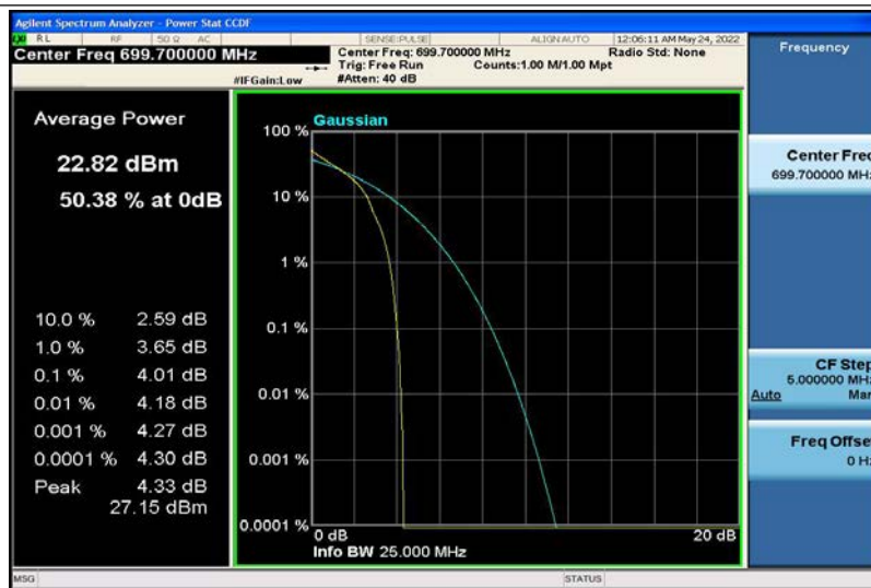
Band12-1.4MHz-QPSK-23017-1RB#0
