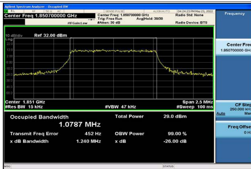
Band2-1.4MHz-16QAM-18607-6RB#0-1.0787
