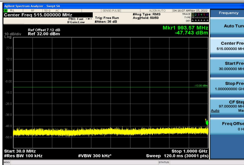
Band66-15MHz-QPSK-132597-1RB#0-30~1000MHz
