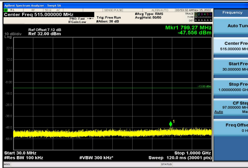
Band66-10MHz-QPSK-132622-1RB#0-30~1000MHz
