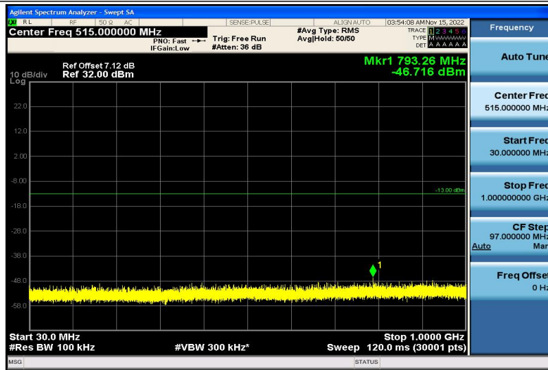
Band66-10MHz-16QAM-132622-1RB#0-30~1000MHz
