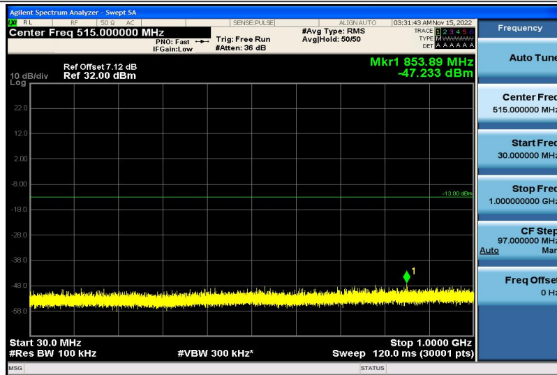
Band66-5MHz-QPSK-132322-1RB#0-30~1000MHz
