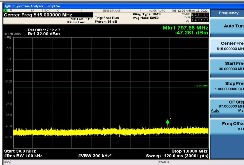
Band66-3MHz-QPSK-132657-1RB#0-30~1000MHz
