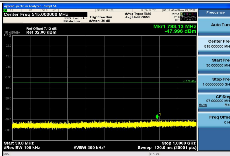
Band66-3MHz-16QAM-132322-1RB#0-30~1000MHz
