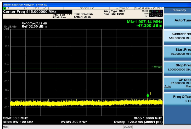
Band66-1.4MHz-QPSK-132665-1RB#0-30~1000MHz
