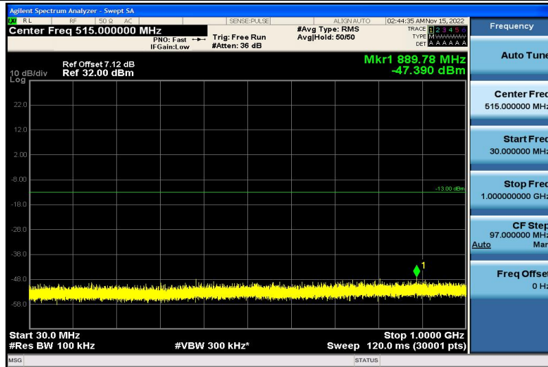
Band66-1.4MHz-16QAM-132322-1RB#0-30~1000MHz
