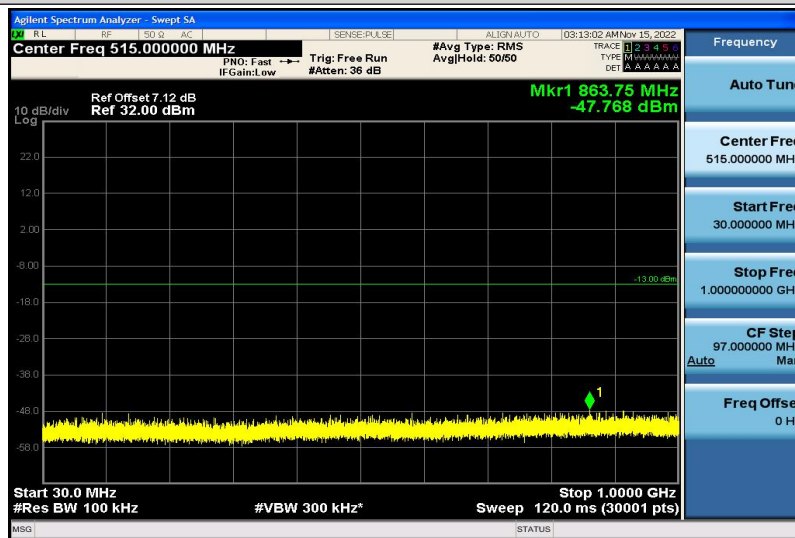
Band66-3MHz-16QAM-132657-1RB#0-30~1000MHz
