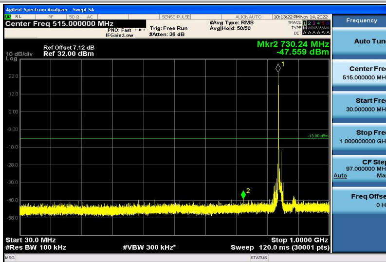
Band5-10MHz-16QAM-20600-1RB#0-30~1000MHz
