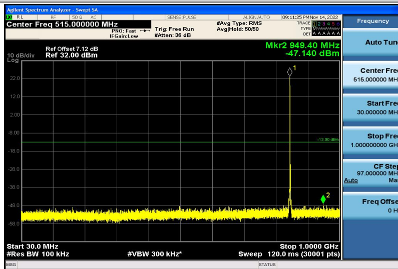
Band5-1.4MHz-QPSK-20643-1RB#0-30~1000MHz
