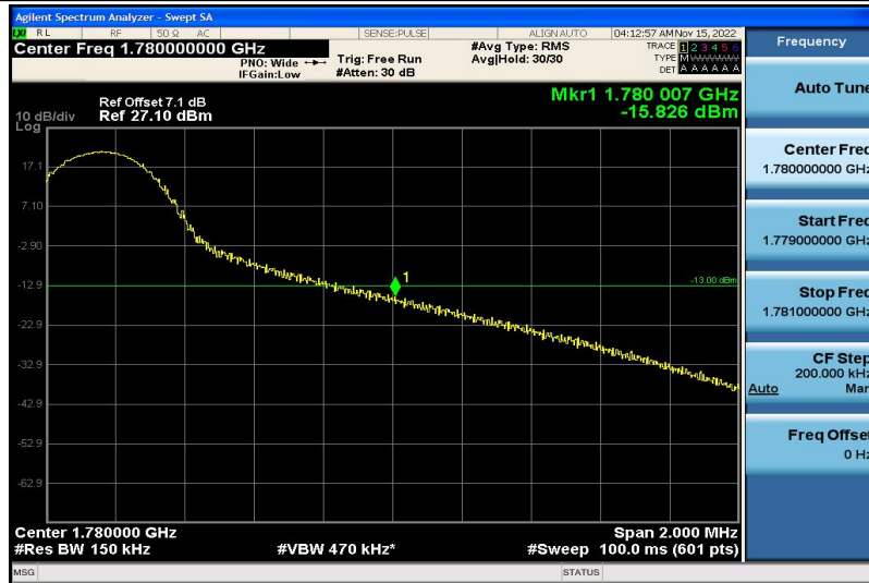
Band66-15MHz-QPSK-132597-1RB#74
