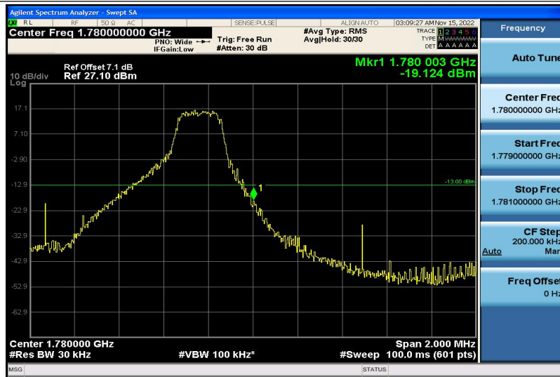
Band66-3MHz-16QAM-132657-1RB#14
