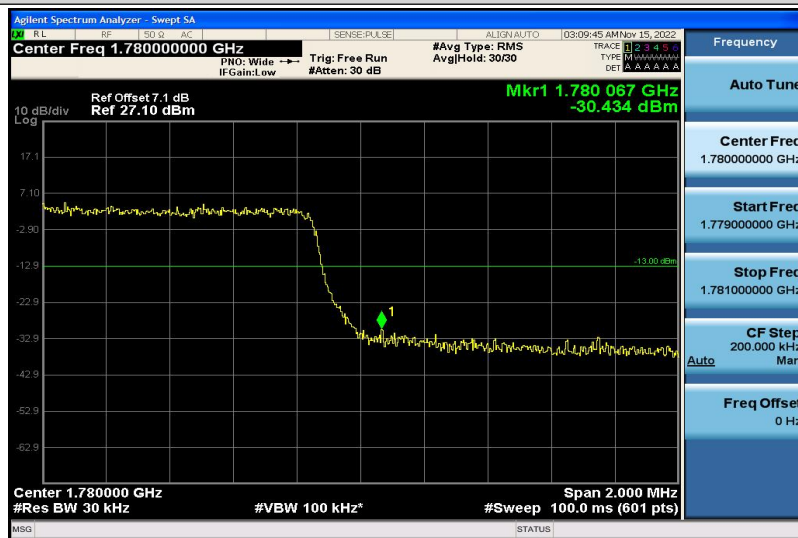
Band66-3MHz-16QAM-132657-15RB#0
