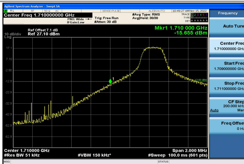
Band66-5MHz-QPSK-131997-1RB#0
