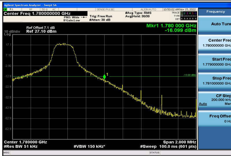
Band66-5MHz-QPSK-132647-1RB#24
