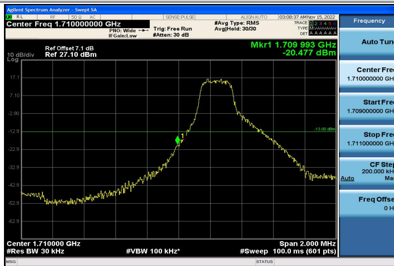
Band66-3MHz-16QAM-131987-1RB#0
