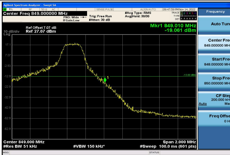
Band5-5MHz-16QAM-20625-1RB#24
