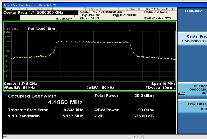
Band66-5MHz-QPSK-132322-25RB#0-4.4860
