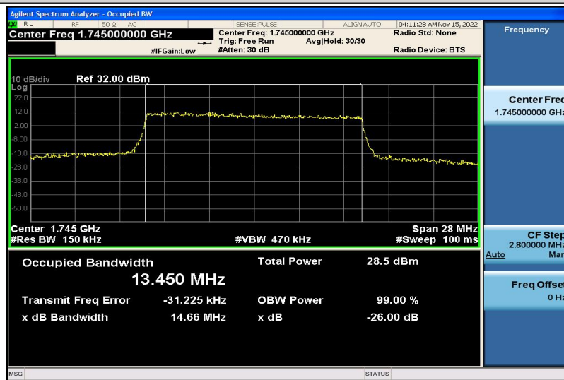
Band66-15MHz-16QAM-132322-75RB#0-13.450
