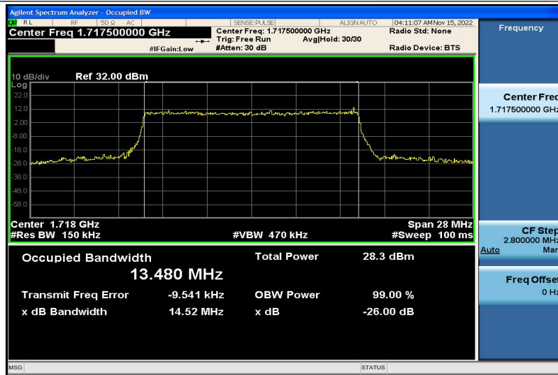
Band66-15MHz-16QAM-132047-75RB#0-13.480
