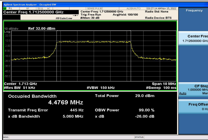
Band66-5MHz-QPSK-131997-25RB#0-4.4769
