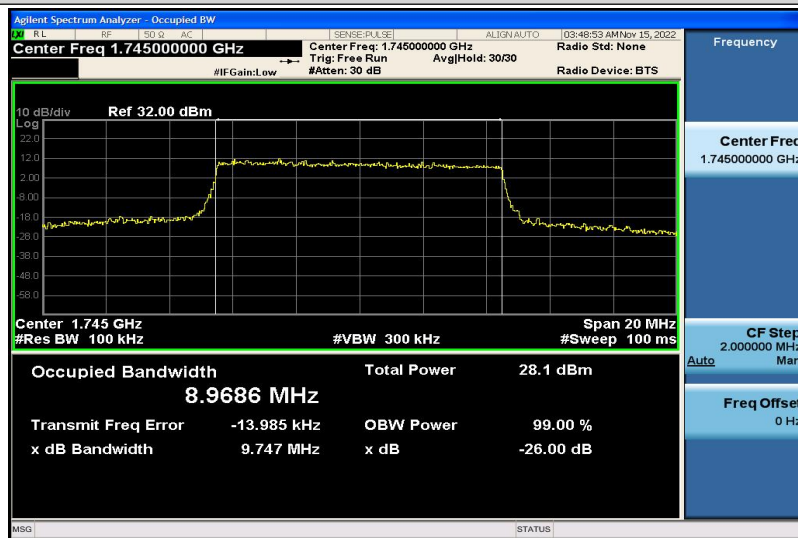
Band66-10MHz-16QAM-132322-50RB#0-8.9686
