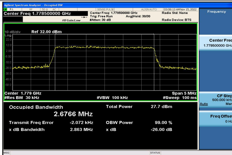
Band66-3MHz-16QAM-132657-15RB#0-2.6766
