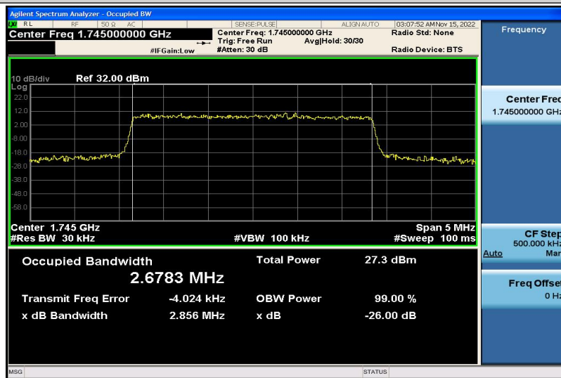
Band66-3MHz-16QAM-132322-15RB#0-2.6783
