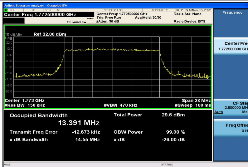
Band66-15MHz-QPSK-132597-75RB#0-13.391
