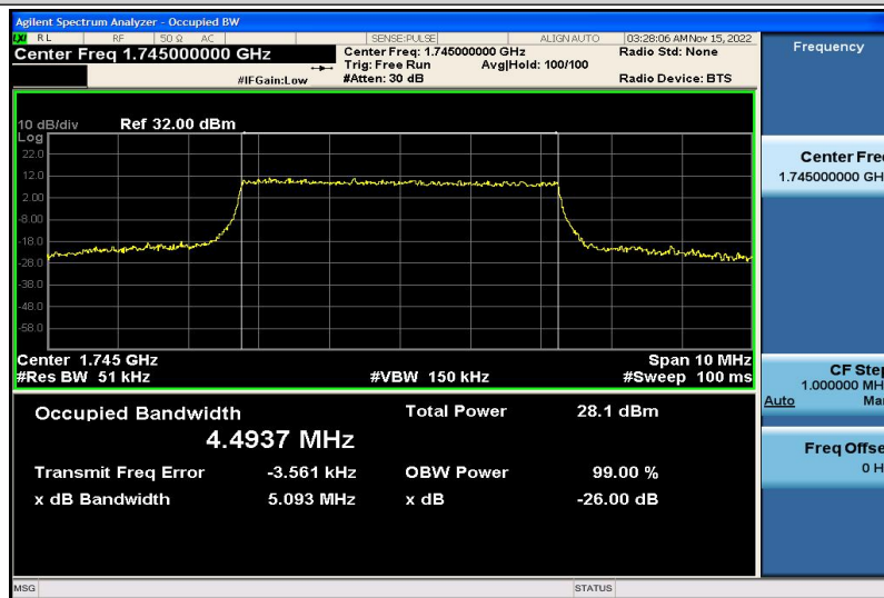
Band66-5MHz-16QAM-132322-25RB#0-4.4937
