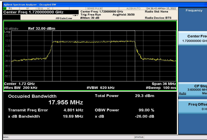
Band66-20MHz-QPSK-132072-100RB#0-17.955
