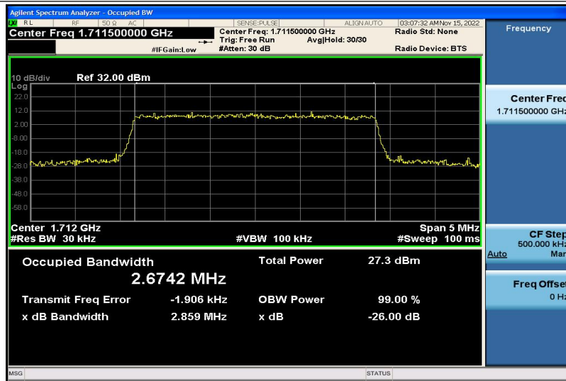
Band66-3MHz-16QAM-131987-15RB#0-2.6742
