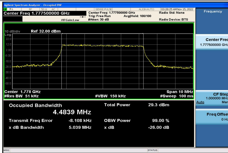
Band66-5MHz-QPSK-132647-25RB#0-4.4839
