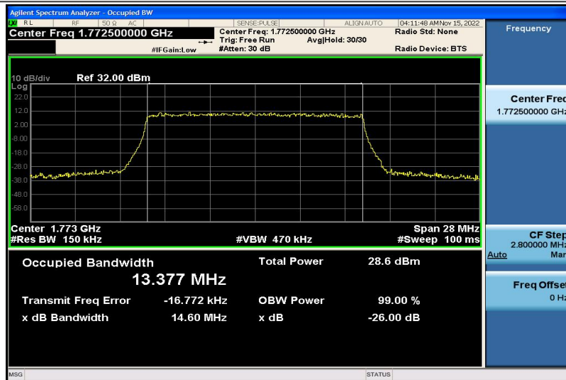
Band66-15MHz-16QAM-132597-75RB#0-13.377
