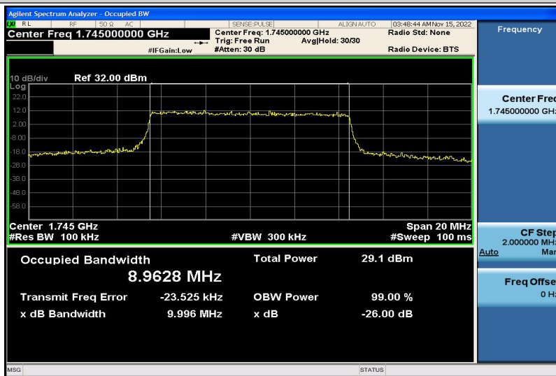
Band66-10MHz-QPSK-132322-50RB#0-8.9628
