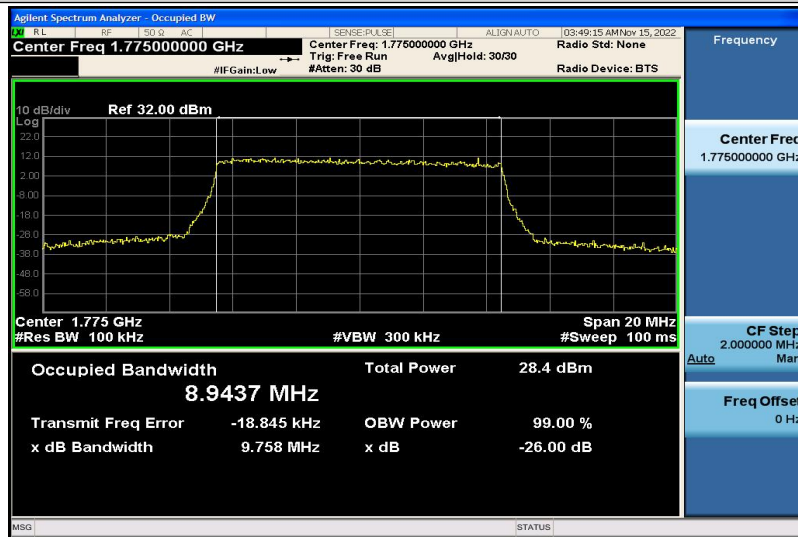
Band66-10MHz-16QAM-132622-50RB#0-8.9437
