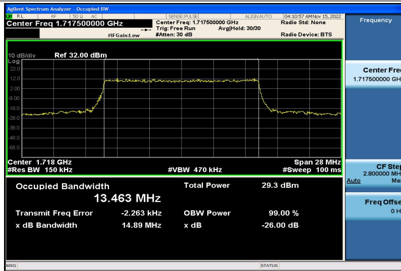
Band66-15MHz-QPSK-132047-75RB#0-13.463
