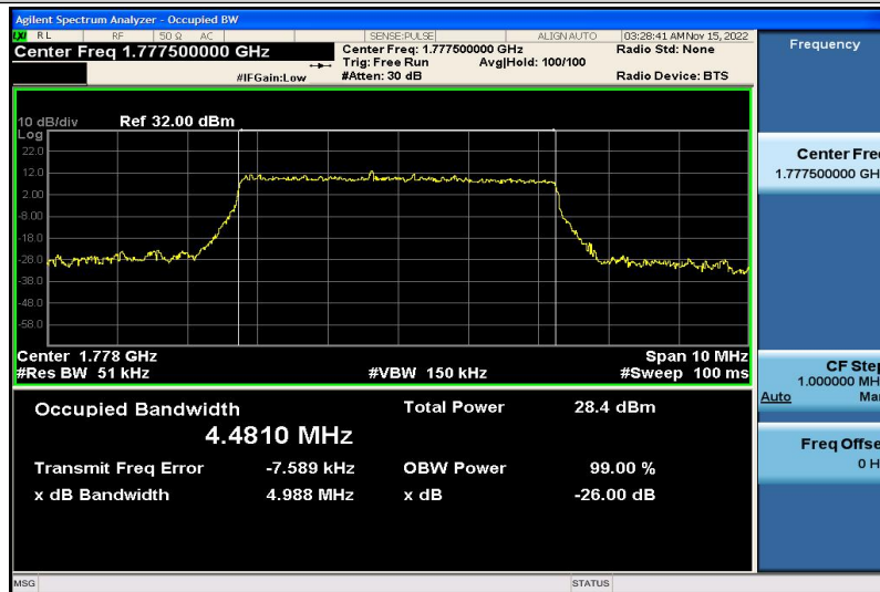
Band66-5MHz-16QAM-132647-25RB#0-4.4810
