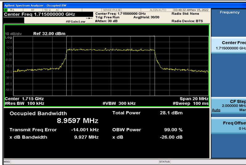
Band66-10MHz-16QAM-132022-50RB#0-8.9597
