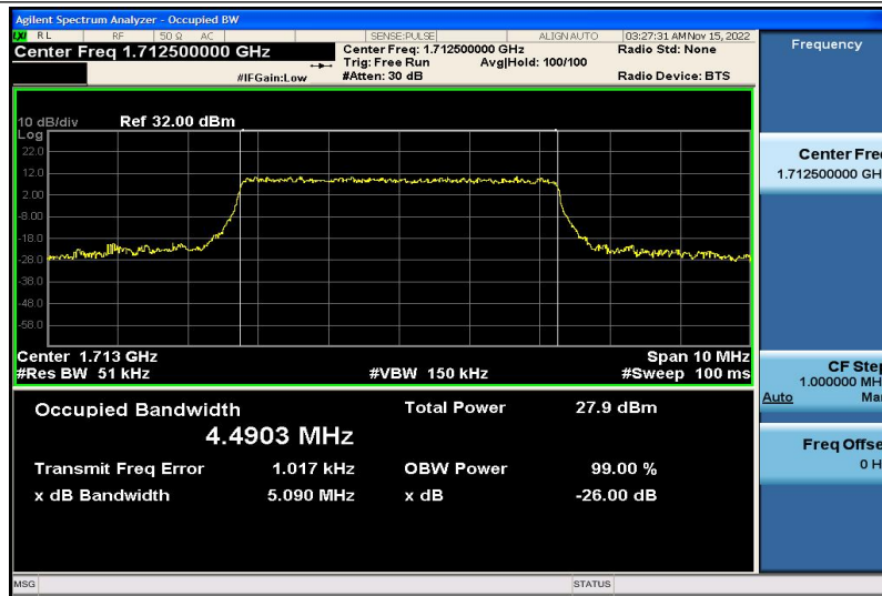
Band66-5MHz-16QAM-131997-25RB#0-4.4903
