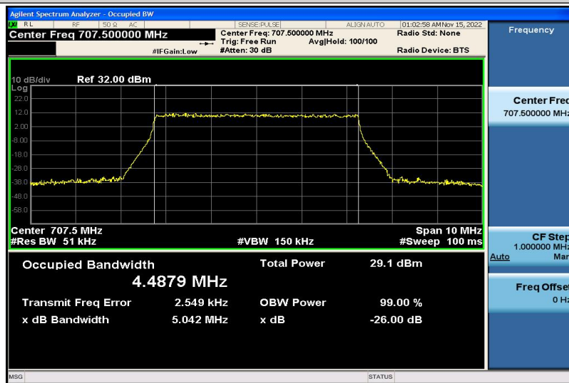
Band12-5MHz-16QAM-23095-25RB#0-4.4879
