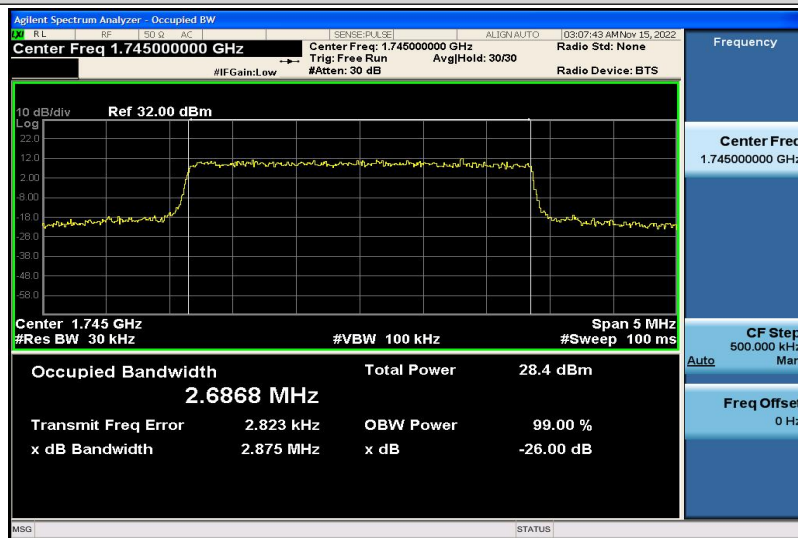
Band66-3MHz-QPSK-132322-15RB#0-2.6868
