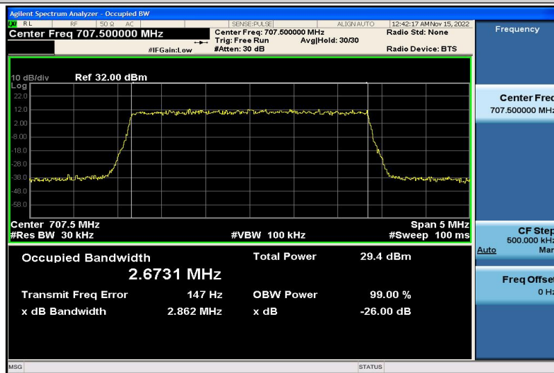
Band12-3MHz-QPSK-23095-15RB#0-2.6731
