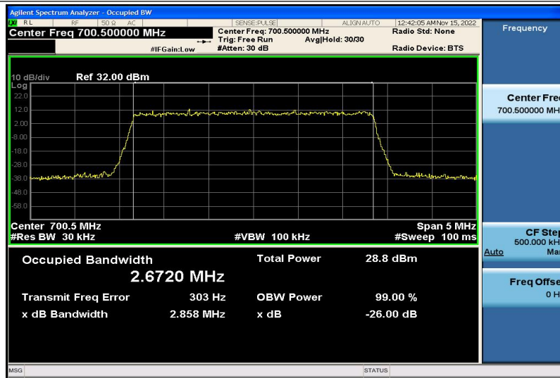
Band12-3MHz-16QAM-23025-15RB#0-2.6720
