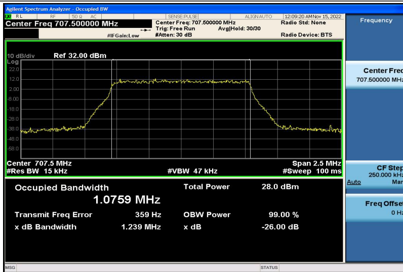
Band12-1.4MHz-16QAM-23095-6RB#0-1.0759
