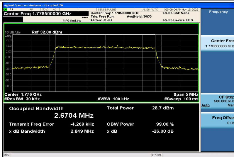
Band66-3MHz-QPSK-132657-15RB#0-2.6704
