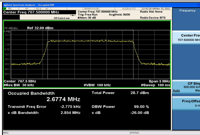
Band12-3MHz-16QAM-23095-15RB#0-2.6774
