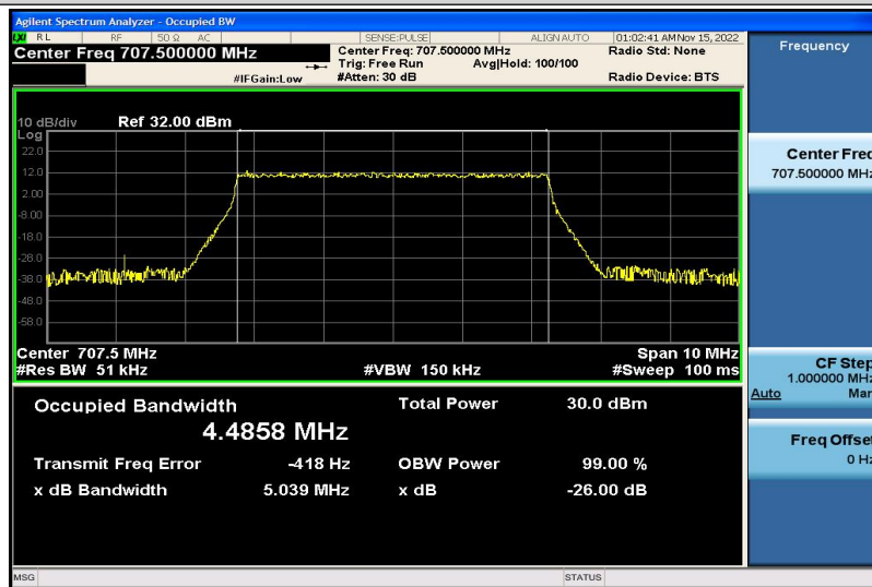
Band12-5MHz-QPSK-23095-25RB#0-4.4858
