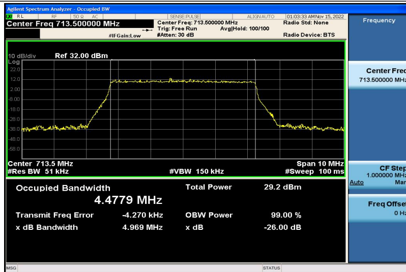
Band12-5MHz-16QAM-23155-25RB#0-4.4779
