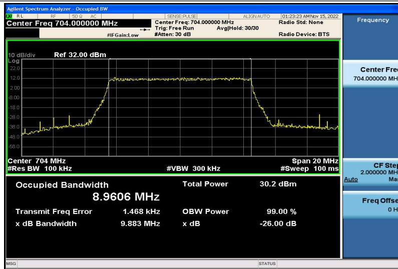
Band12-10MHz-QPSK-23060-50RB#0-8.9606
