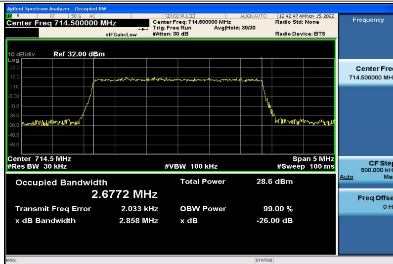
Band12-3MHz-16QAM-23165-15RB#0-2.6772
