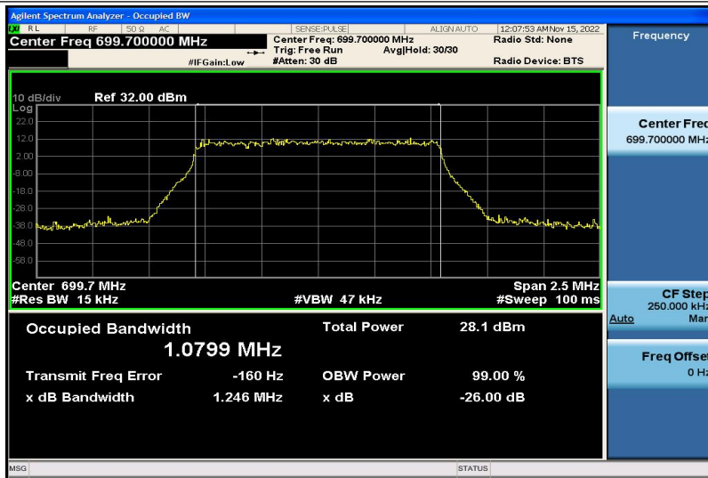
Band12-1.4MHz-16QAM-23017-6RB#0-1.0799
