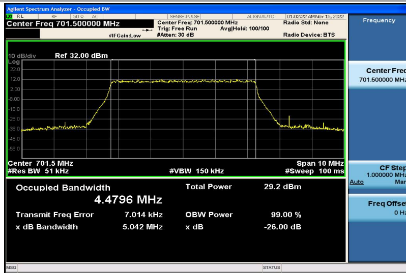
Band12-5MHz-16QAM-23035-25RB#0-4.4796
