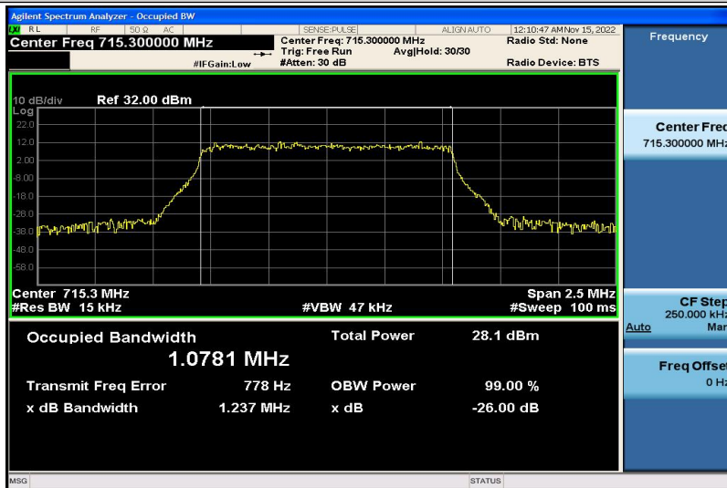
Band12-1.4MHz-16QAM-23173-6RB#0-1.0781
