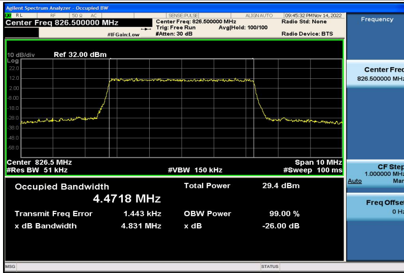
Band5-5MHz-16QAM-20425-25RB#0-4.4718
