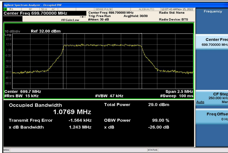
Band12-1.4MHz-QPSK-23017-6RB#0-1.0769
