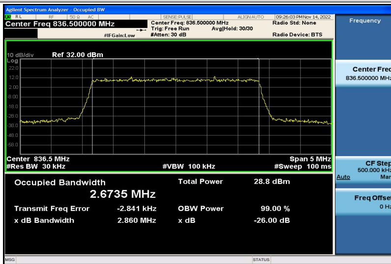
Band5-3MHz-16QAM-20525-15RB#0-2.6735
