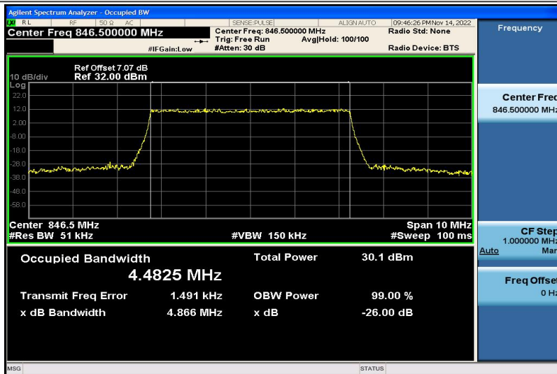
Band5-5MHz-QPSK-20625-25RB#0-4.4825
