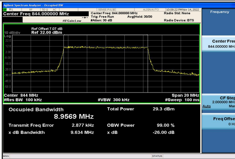
Band5-10MHz-16QAM-20600-50RB#0-8.9569
