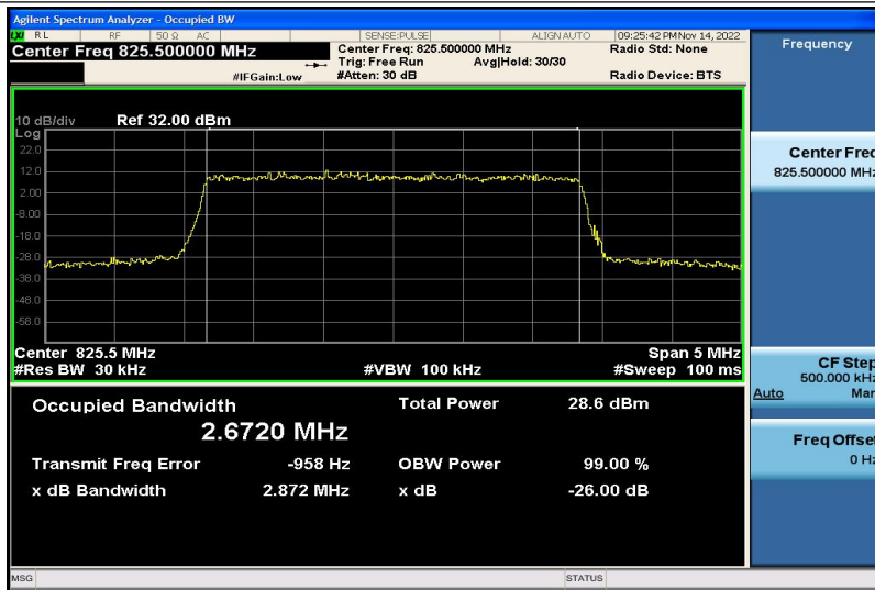
Band5-3MHz-16QAM-20415-15RB#0-2.6720
