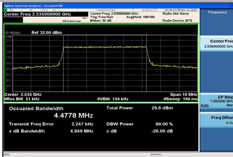
Band7-5MHz-QPSK-21100-25RB#0-4.4778
