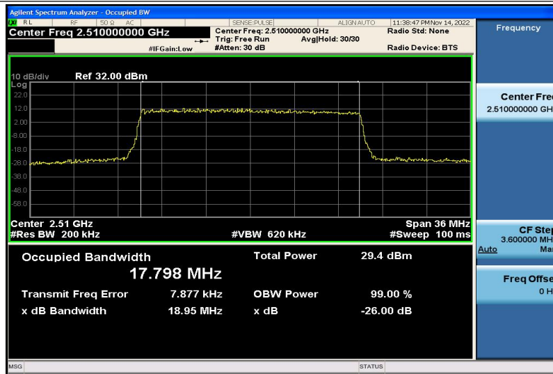
Band7-20MHz-16QAM-20850-100RB#0-17.798
