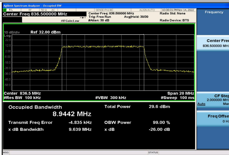
Band5-10MHz-16QAM-20525-50RB#0-8.9442
