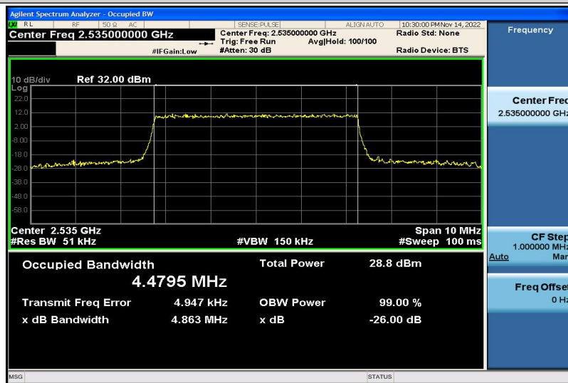
Band7-5MHz-16QAM-21100-25RB#0-4.4795
