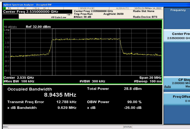
Band7-10MHz-16QAM-21100-50RB#0-8.9435
