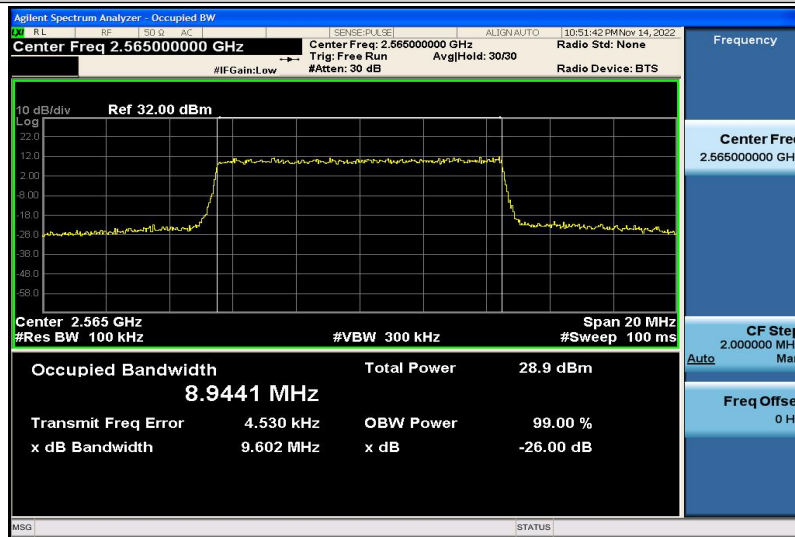
Band7-10MHz-16QAM-21400-50RB#0-8.9441
