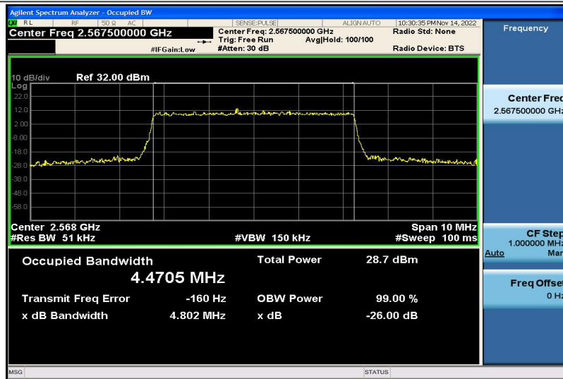
Band7-5MHz-16QAM-21425-25RB#0-4.4705
