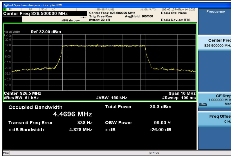
Band5-5MHz-QPSK-20425-25RB#0-4.4696
