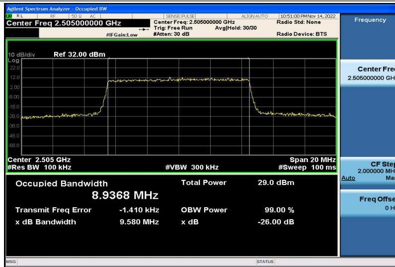
Band7-10MHz-16QAM-20800-50RB#0-8.9368
