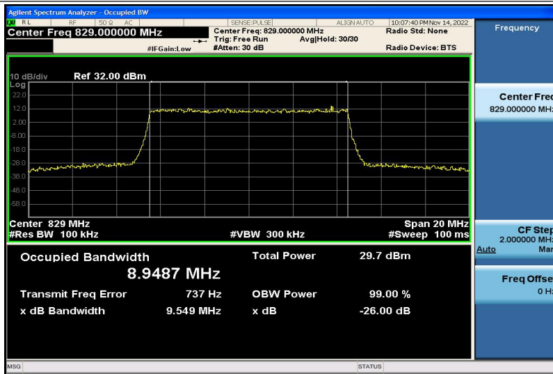
Band5-10MHz-16QAM-20450-50RB#0-8.9487
