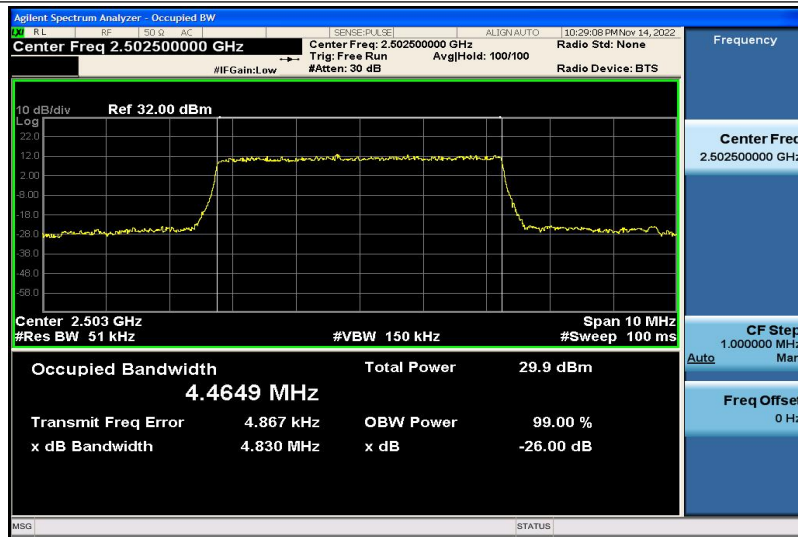
Band7-5MHz-QPSK-20775-25RB#0-4.4649
