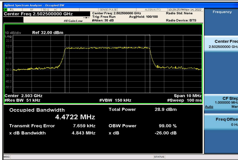
Band7-5MHz-16QAM-20775-25RB#0-4.4722
