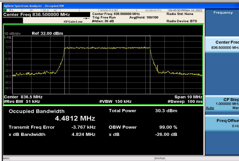
Band5-5MHz-QPSK-20525-25RB#0-4.4812
