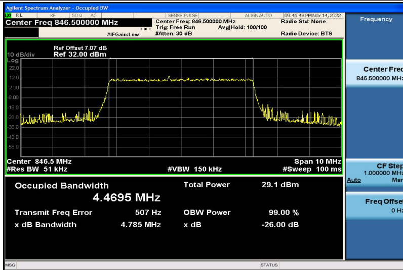
Band5-5MHz-16QAM-20625-25RB#0-4.4695
