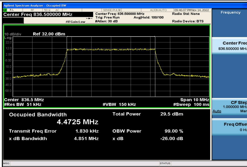
Band5-5MHz-16QAM-20525-25RB#0-4.4725
