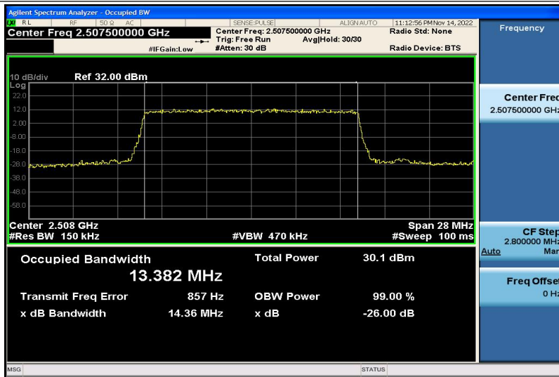
Band7-15MHz-QPSK-20825-75RB#0-13.382
