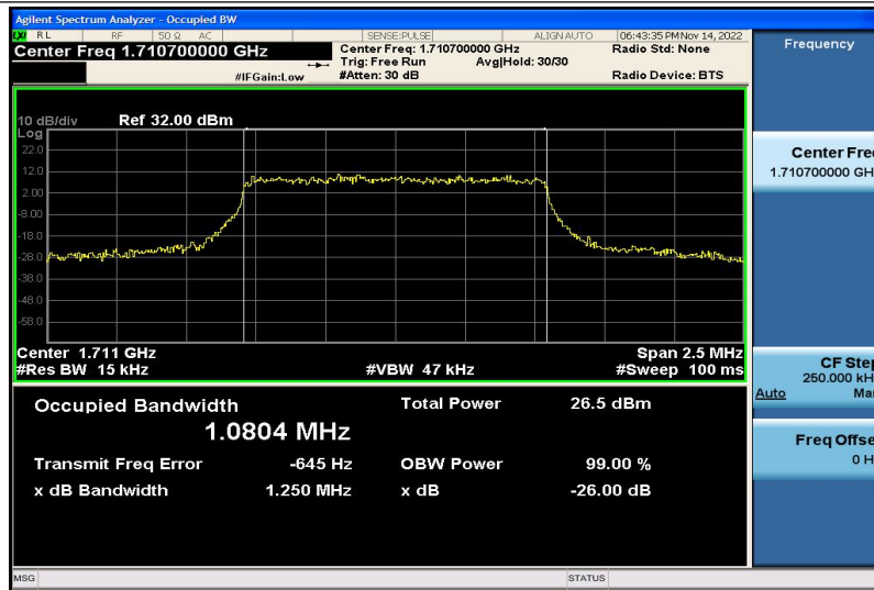
Band4-1.4MHz-16QAM-19957-6RB#0-1.0804
