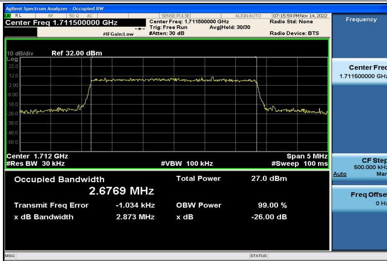
Band4-3MHz-16QAM-19965-15RB#0-2.6769
