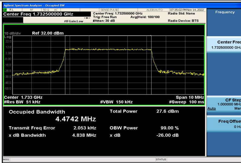
Band4-5MHz-16QAM-20175-25RB#0-4.4742
