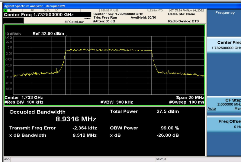
Band4-10MHz-16QAM-20175-50RB#0-8.9316
