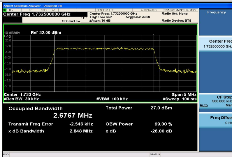
Band4-3MHz-16QAM-20175-15RB#0-2.6767
