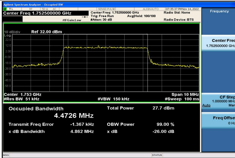
Band4-5MHz-16QAM-20375-25RB#0-4.4726
