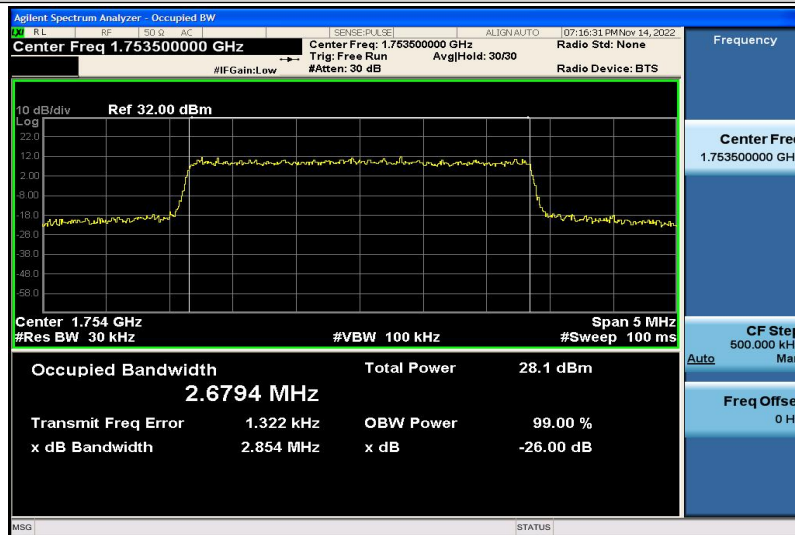
Band4-3MHz-QPSK-20385-15RB#0-2.6794
