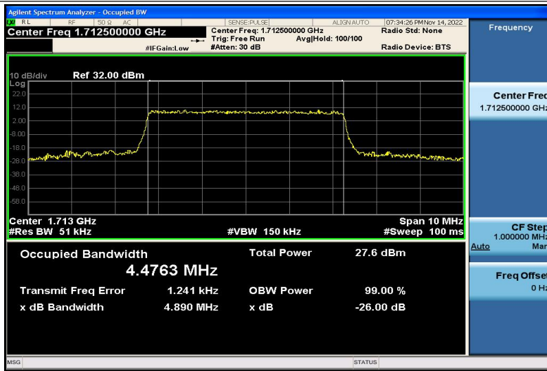
Band4-5MHz-16QAM-19975-25RB#0-4.4763
