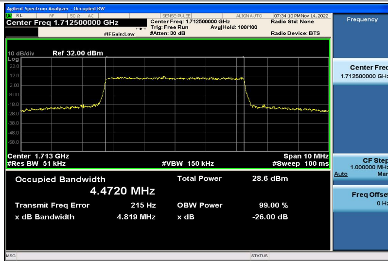
Band4-5MHz-QPSK-19975-25RB#0-4.4720
