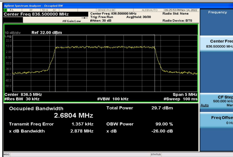
Band5-3MHz-QPSK-20525-15RB#0-2.6804
