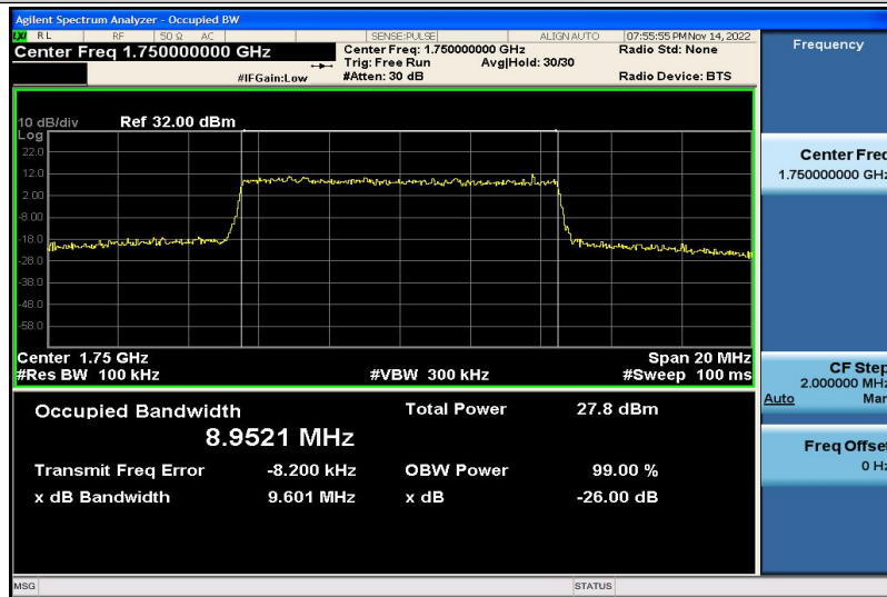
Band4-10MHz-16QAM-20350-50RB#0-8.9521
