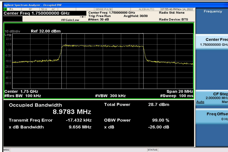
Band4-10MHz-QPSK-20350-50RB#0-8.9783
