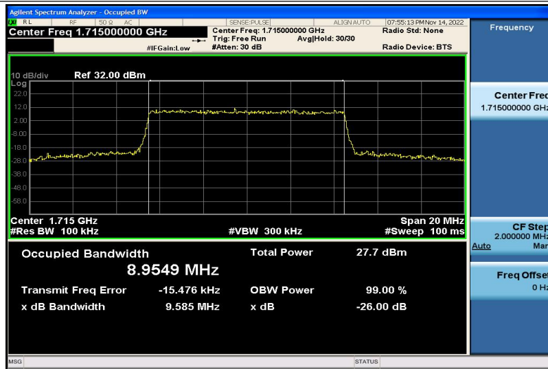
Band4-10MHz-16QAM-20000-50RB#0-8.9549
