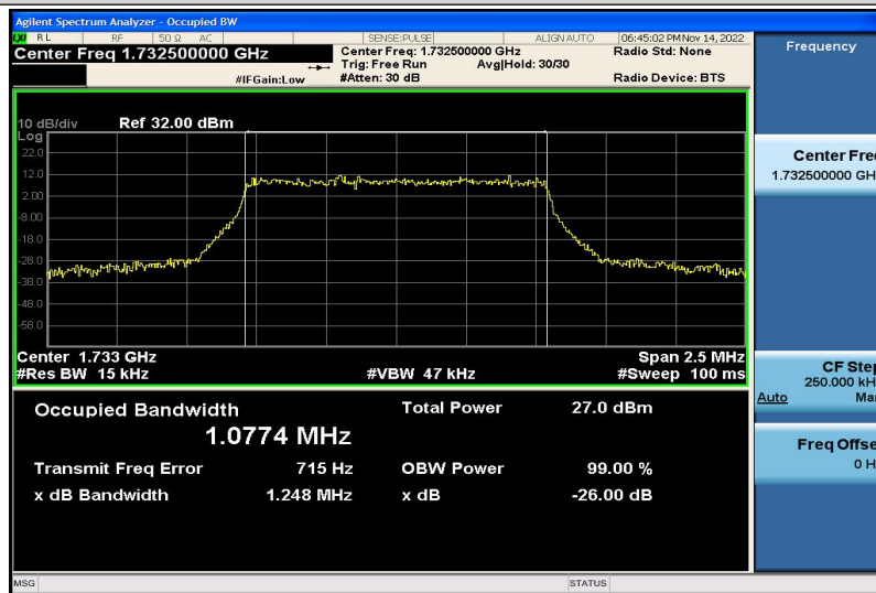
Band4-1.4MHz-16QAM-20175-6RB#0-1.0774
