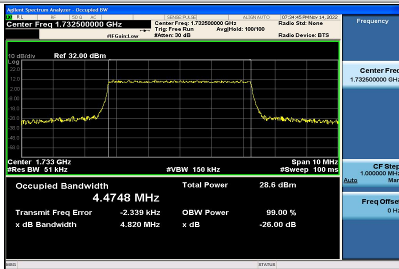
Band4-5MHz-QPSK-1732500000-4.4748
