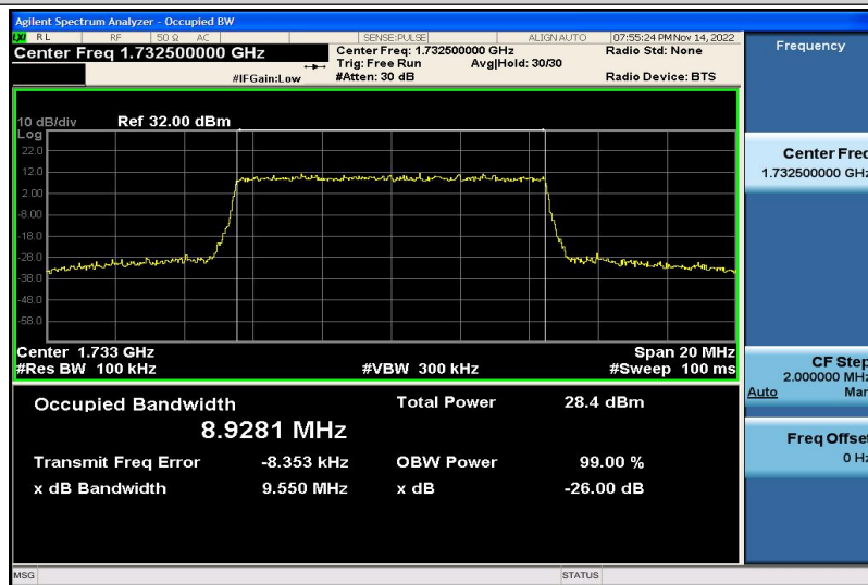
Band4-10MHz-QPSK-20175-50RB#0-8.9281
