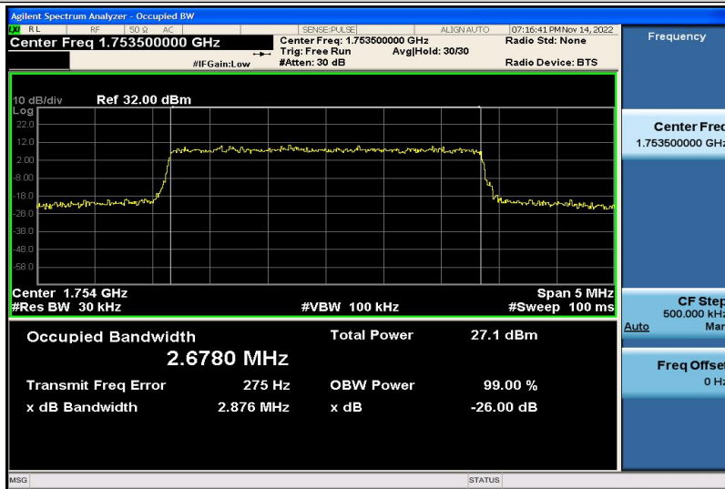
Band4-3MHz-16QAM-20385-15RB#0-2.6780
