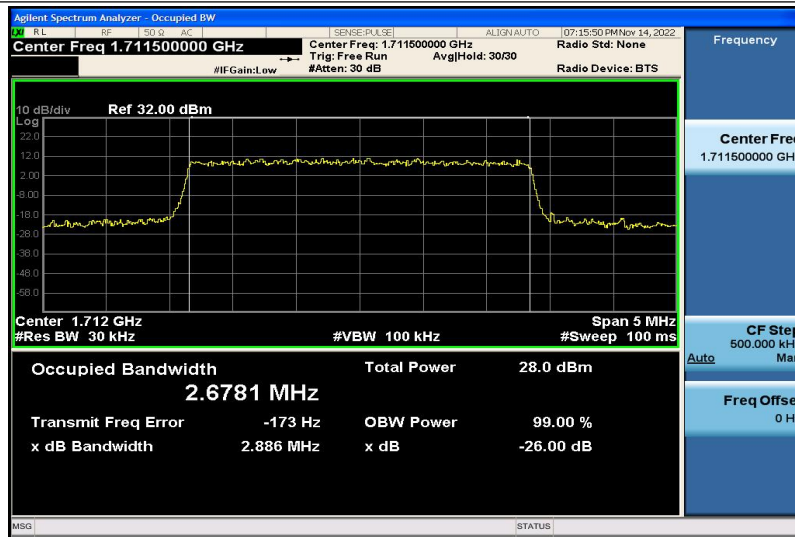
Band4-3MHz-QPSK-19965-15RB#0-2.6781
