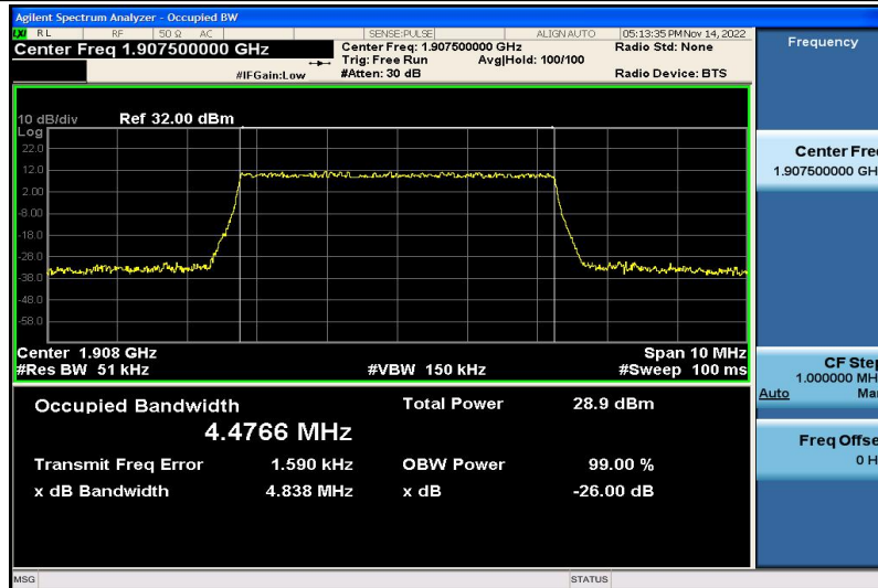
Band2-5MHz-QPSK-19175-25RB#0-4.4766
