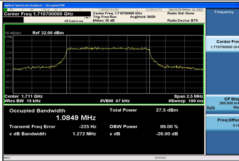
Band4-1.4MHz-QPSK-19957-6RB#0-1.0849
