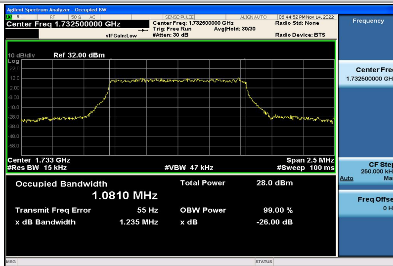
Band4-1.4MHz-QPSK-20175-6RB#0-1.0810
