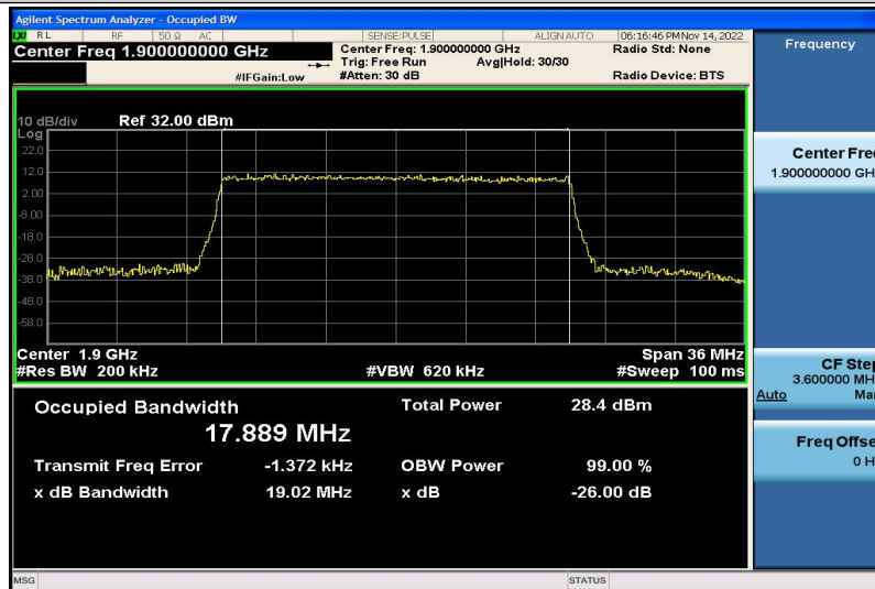
Band2-20MHz-16QAM-19100-100RB#0-17.889
