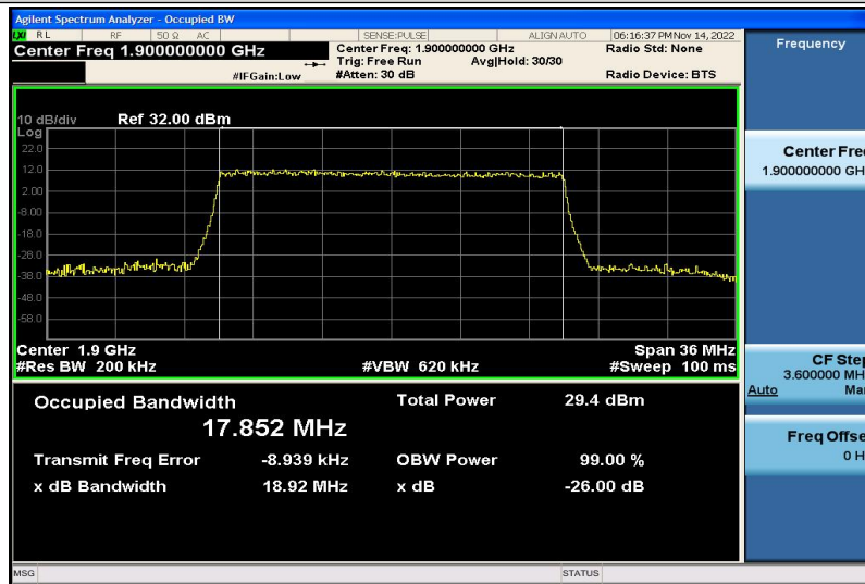
Band2-20MHz-QPSK-19100-100RB#0-17.852
