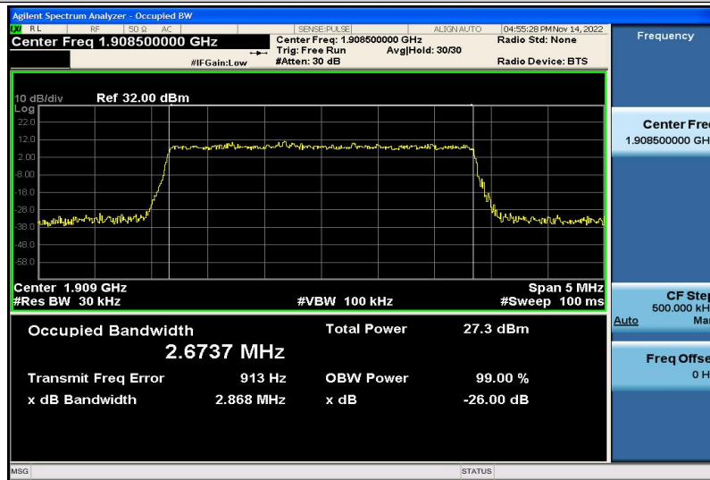
Band2-3MHz-16QAM-19185-15RB#0-2.6737
