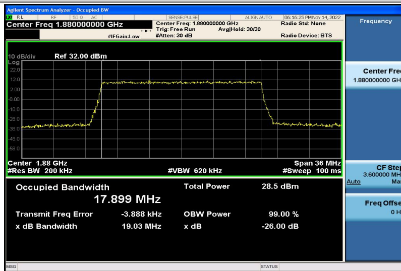
Band2-20MHz-16QAM-18900-100RB#0-17.899
