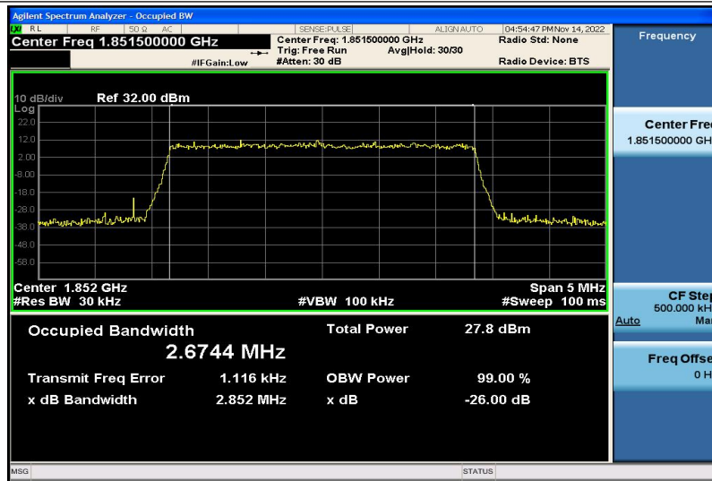
Band2-3MHz-16QAM-18615-15RB#0-2.6744
