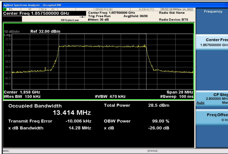
Band2-15MHz-16QAM-18675-75RB#0-13.414
