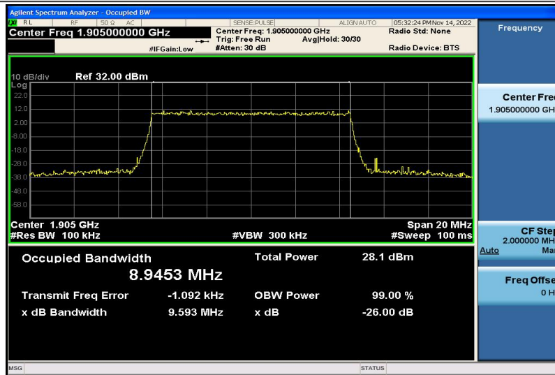
Band2-10MHz-16QAM-19150-50RB#0-8.9453
