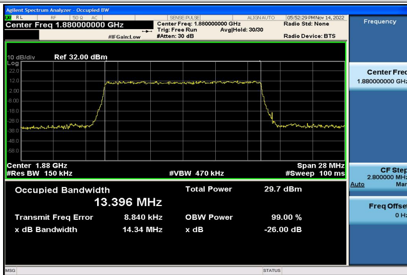
Band2-15MHz-QPSK-18900-75RB#0-13.396
