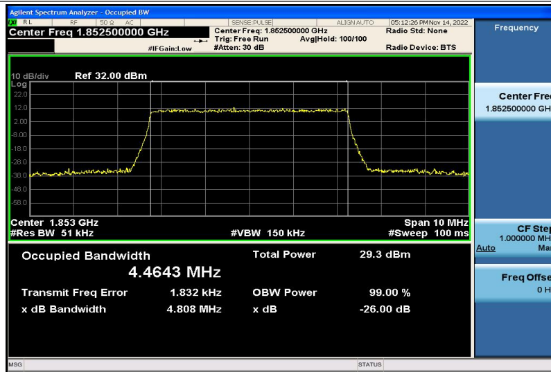
Band2-5MHz-QPSK-18625-25RB#0-4.4643
