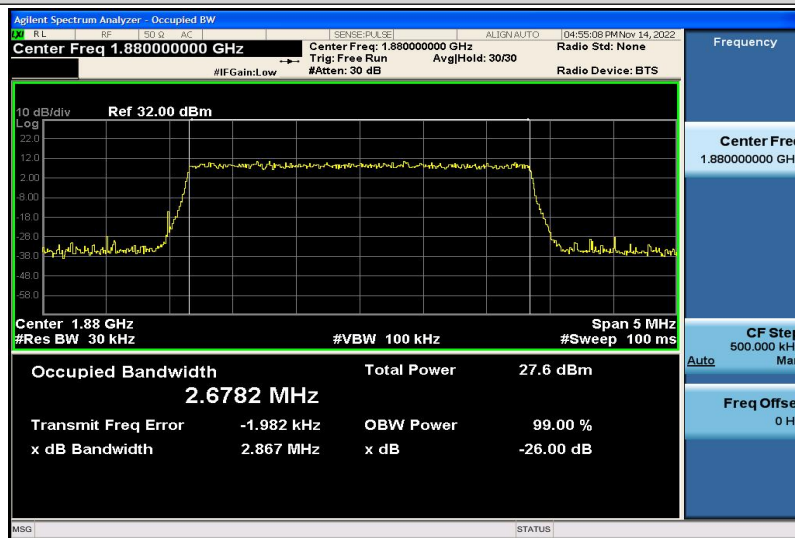
Band2-3MHz-16QAM-18900-15RB#0-2.6782
