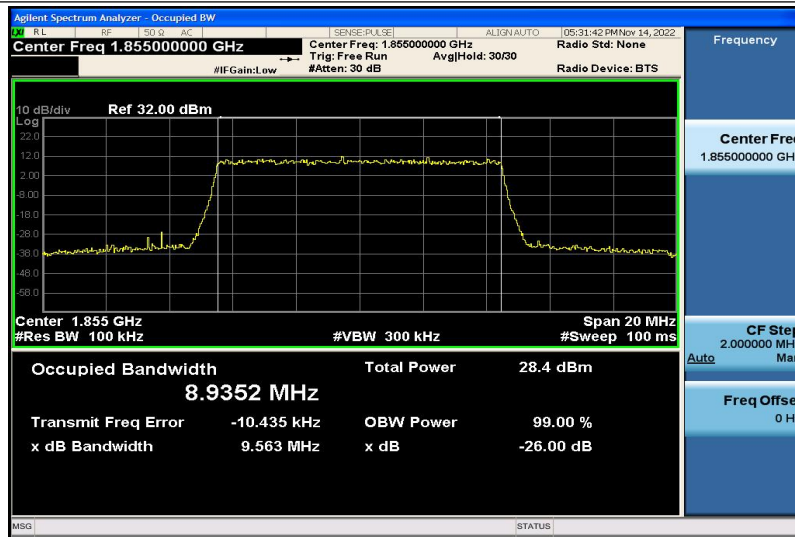
Band2-10MHz-16QAM-18650-50RB#0-8.9352
