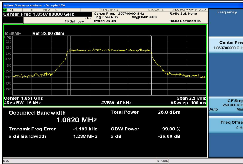
Band2-1.4MHz-16QAM-18607-6RB#0-1.0820
