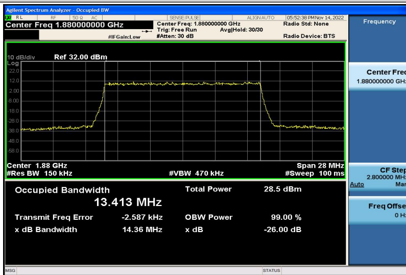
Band2-15MHz-16QAM-18900-75RB#0-13.413
