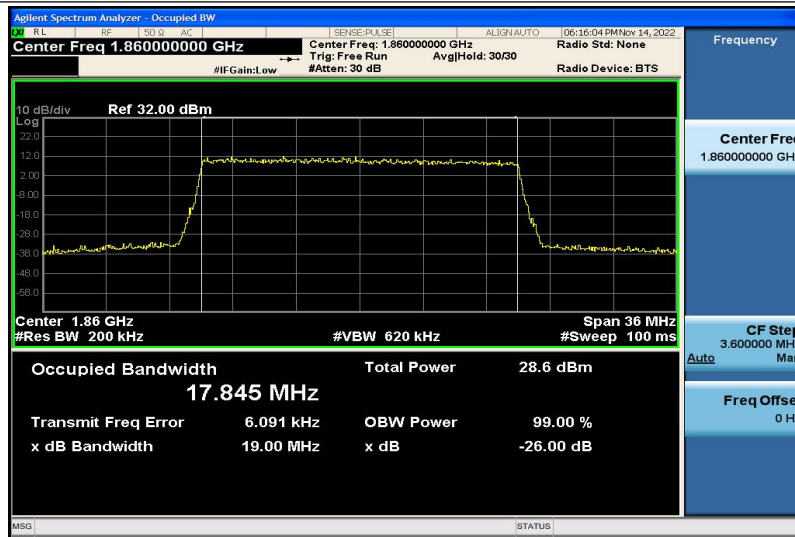
Band2-20MHz-16QAM-18700-100RB#0-17.845
