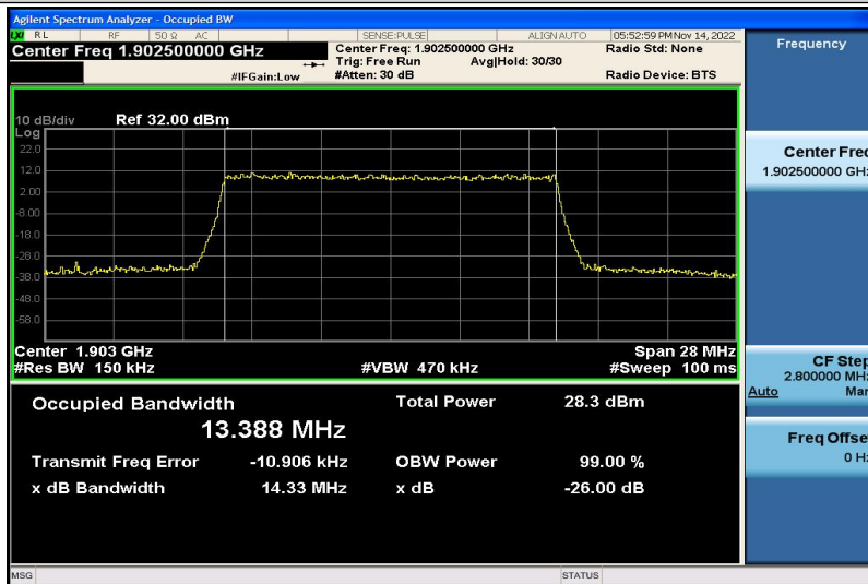
Band2-15MHz-16QAM-19125-75RB#0-13.388
