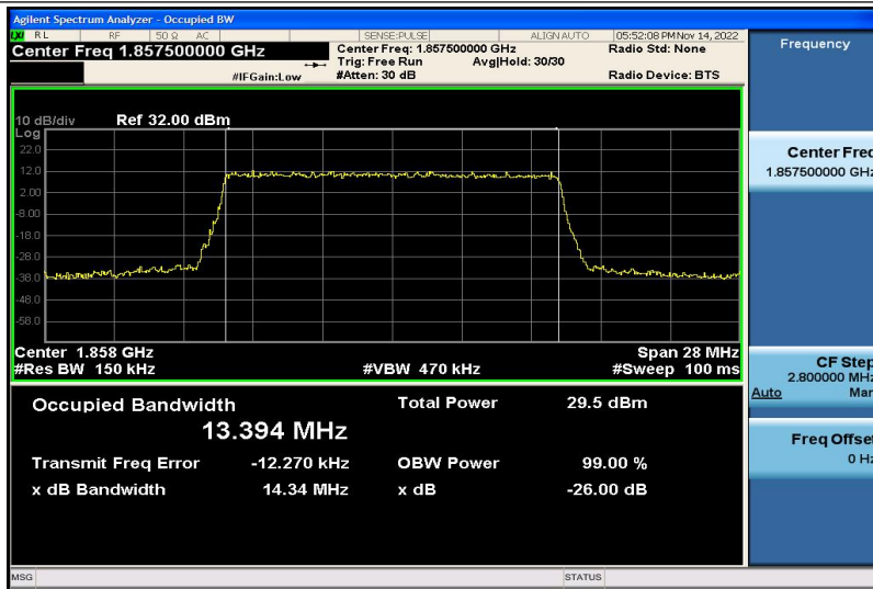
Band2-15MHz-QPSK-18675-75RB#0-13.394
