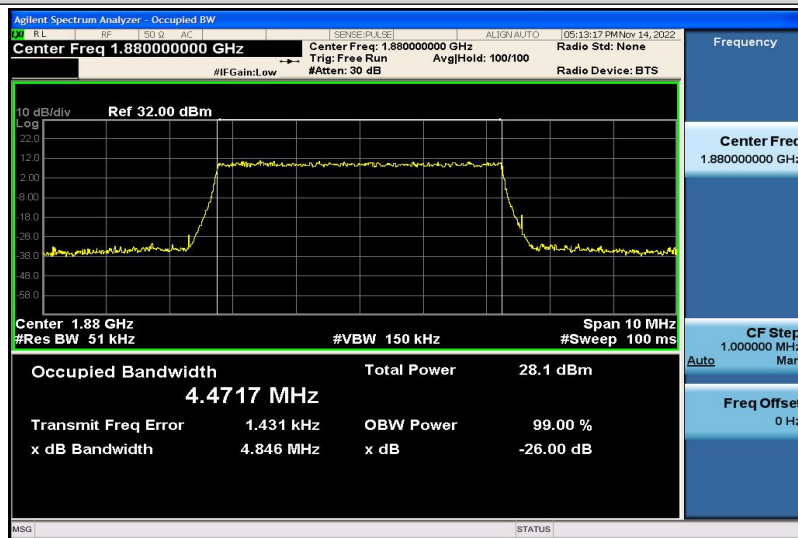
Band2-5MHz-16QAM-18900-25RB#0-4.4717
