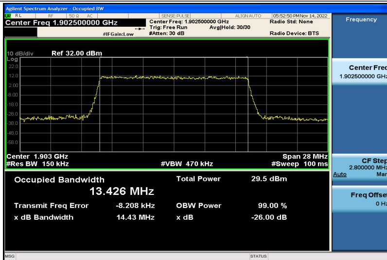
Band2-15MHz-QPSK-19125-75RB#0-13.426
