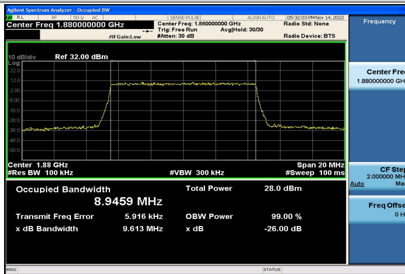
Band2-10MHz-16QAM-18900-50RB#0-8.9459
