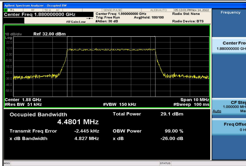
Band2-5MHz-QPSK-18900-25RB#0-4.4801
