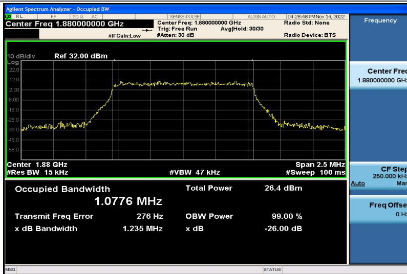
Band2-1.4MHz-16QAM-18900-6RB#0-1.0776
