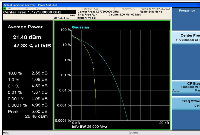
Band66-5MHz-QPSK-132647-1RB#0
