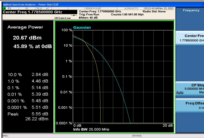
Band66-3MHz-16QAM-132657-1RB#0
