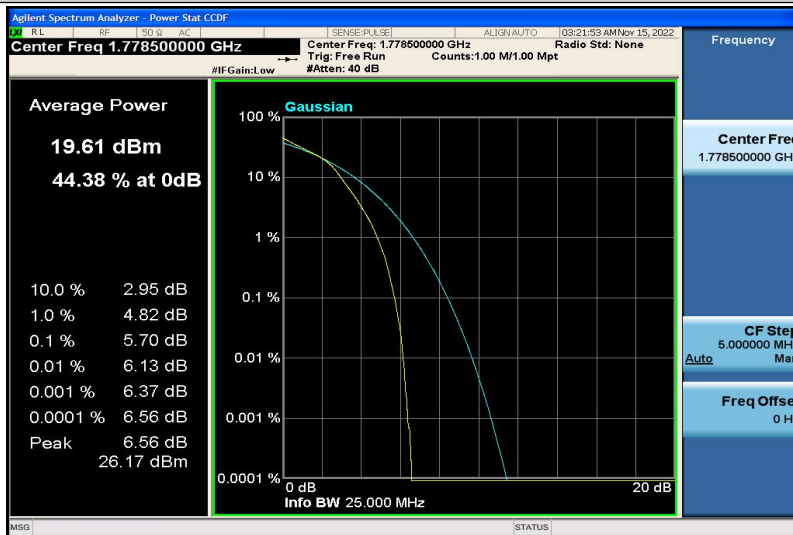
Band66-3MHz-16QAM-132657-15RB#0
