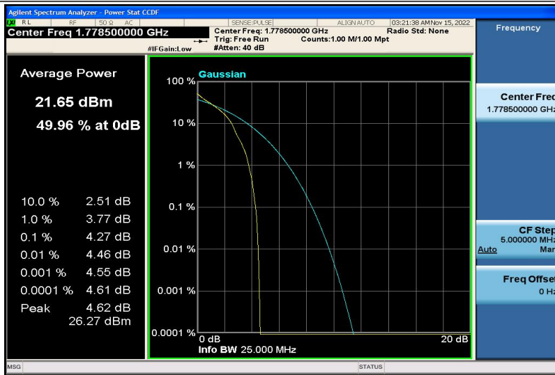
Band66-3MHz-QPSK-132657-1RB#0
