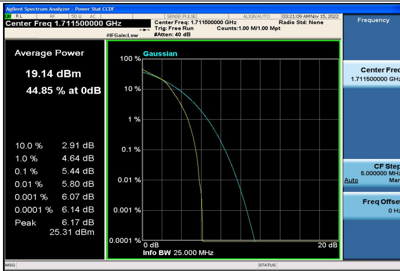
Band66-3MHz-16QAM-131987-15RB#0
