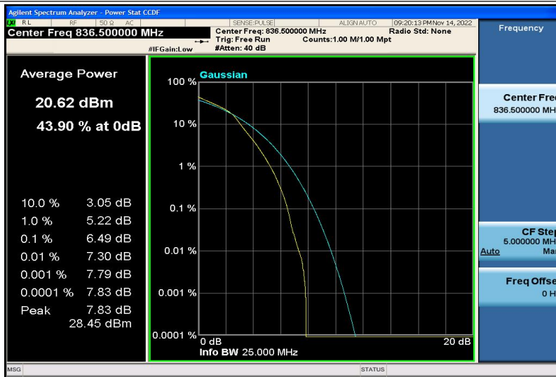
Band5-1.4MHz-16QAM-20525-6RB#0
