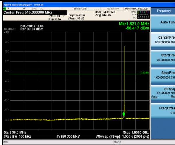
Band5_1.4MHz_QPSK_20407_1RB#0_30~1000_30~1000
