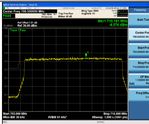
Band17_10MHz_QPSK_23780_50RB#0
