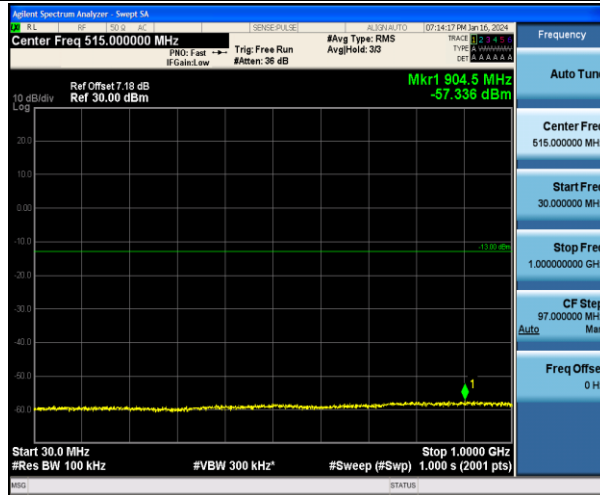
Band2_5MHz_QPSK_19175_1RB#0_30~1000_30~1000
