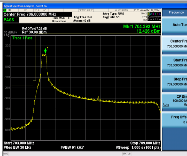
Band17_5MHz_QPSK_23755_1RB#0
