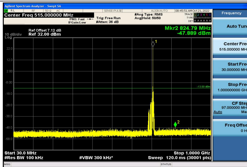
Band12-1.4MHz-16QAM-23173-1RB#0-30~1000MHz
