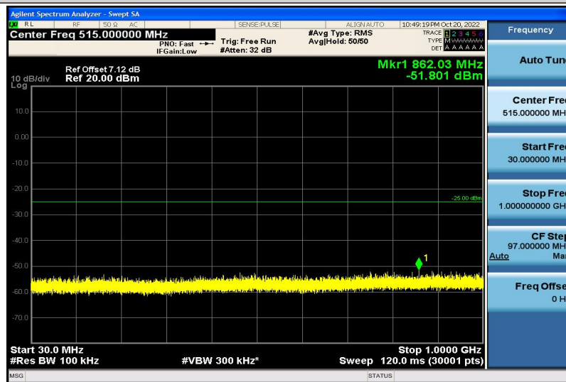
Band7-15MHz-QPSK-21375-1RB#0-30~1000MHz
