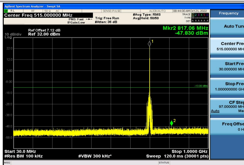
Band12-1.4MHz-16QAM-23095-1RB#0-30~1000MHz
