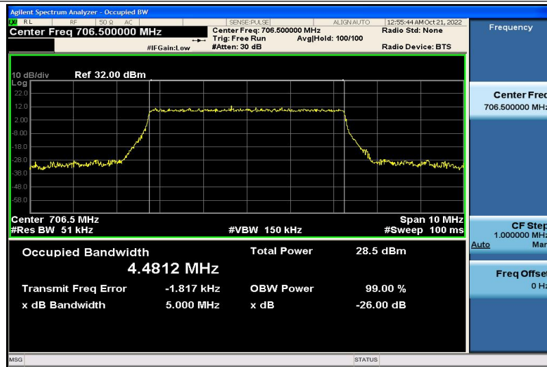
Band17-5MHz-16QAM-23755-25RB#0-4.4812
