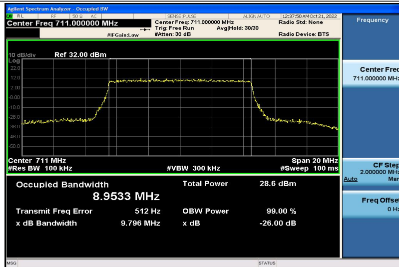
Band12-10MHz-16QAM-23130-50RB#0-8.9533
