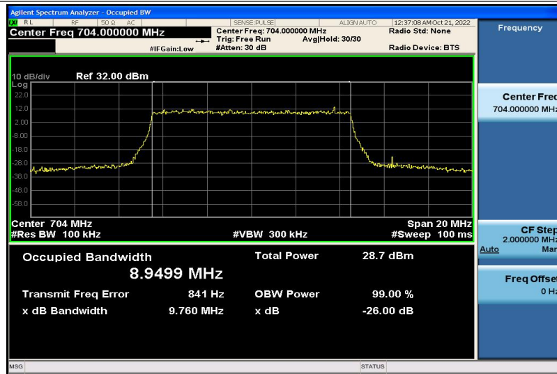
Band12-10MHz-16QAM-23060-50RB#0-8.9499
