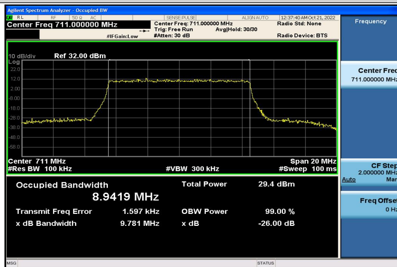
Band12-10MHz-QPSK-23130-50RB#0-8.9419
