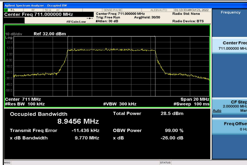
Band17-10MHz-16QAM-23800-50RB#0-8.9456
