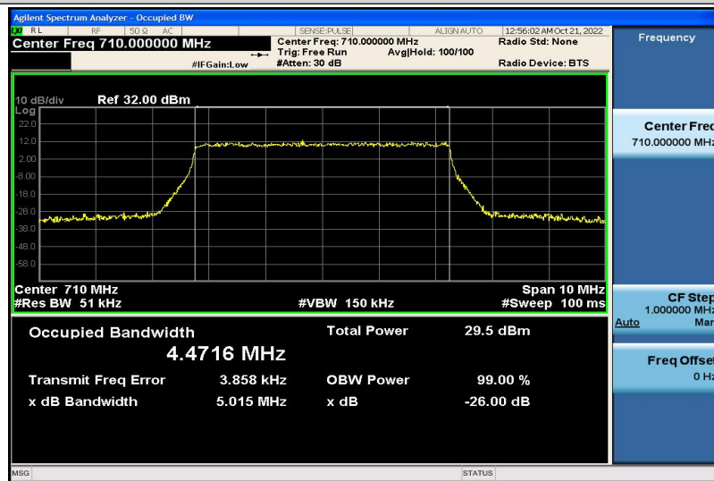
Band17-5MHz-QPSK-23790-25RB#0-4.4716
