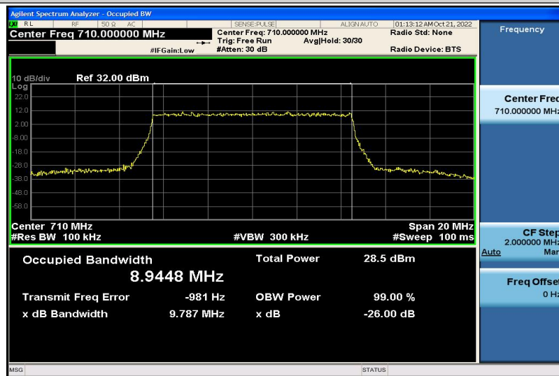
Band17-10MHz-16QAM-23790-50RB#0-8.9448
