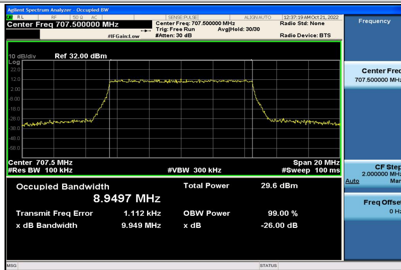
Band12-10MHz-QPSK-23095-50RB#0-8.9497
