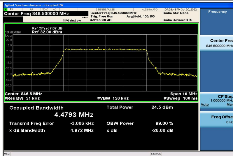
Band5-5MHz-16QAM-20625-25RB#0-4.4793
