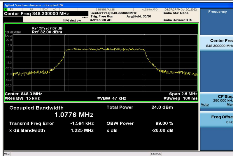
Band5-1.4MHz-QPSK-20643-6RB#0-1.0776
