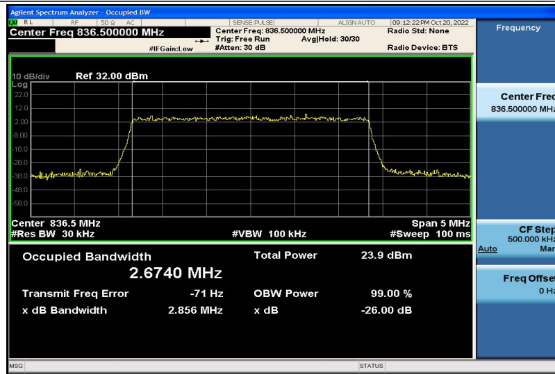
Band5-3MHz-16QAM-20525-15RB#0-2.6740
