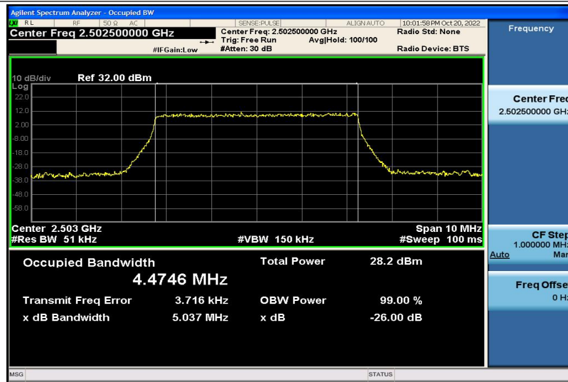
Band7-5MHz-QPSK-20775-25RB#0-4.4746
