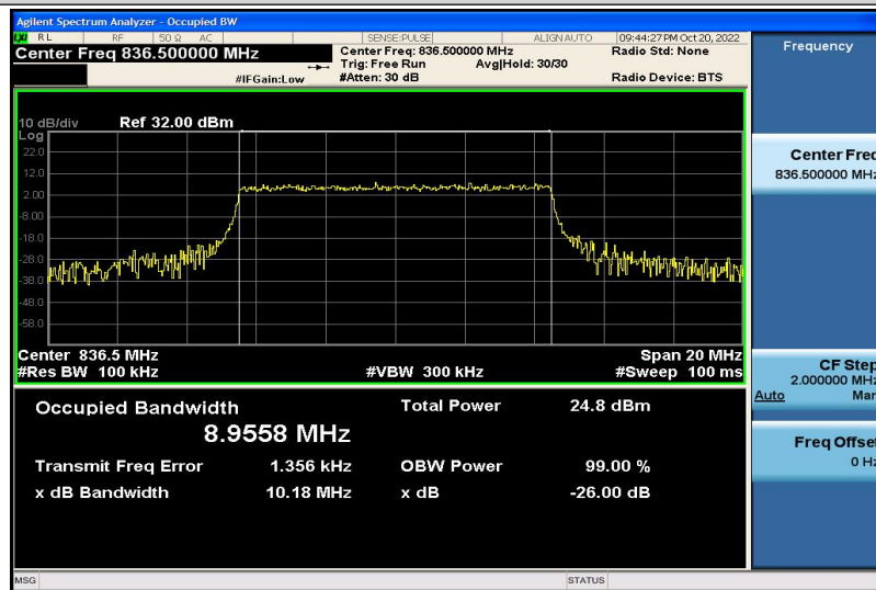
Band5-10MHz-16QAM-20525-50RB#0-8.9558
