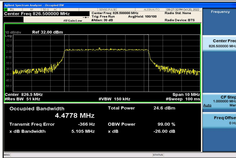
Band5-5MHz-16QAM-20425-25RB#0-4.4778
