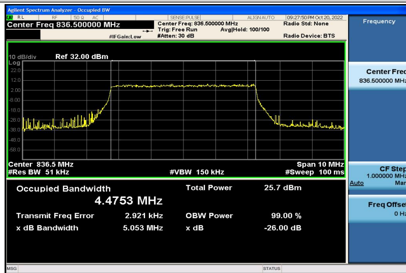
Band5-5MHz-QPSK-20525-25RB#0-4.4753
