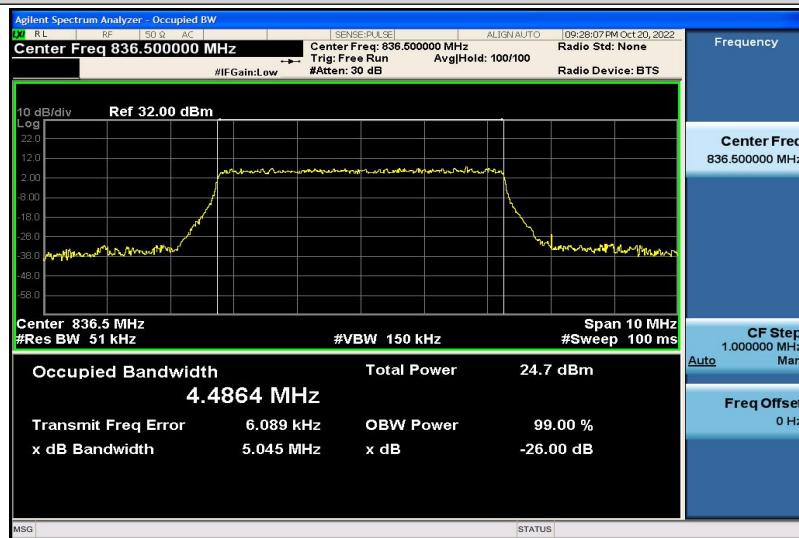
Band5-5MHz-16QAM-20525-25RB#0-4.4864
