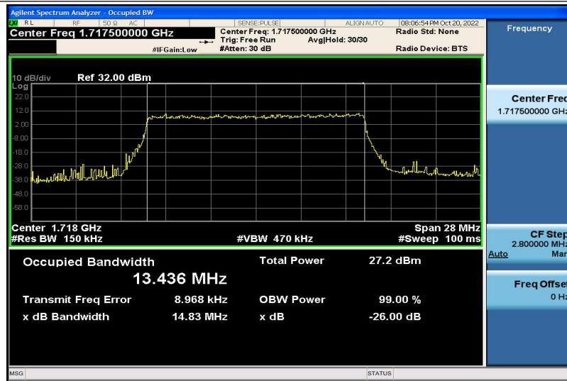
Band4-15MHz-QPSK-20025-75RB#0-13.436
