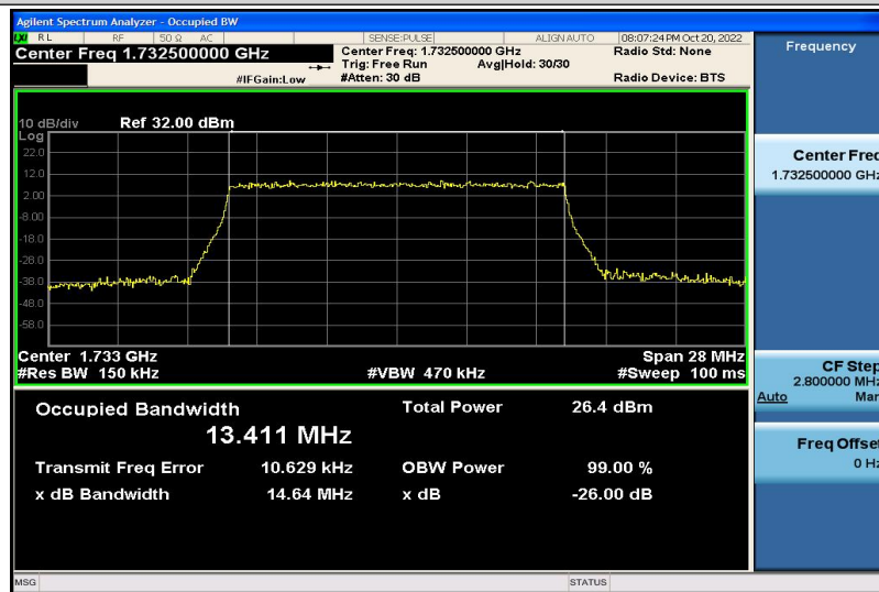
Band4-15MHz-16QAM-20175-75RB#0-13.411
