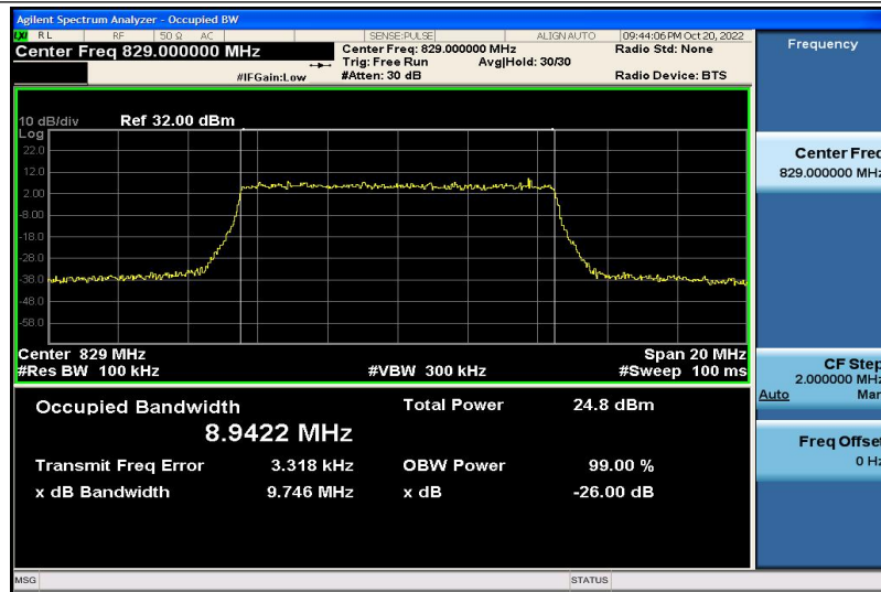
Band5-10MHz-16QAM-20450-50RB#0-8.9422
