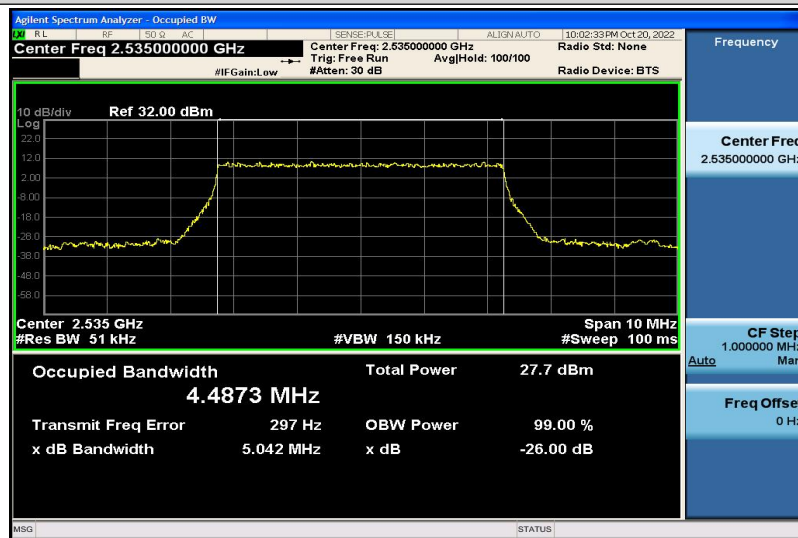
Band7-5MHz-QPSK-21100-25RB#0-4.4873
