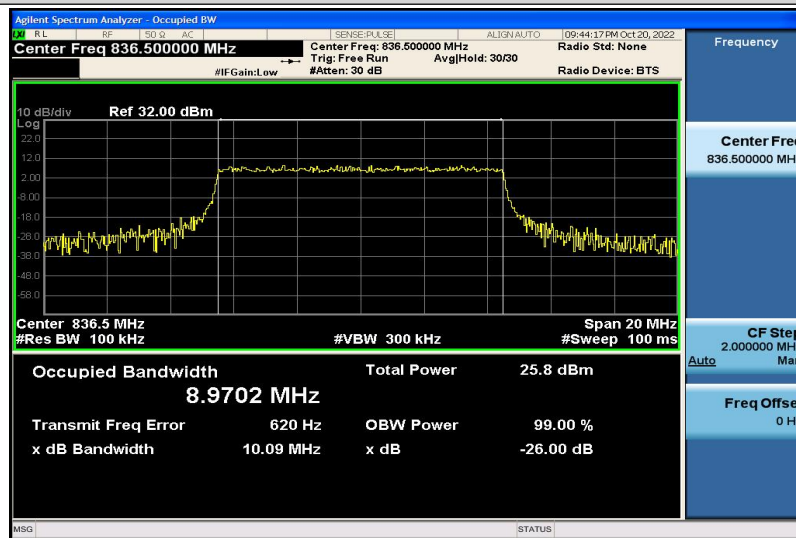
Band5-10MHz-QPSK-20525-50RB#0-8.9702
