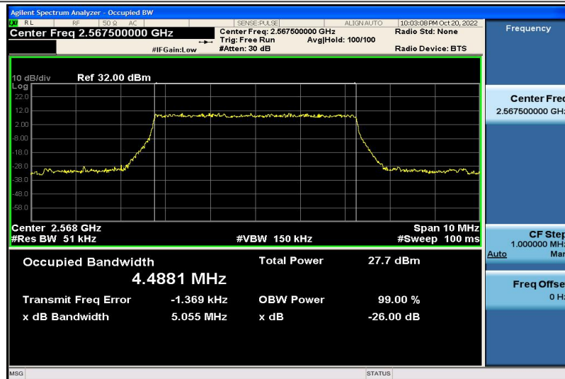
Band7-5MHz-QPSK-21425-25RB#0-4.4881
