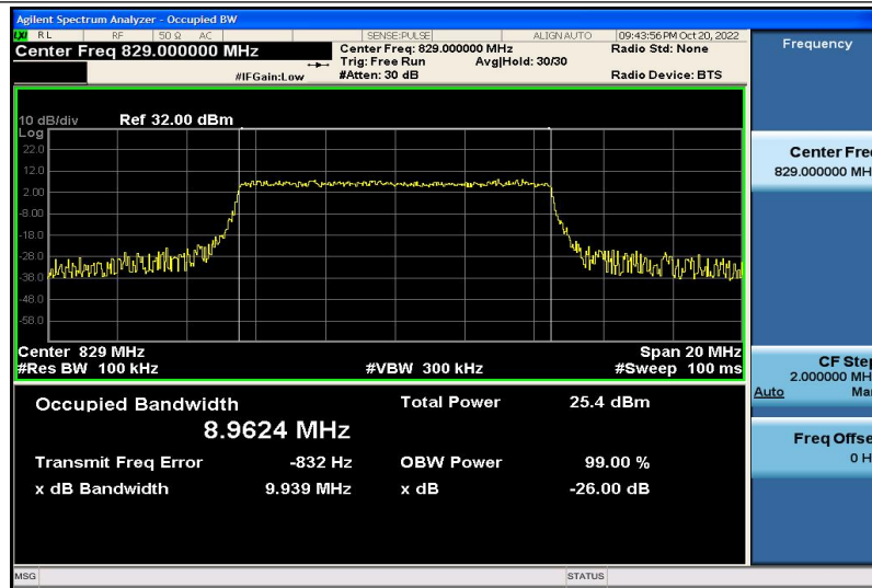
Band5-10MHz-QPSK-20450-50RB#0-8.9624
