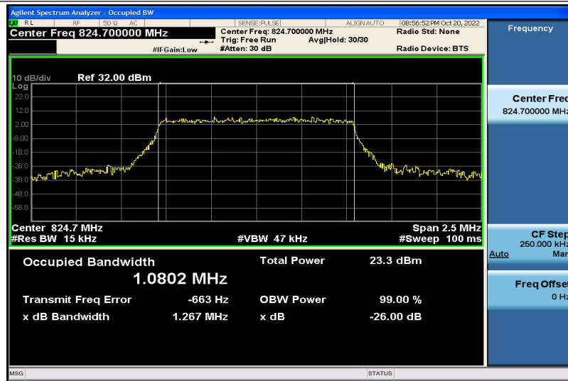
Band5-1.4MHz-16QAM-20407-6RB#0-1.0802
