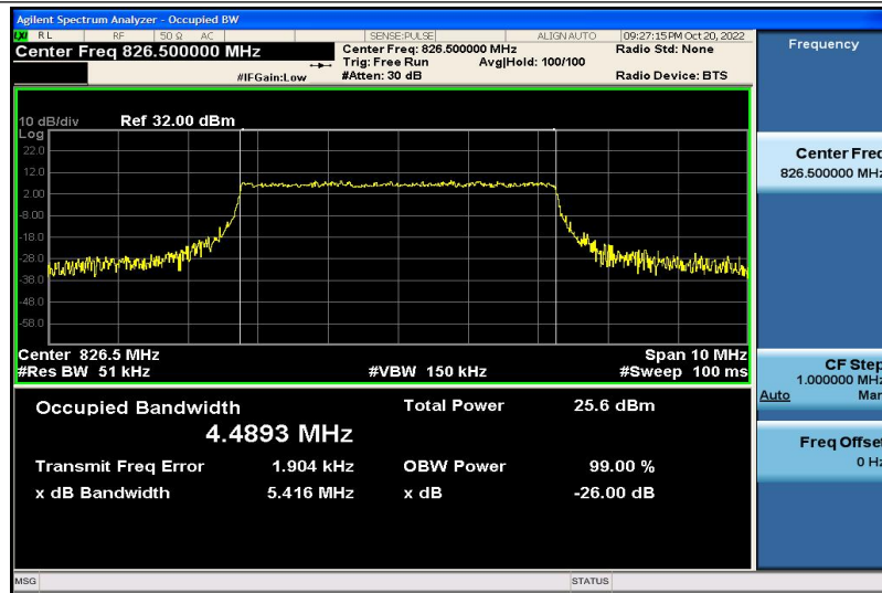
Band5-5MHz-QPSK-20425-25RB#0-4.4893
