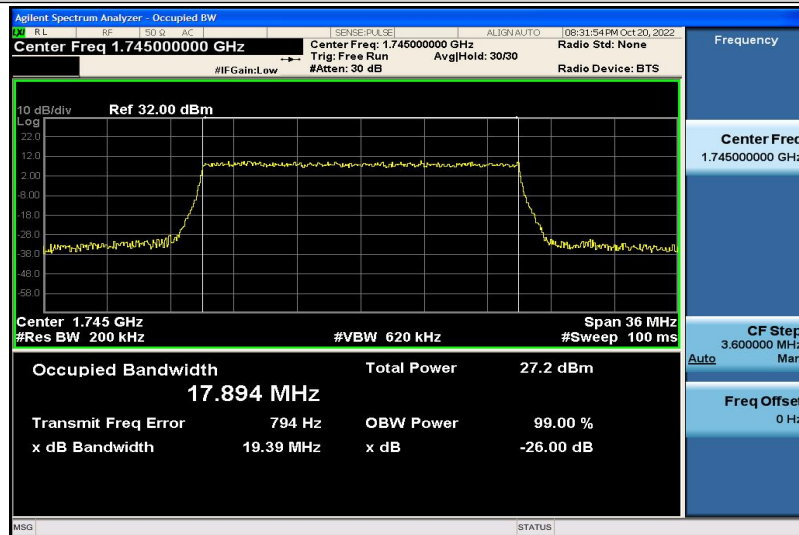
Band4-20MHz-16QAM-20300-100RB#0-17.894
