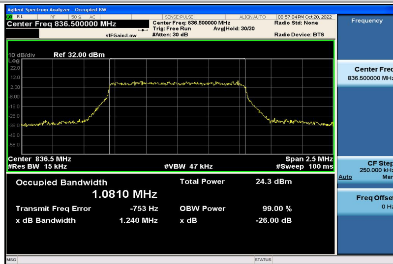
Band5-1.4MHz-QPSK-20525-6RB#0-1.0810
