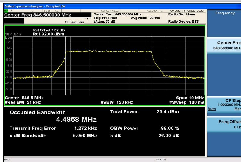
Band5-5MHz-QPSK-20625-25RB#0-4.4858
