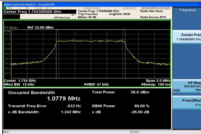
Band4-1.4MHz-QPSK-20393-6RB#0-1.0779
