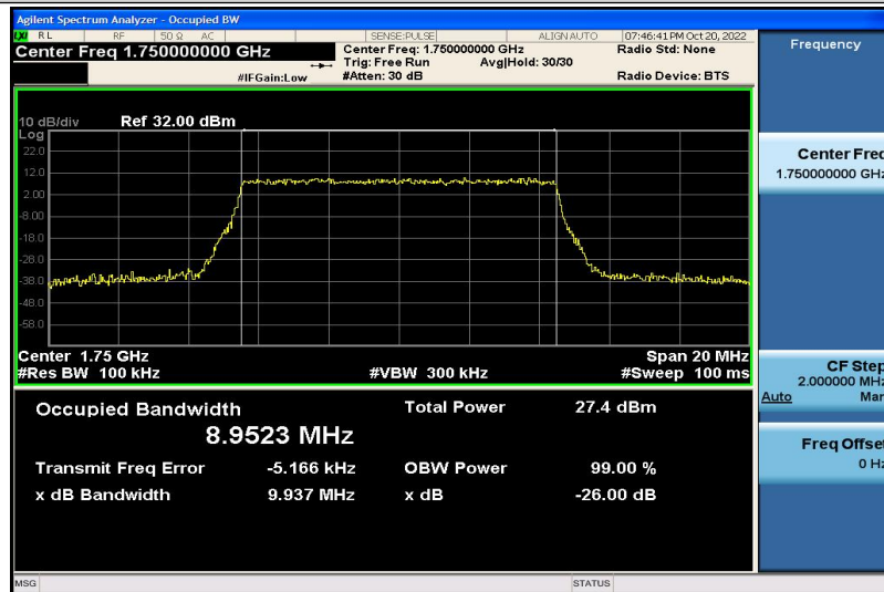
Band4-10MHz-QPSK-20350-50RB#0-8.9523
