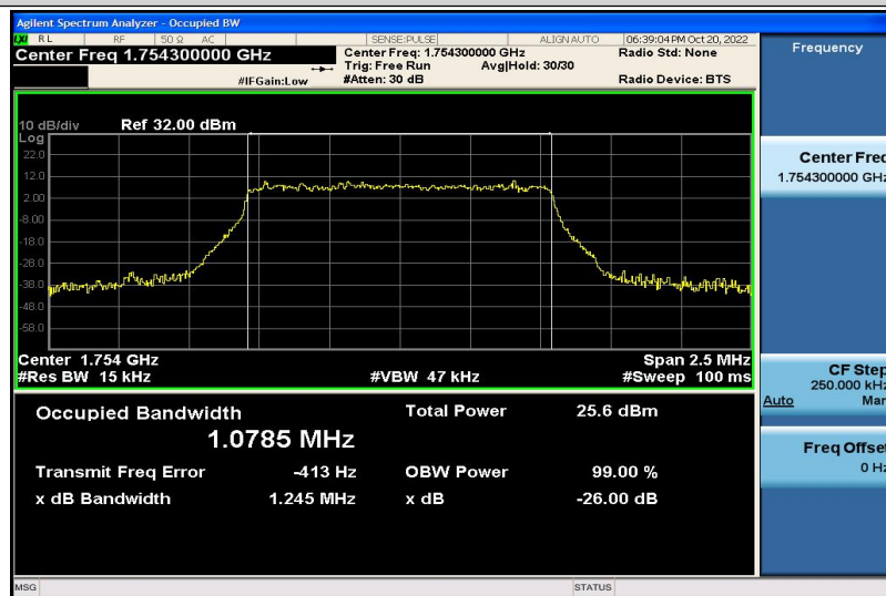
Band4-1.4MHz-16QAM-20393-6RB#0-1.0785
