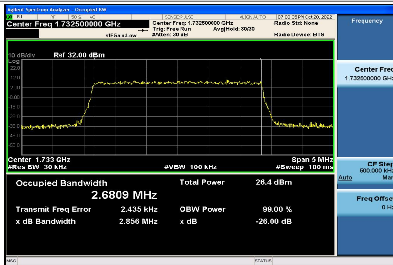
Band4-3MHz-QPSK-20175-15RB#0-2.6809
