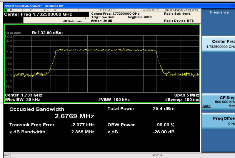
Band4-3MHz-16QAM-20175-15RB#0-2.6769
