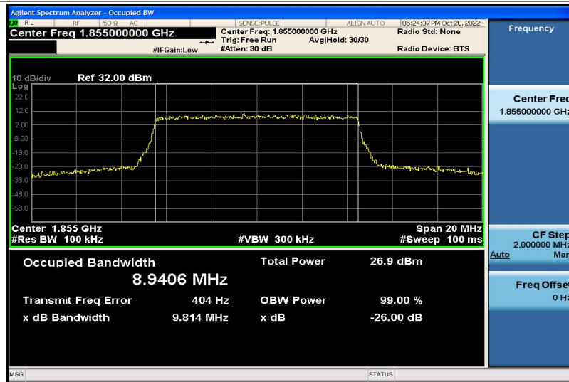
Band2-10MHz-16QAM-18650-50RB#0-8.9406
