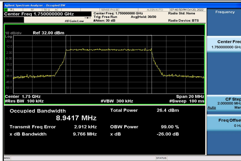
Band4-10MHz-16QAM-20350-50RB#0-8.9417
