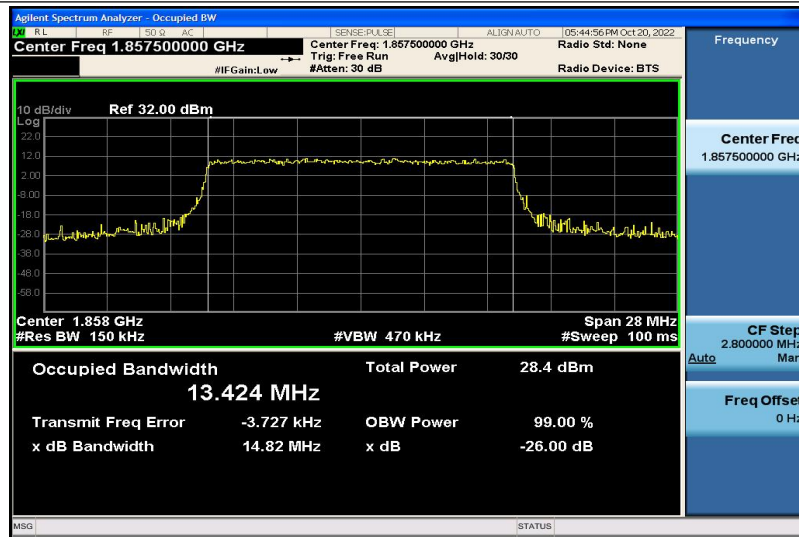
Band2-15MHz-QPSK-18675-75RB#0-13.424
