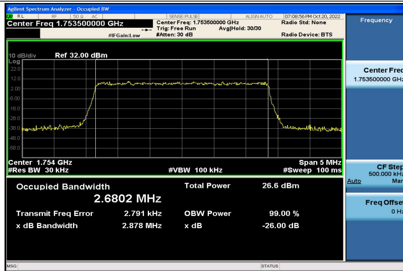
Band4-3MHz-QPSK-20385-15RB#0-2.6802
