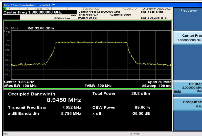
Band2-10MHz-16QAM-18900-50RB#0-8.9450
