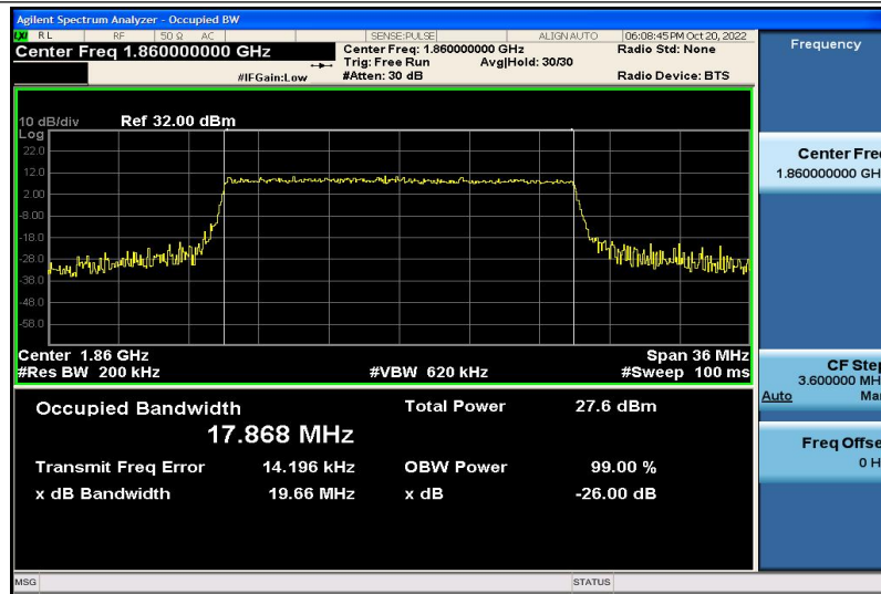
Band2-20MHz-16QAM-18700-100RB#0-17.868
