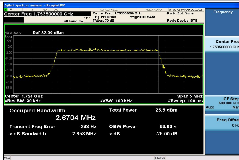
Band4-3MHz-16QAM-20385-15RB#0-2.6704
