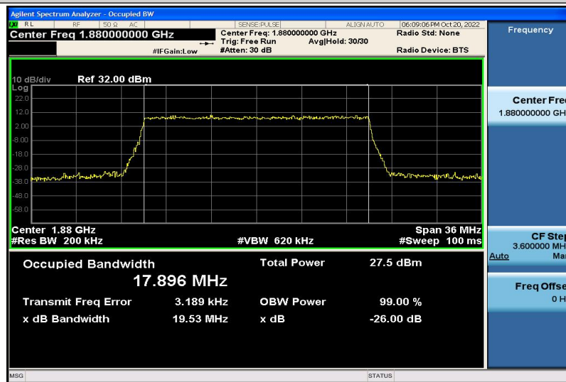
Band2-20MHz-16QAM-18900-100RB#0-17.896
