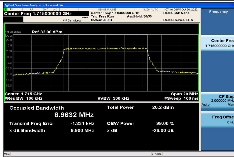
Band4-10MHz-16QAM-20000-50RB#0-8.9632
