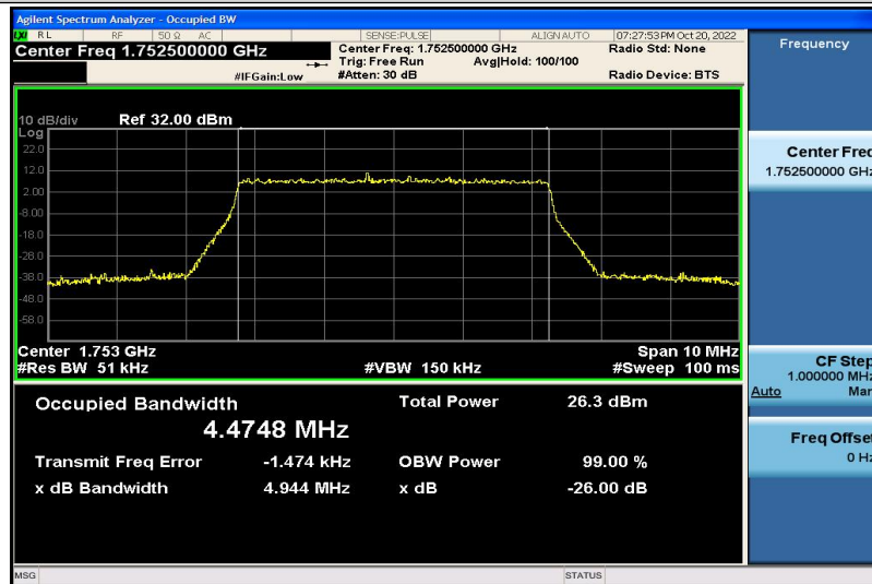
Band4-5MHz-16QAM-20375-25RB#0-4.4748
