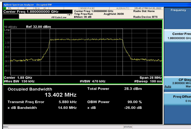
Band2-15MHz-QPSK-18900-75RB#0-13.402
