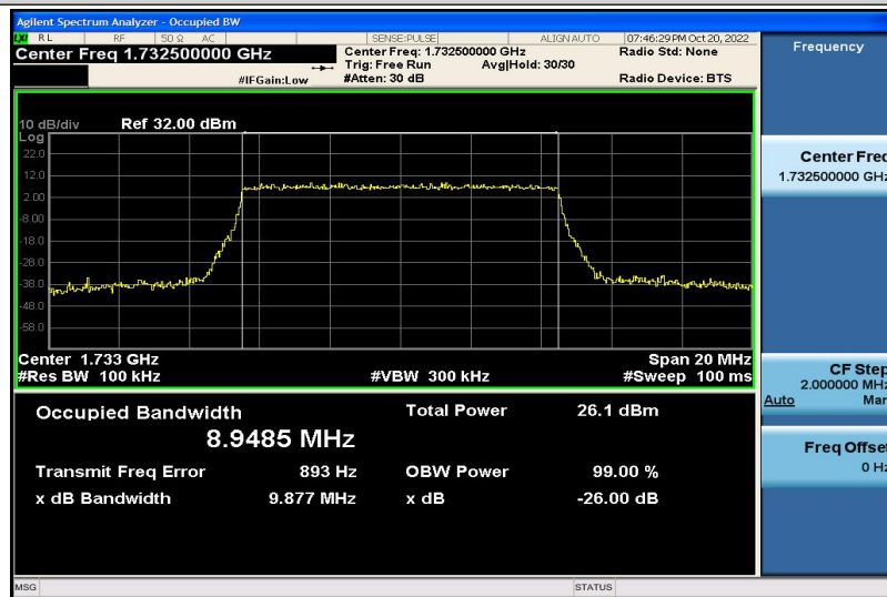
Band4-10MHz-16QAM-20175-50RB#0-8.9485
