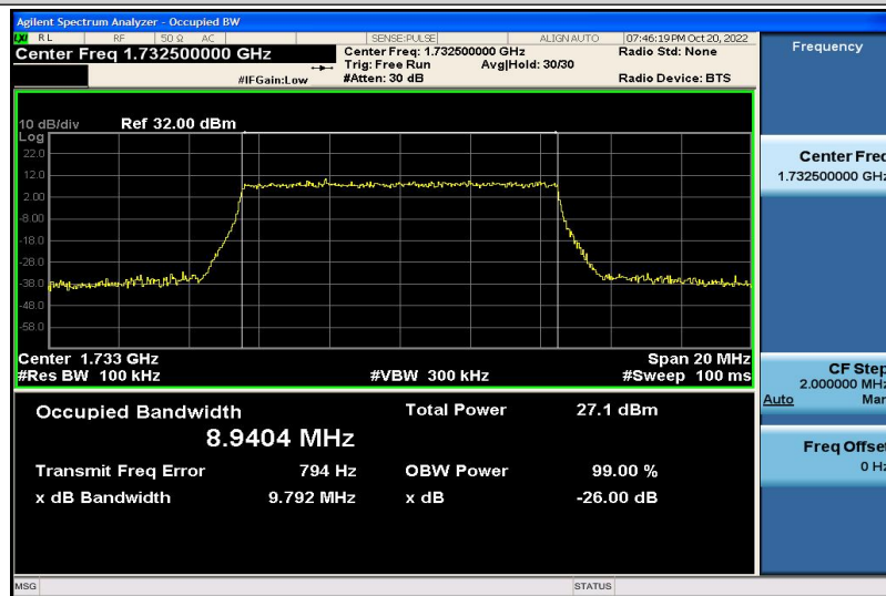
Band4-10MHz-QPSK-20175-50RB#0-8.9404
