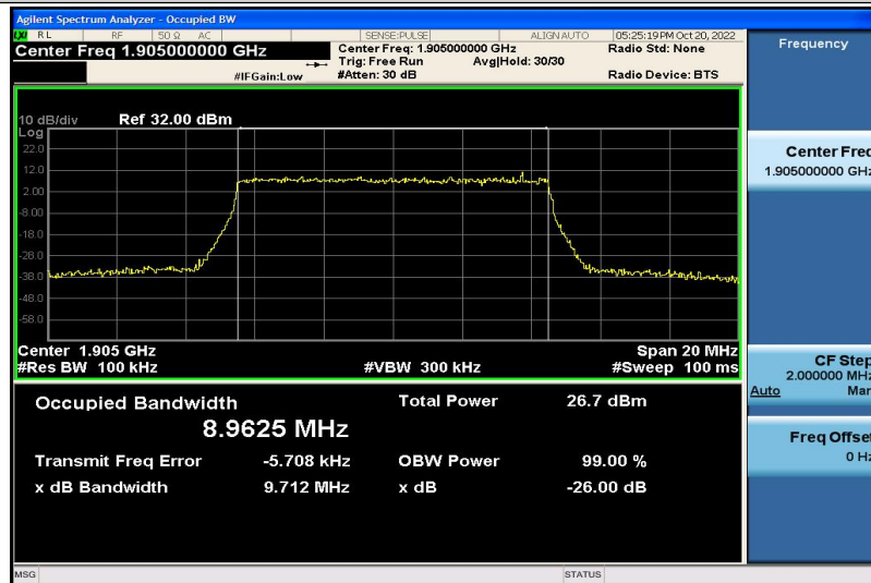
Band2-10MHz-16QAM-19150-50RB#0-8.9625
