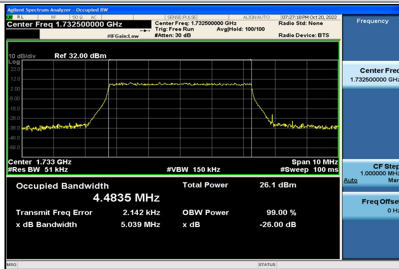
Band4-5MHz-16QAM-20175-25RB#0-4.4835
