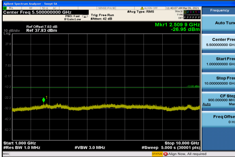
GSM850-190-1000~10000
