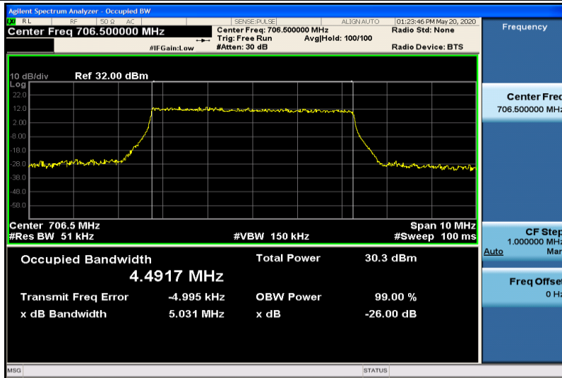
Band17-5MHz-QPSK-23755-25RB#0-4.4917
