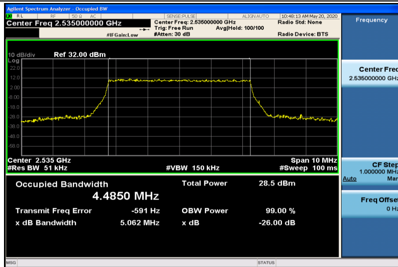
Band7-5MHz-16QAM-21100-25RB#0-4.4850
