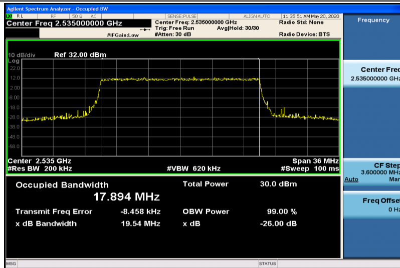
Band7-20MHz-QPSK-21100-100RB#0-17.894
