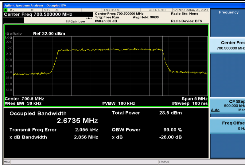
Band12-3MHz-16QAM-23025-15RB#0-2.6735
