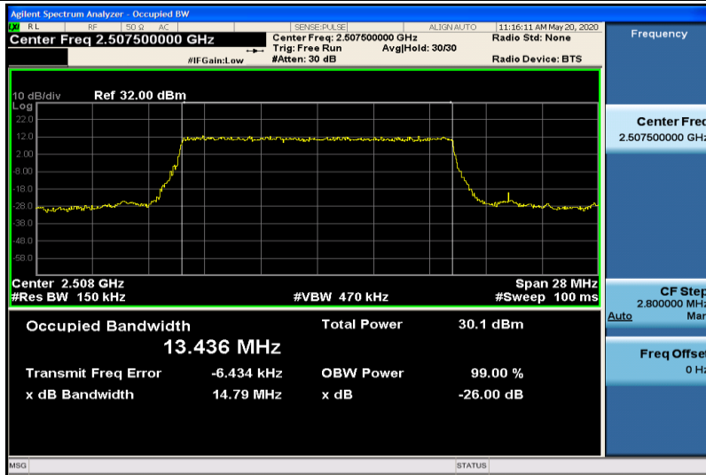
Band7-15MHz-QPSK-20825-75RB#0-13.436
