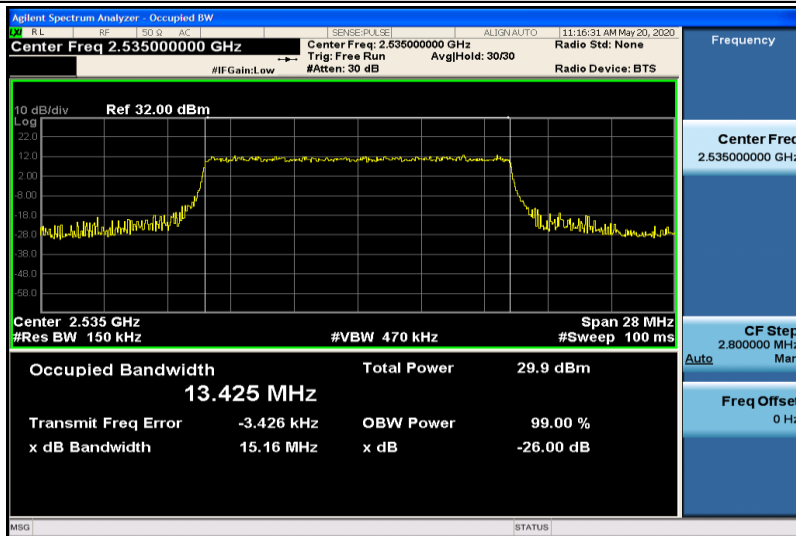
Band7-15MHz-QPSK-21100-75RB#0-13.425
