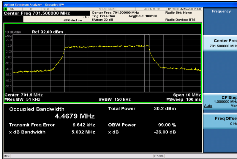
Band12-5MHz-QPSK-23035-25RB#0-4.4679
