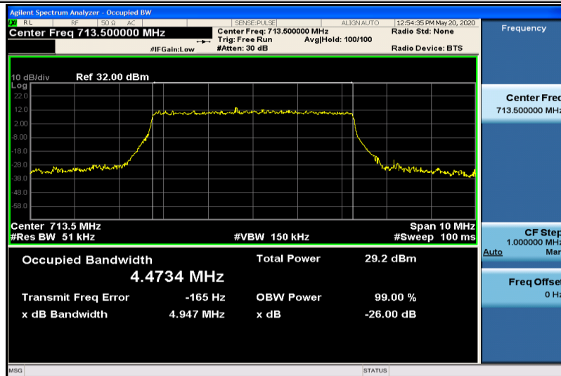
Band12-5MHz-16QAM-23155-25RB#0-4.4734
