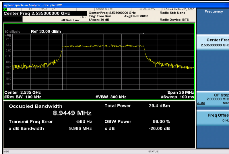
Band7-10MHz-QPSK-21100-50RB#0-8.9449
