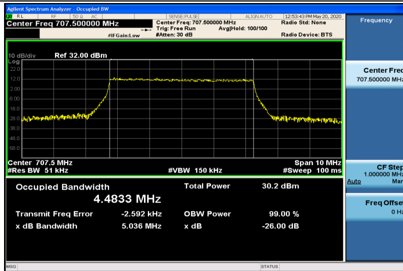
Band12-5MHz-QPSK-23095-25RB#0-4.4833
