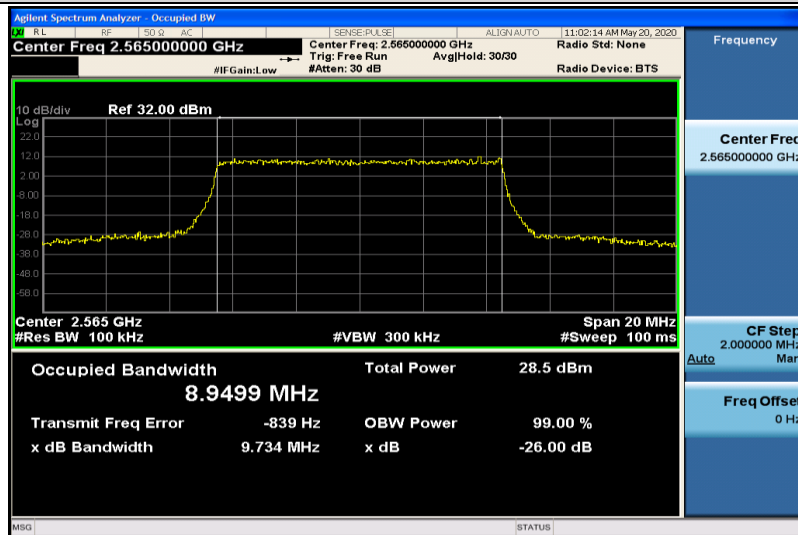
Band7-10MHz-16QAM-21400-50RB#0-8.9499
