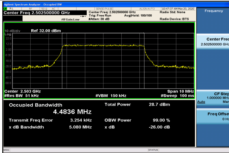
Band7-5MHz-16QAM-20775-25RB#0-4.4836
