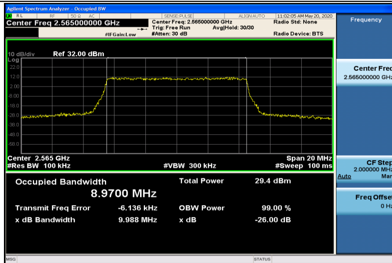
Band7-10MHz-QPSK-21400-50RB#0-8.9700
