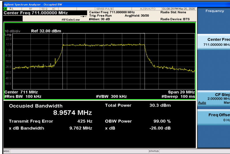
Band12-10MHz-QPSK-23130-50RB#0-8.9574
