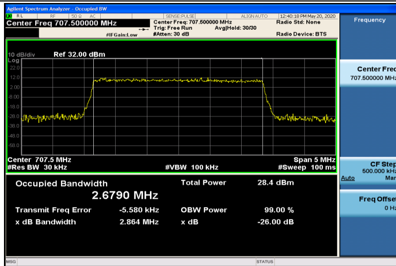
Band12-3MHz-16QAM-23095-15RB#0-2.6790
