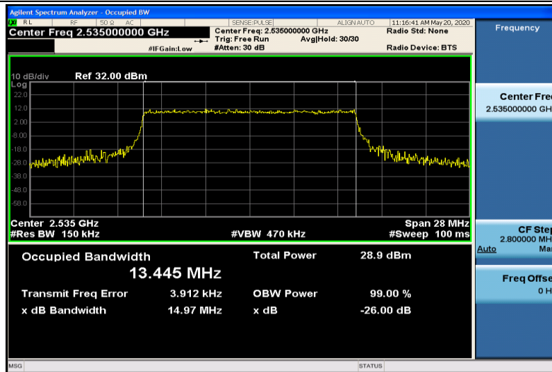
Band7-15MHz-16QAM-21100-75RB#0-13.445
