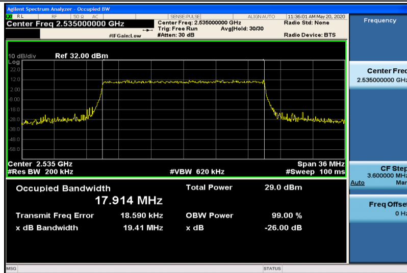
Band7-20MHz-16QAM-21100-100RB#0-17.914
