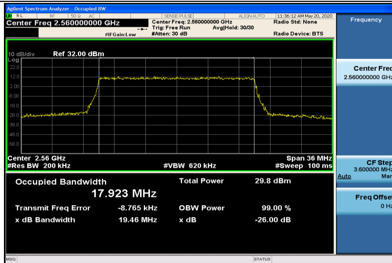
Band7-20MHz-QPSK-21350-100RB#0-17.923
