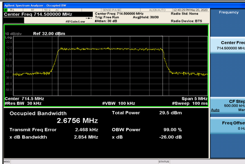
Band12-3MHz-QPSK-23165-15RB#0-2.6756
