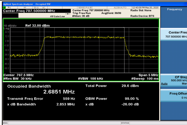
Band12-3MHz-QPSK-23095-15RB#0-2.6851
