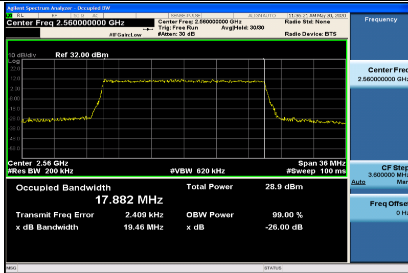
Band7-20MHz-16QAM-21350-100RB#0-17.882
