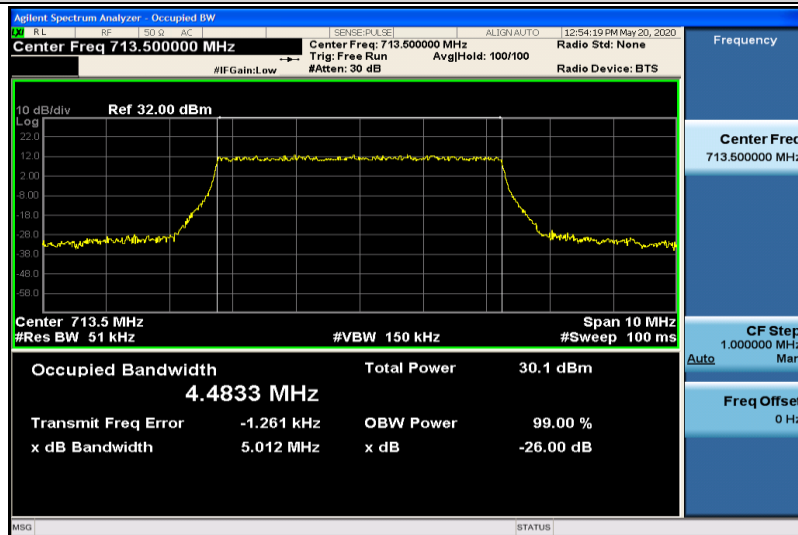
Band12-5MHz-QPSK-23155-25RB#0-4.4833
