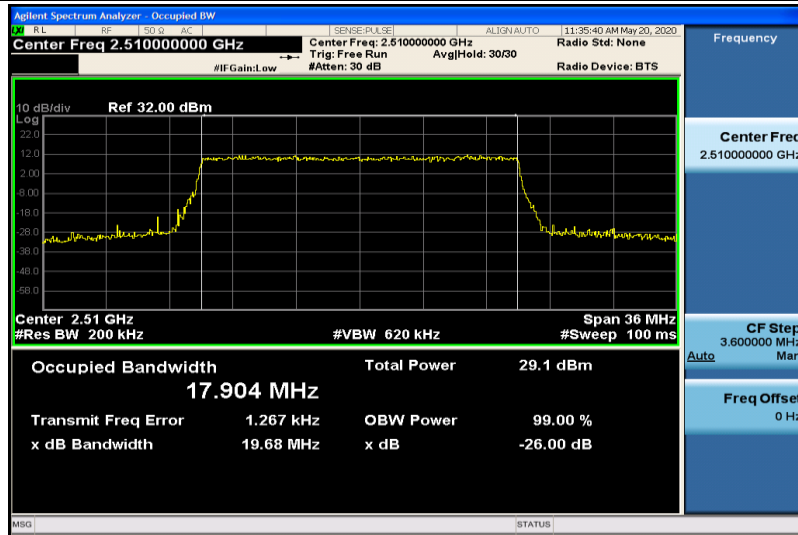
Band7-20MHz-16QAM-20850-100RB#0-17.904
