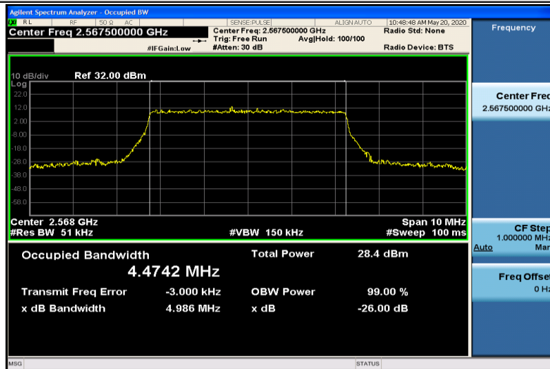
Band7-5MHz-16QAM-21425-25RB#0-4.4742
