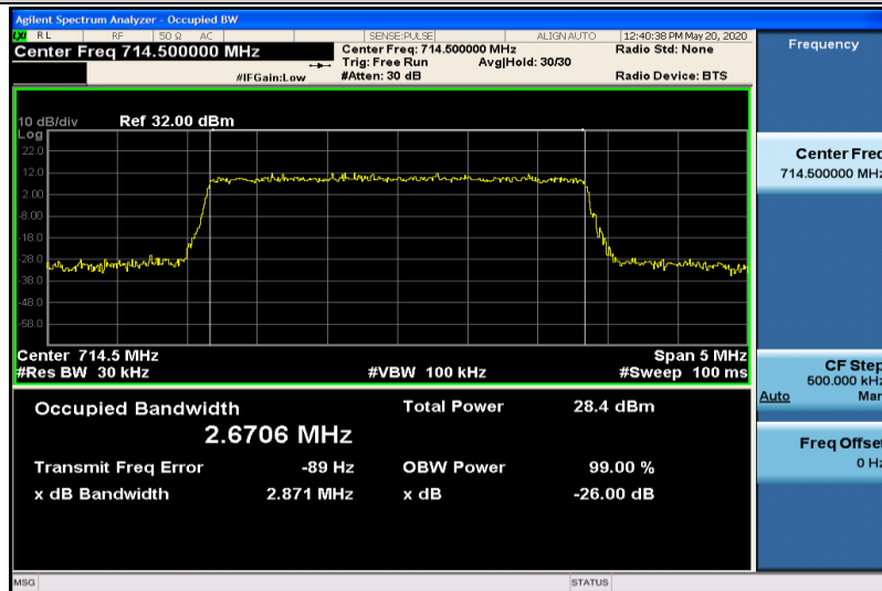
Band12-3MHz-16QAM-23165-15RB#0-2.6706
