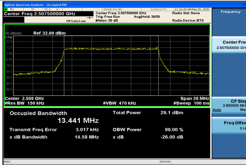
Band7-15MHz-16QAM-20825-75RB#0-13.441
