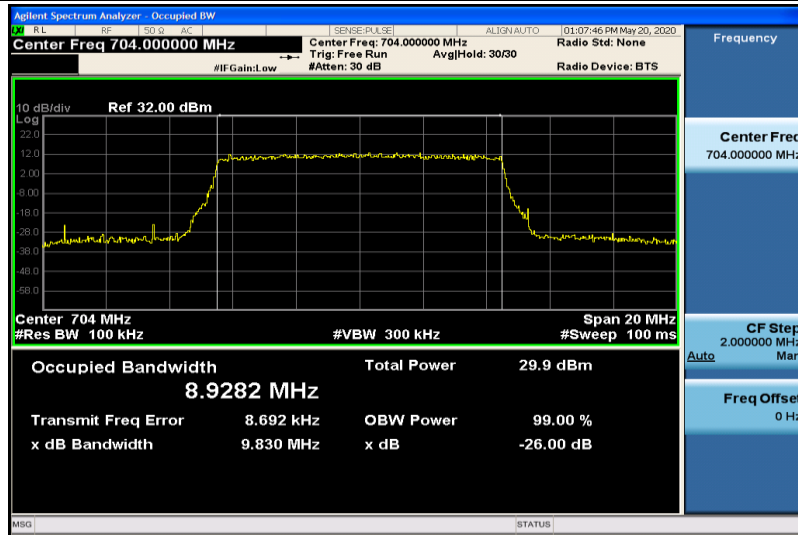
Band12-10MHz-QPSK-23060-50RB#0-8.9282
