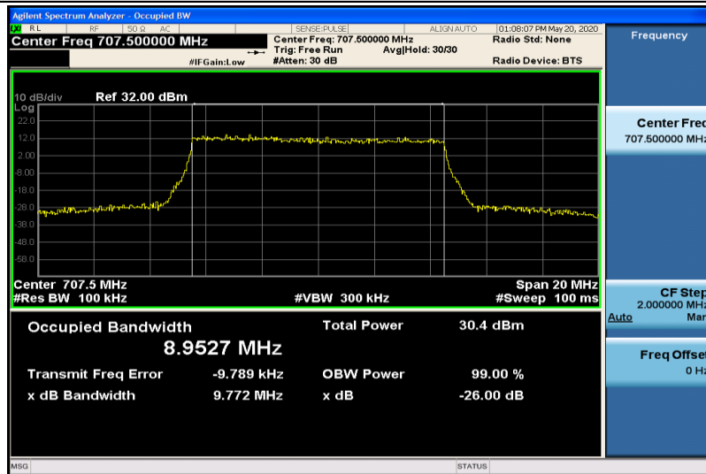
Band12-10MHz-QPSK-23095-50RB#0-8.9527
