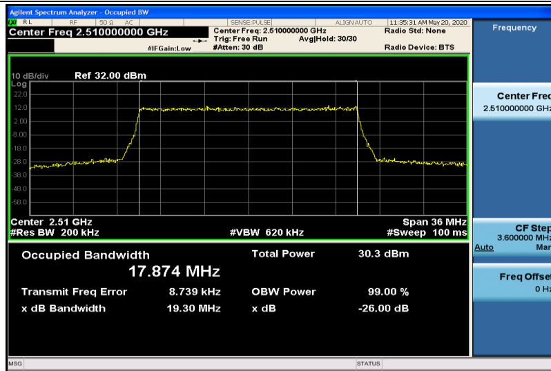
Band7-20MHz-QPSK-20850-100RB#0-17.874
