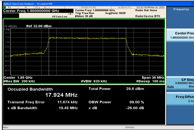
Band2-20MHz-16QAM-18700-100RB#0-17.924
