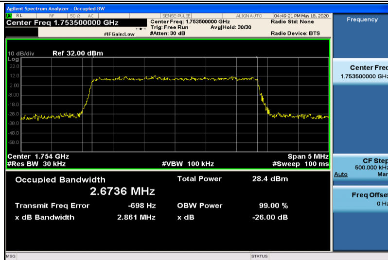
Band4-3MHz-QPSK-20385-15RB#0-2.6736
