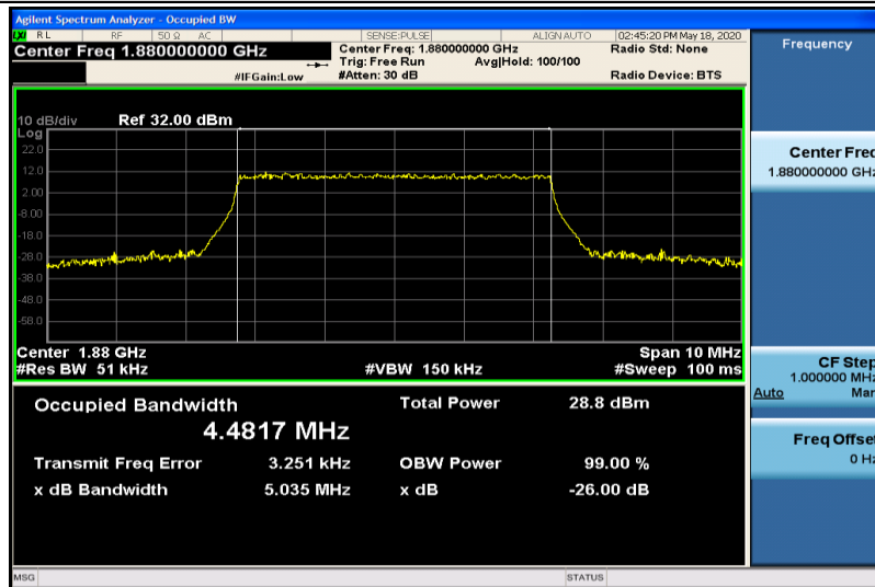
Band2-5MHz-16QAM-18900-25RB#0-4.4817
