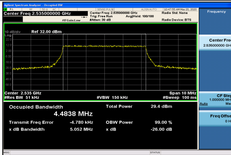
Band7-5MHz-QPSK-21100-25RB#0-4.4838
