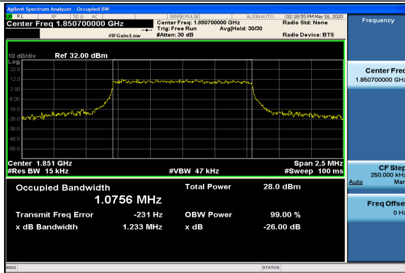
Band2-1.4MHz-16QAM-18607-6RB#0-1.0756
