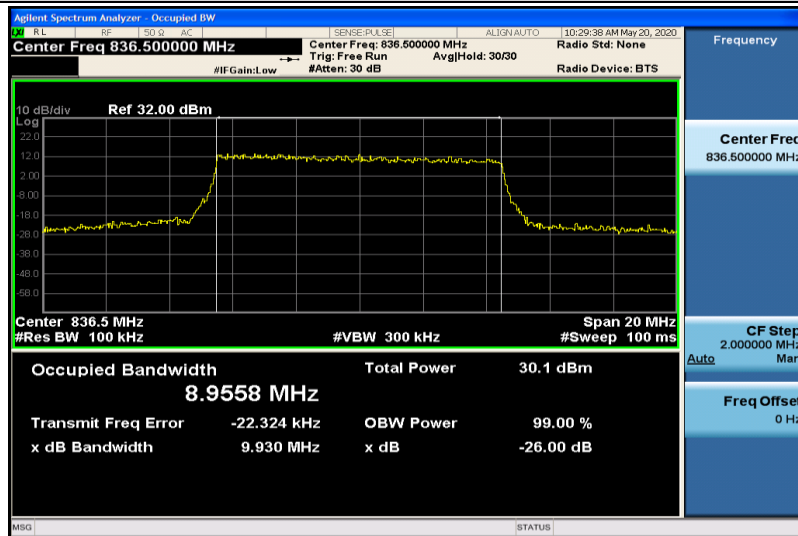
Band5-10MHz-QPSK-20525-50RB#0-8.9558
