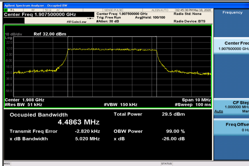
Band2-5MHz-QPSK-19175-25RB#0-4.4863
