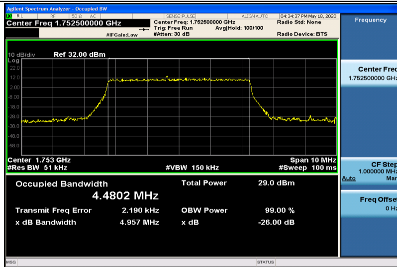
Band4-5MHz-16QAM-20375-25RB#0-4.4802
