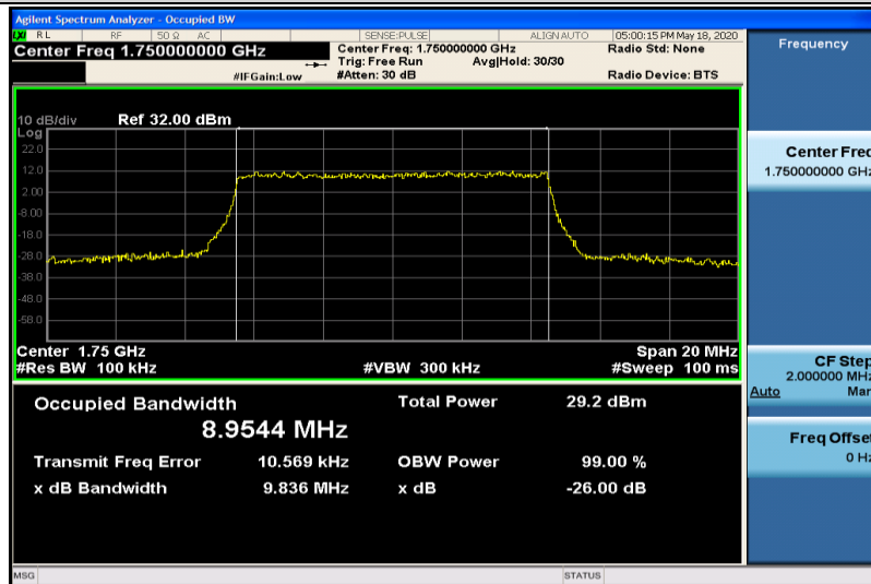
Band4-10MHz-16QAM-20350-50RB#0-8.9544
