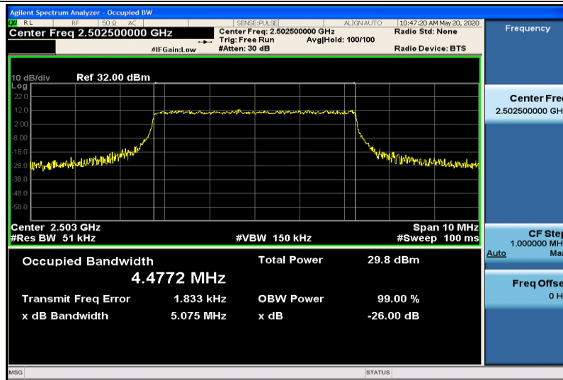
Band7-5MHz-QPSK-20775-25RB#0-4.4772
