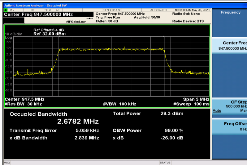
Band5-3MHz-QPSK-20635-15RB#0-2.6782
