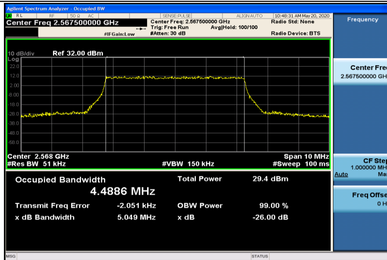
Band7-5MHz-QPSK-21425-25RB#0-4.4886
