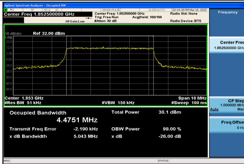
Band2-5MHz-QPSK-18625-25RB#0-4.4751
