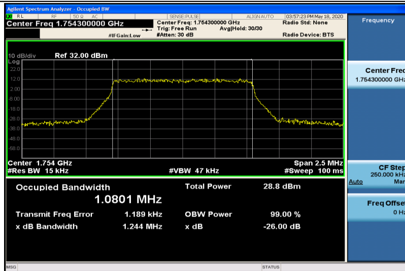
Band4-1.4MHz-QPSK-20393-6RB#0-1.0801
