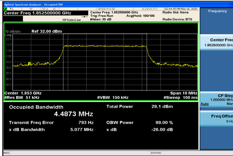
Band2-5MHz-16QAM-18525-25RB#0-4.4873
