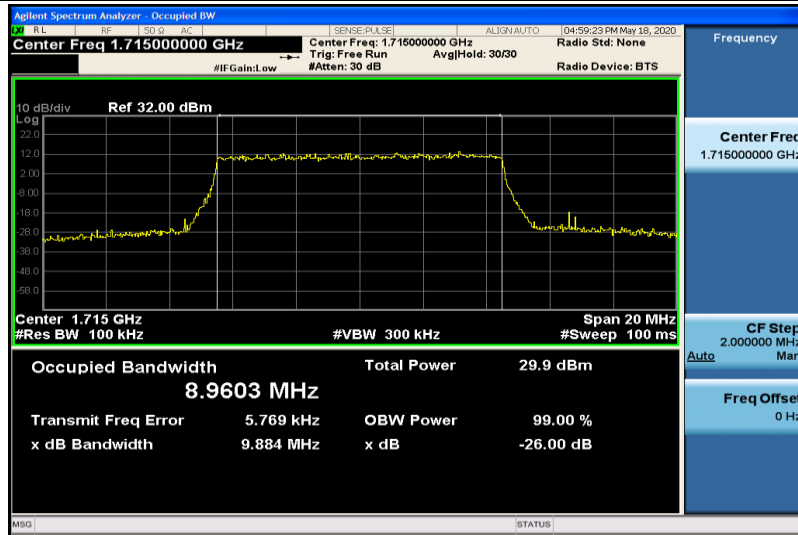
Band4-10MHz-QPSK-20000-50RB#0-8.9603
