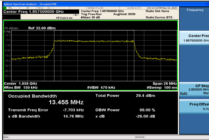
Band2-15MHz-16QAM-18675-75RB#0-13.455
