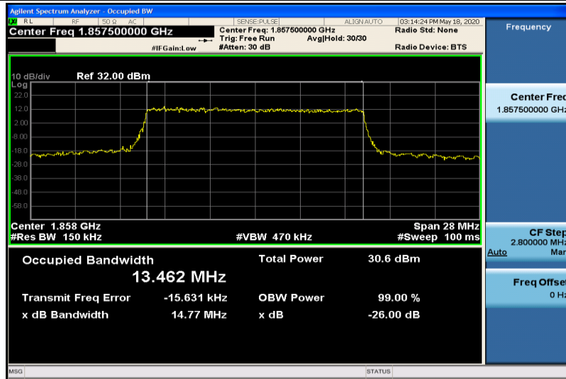
Band2-15MHz-QPSK-18675-75RB#0-13.462
