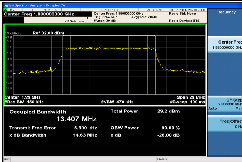
Band2-15MHz-16QAM-18900-75RB#0-13.407
