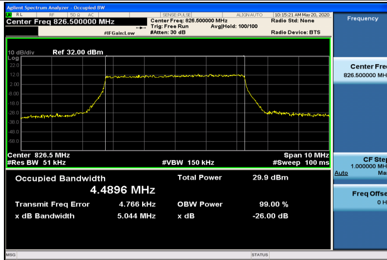
Band5-5MHz-QPSK-20425-25RB#0-4.4896
