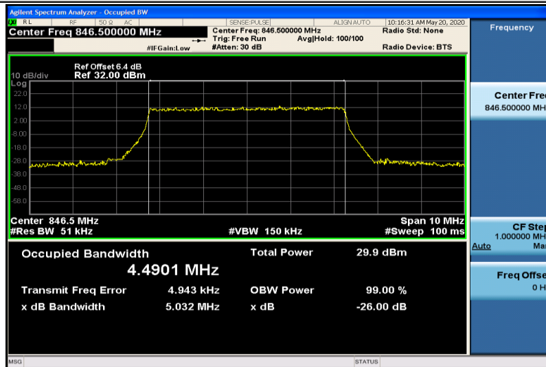
Band5-5MHz-QPSK-20625-25RB#0-4.4901
