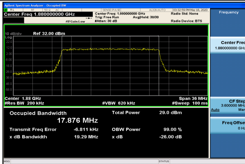
Band2-20MHz-16QAM-18900-100RB#0-17.876
