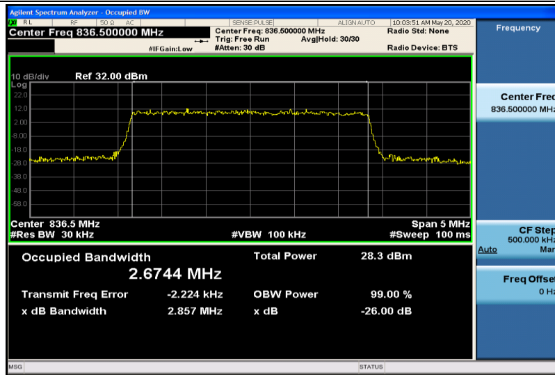
Band5-3MHz-16QAM-20525-15RB#0-2.6744
