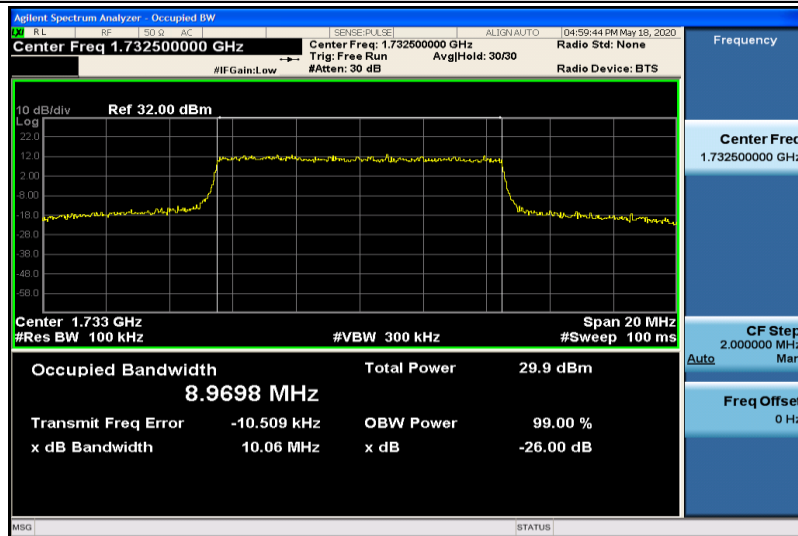
Band4-10MHz-QPSK-17325-50RB#0-8.9698
