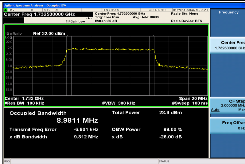
Band4-10MHz-16QAM-20175-50RB#0-8.9811
