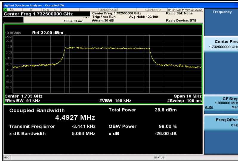
Band4-5MHz-16QAM-20175-25RB#0-4.4927
