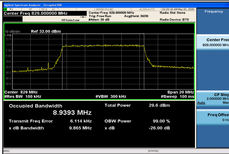
Band5-10MHz-QPSK-20450-50RB#0-8.9393
