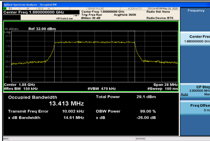
Band2-15MHz-QPSK-18900-75RB#0-13.413
