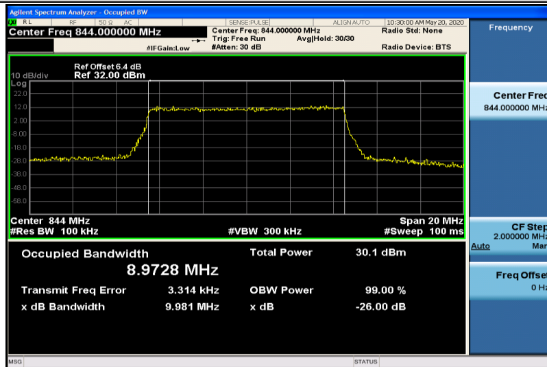
Band5-10MHz-QPSK-20600-50RB#0-8.9728
