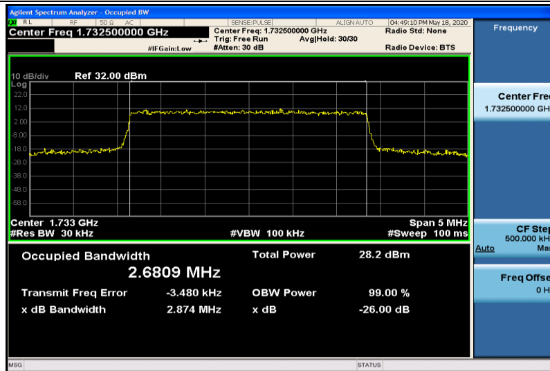
Band4-3MHz-16QAM-20175-15RB#0-2.6809
