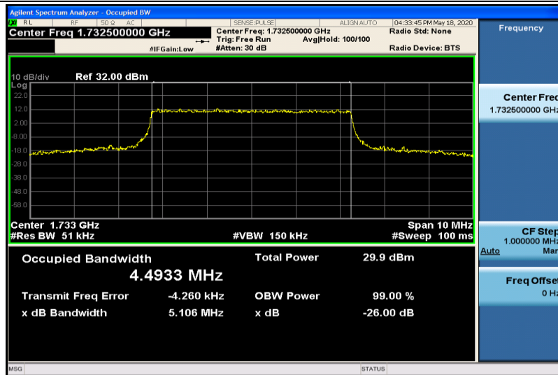
Band4-5MHz-QPSK-17325-25RB#0-4.4933
