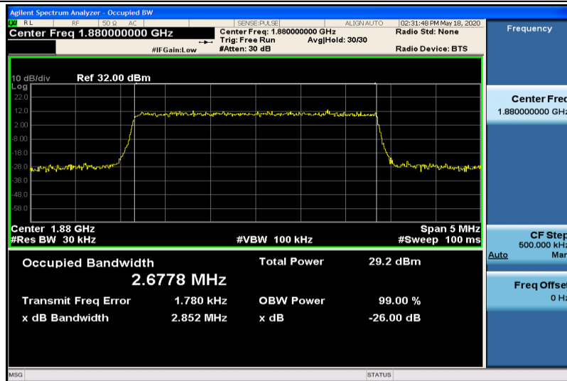
Band2-3MHz-QPSK-18900-15RB#0-2.6778
