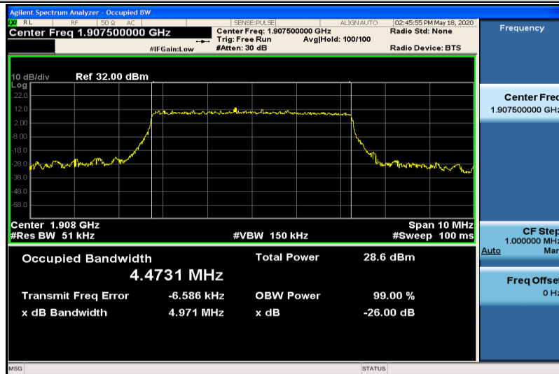
Band2-5MHz-16QAM-19175-25RB#0-4.4731
