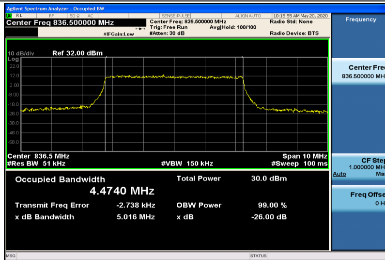
Band5-5MHz-QPSK-20525-25RB#0-4.4740
