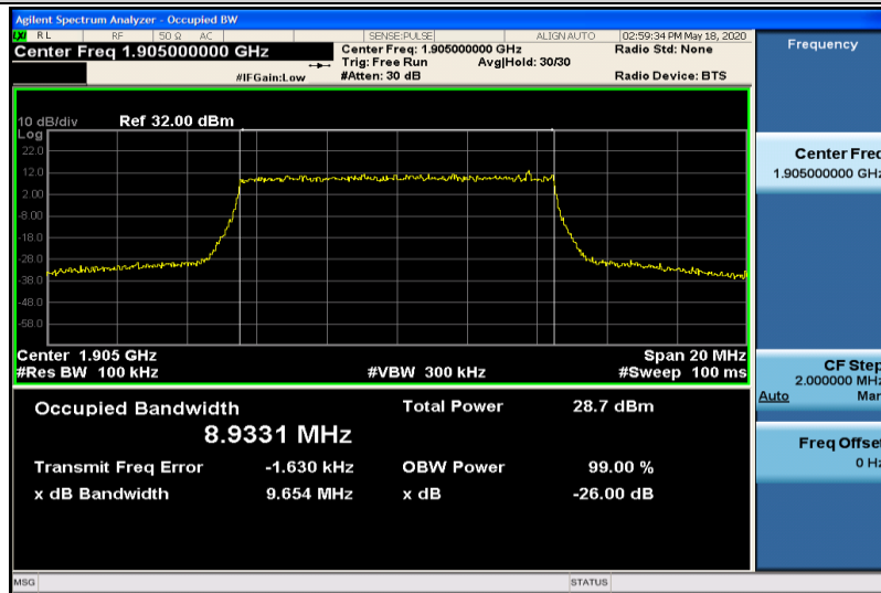
Band2-10MHz-16QAM-19150-50RB#0-8.9331
