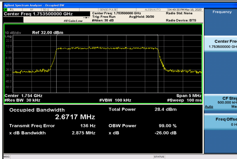
Band4-3MHz-16QAM-20385-15RB#0-2.6717
