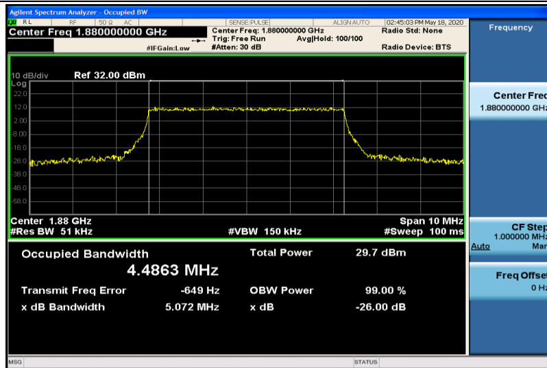
Band2-5MHz-QPSK-18900-25RB#0-4.4863
