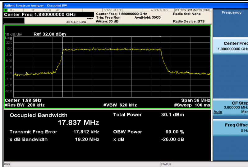
Band2-20MHz-QPSK-18900-100RB#0-17.837
