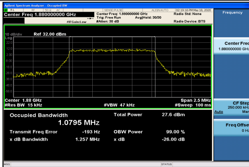
Band2-1.4MHz-16QAM-18900-6RB#0-1.0795
