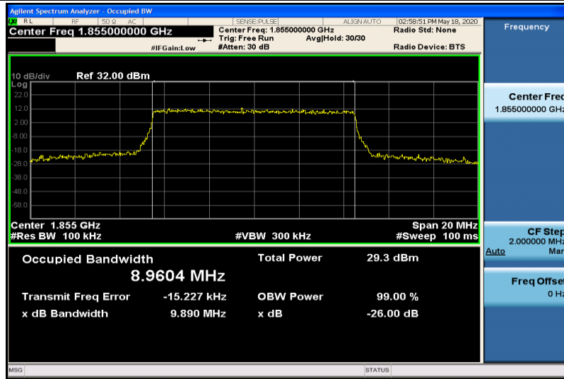
Band2-10MHz-16QAM-18650-50RB#0-8.9604
