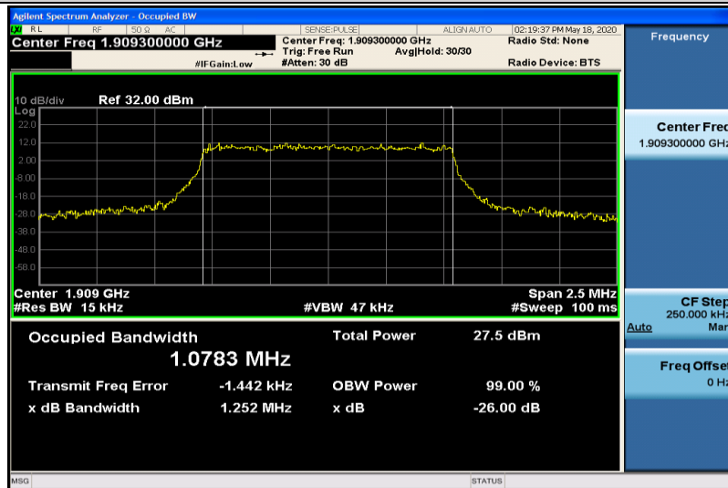
Band2-1.4MHz-16QAM-19193-6RB#0-1.0783
