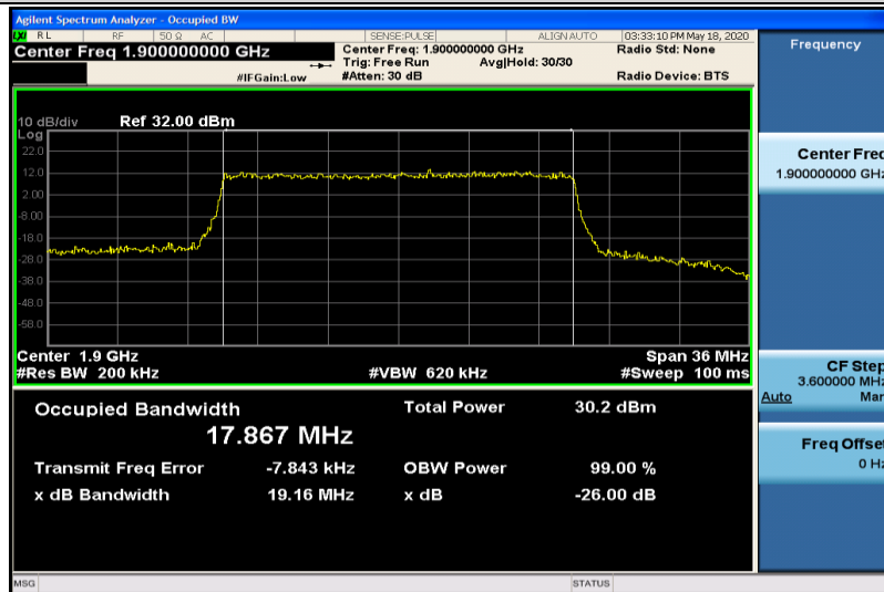
Band2-20MHz-QPSK-19100-100RB#0-17.867
