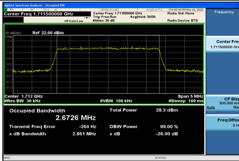
Band4-3MHz-16QAM-19965-15RB#0-2.6726
