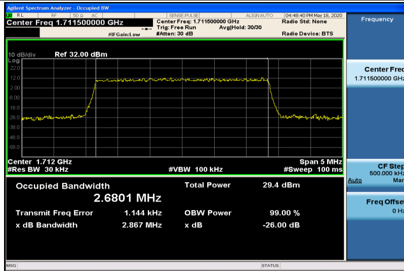
Band4-3MHz-QPSK-19965-15RB#0-2.6801
