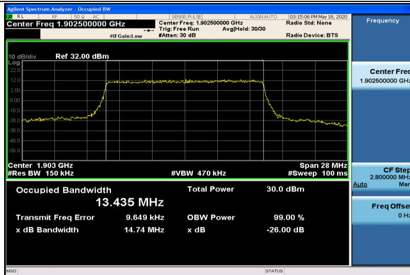
Band2-15MHz-QPSK-19125-75RB#0-13.435
