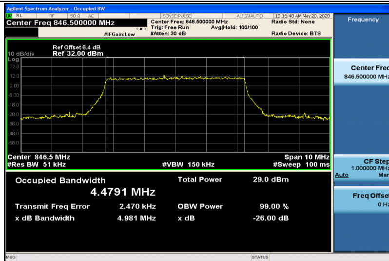
Band5-5MHz-16QAM-20625-25RB#0-4.4791
