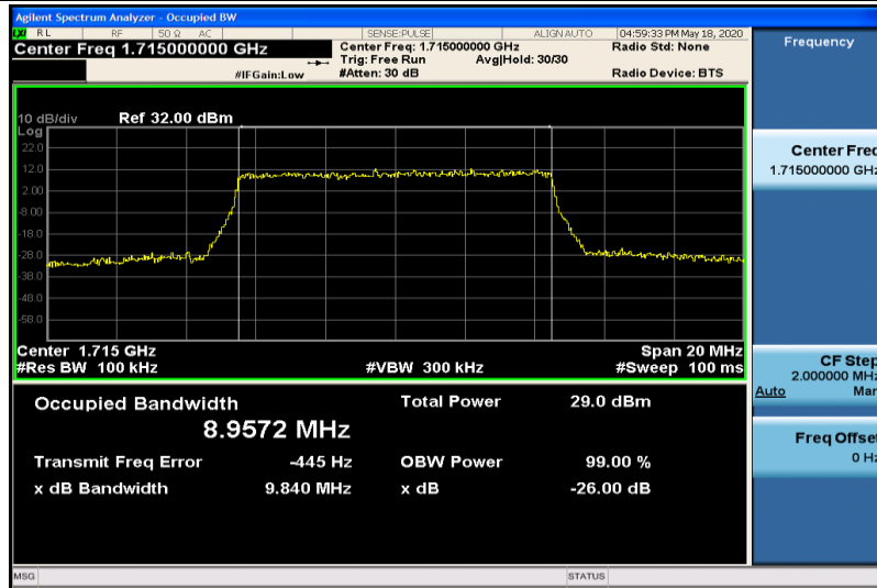
Band4-10MHz-16QAM-20000-50RB#0-8.9572
