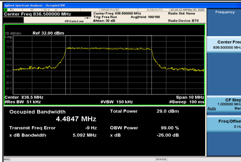
Band5-5MHz-16QAM-20525-25RB#0-4.4847
