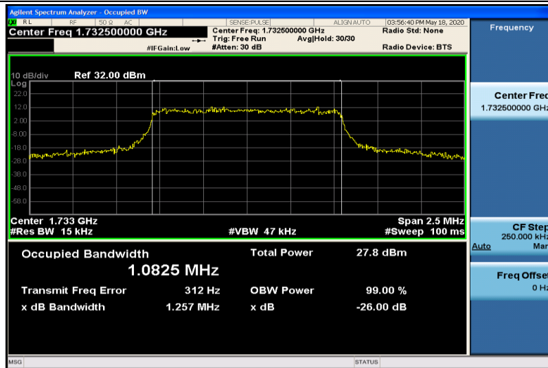
Band4-1.4MHz-16QAM-20175-6RB#0-1.0825
