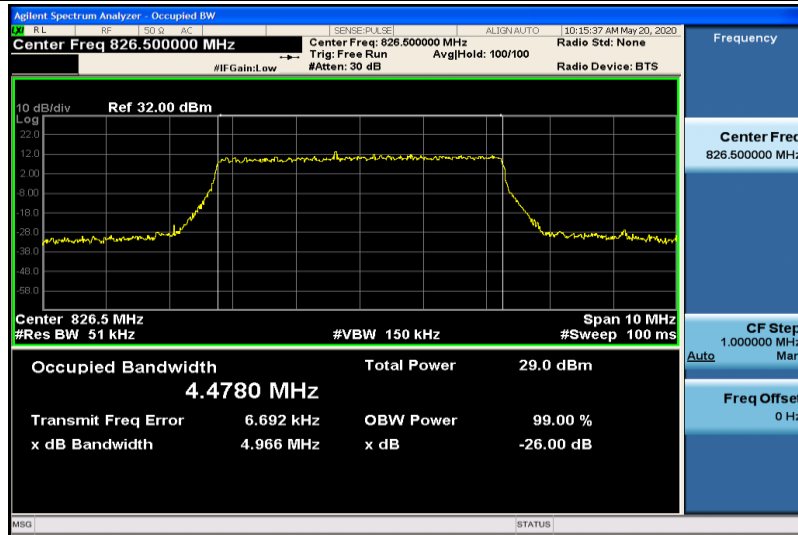
Band5-5MHz-16QAM-20425-25RB#0-4.4780
