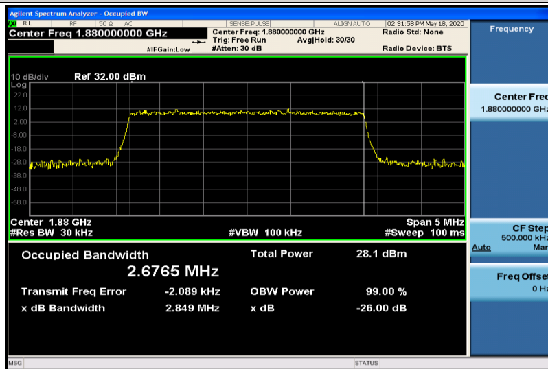
Band2-3MHz-16QAM-18900-15RB#0-2.6765
