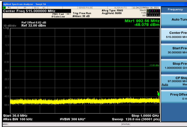
Band2-5MHz-16QAM-18625-1RB#0-30~1000MHz
