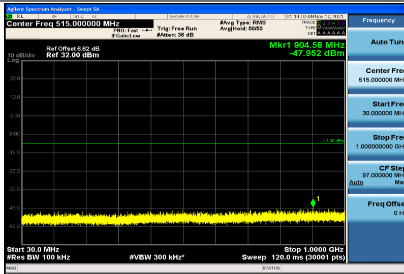
Band4-1.4MHz-QPSK-19957-1RB#0-30~1000MHz
