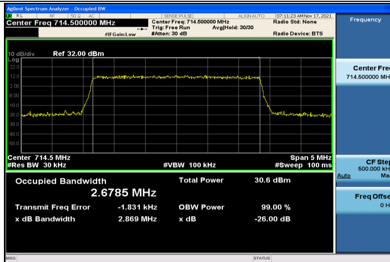
Band12-3MHz-QPSK-23165-15RB#0-2.6785
