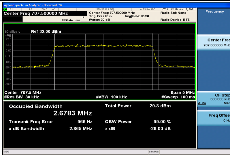
Band12-3MHz-16QAM-23095-15RB#0-2.6783
