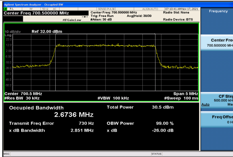
Band12-3MHz-QPSK-23025-15RB#0-2.6736
