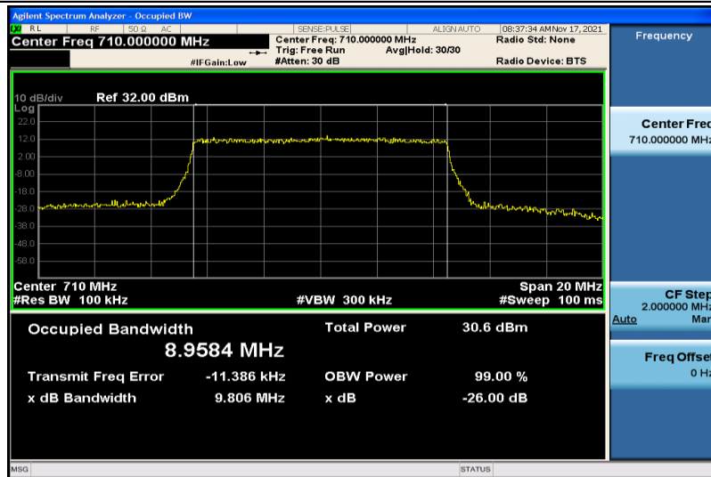
Band17-10MHz-16QAM-23790-50RB#0-8.9584
