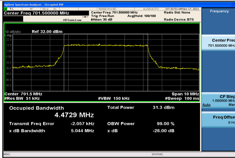
Band12-5MHz-QPSK-23035-25RB#0-4.4729
