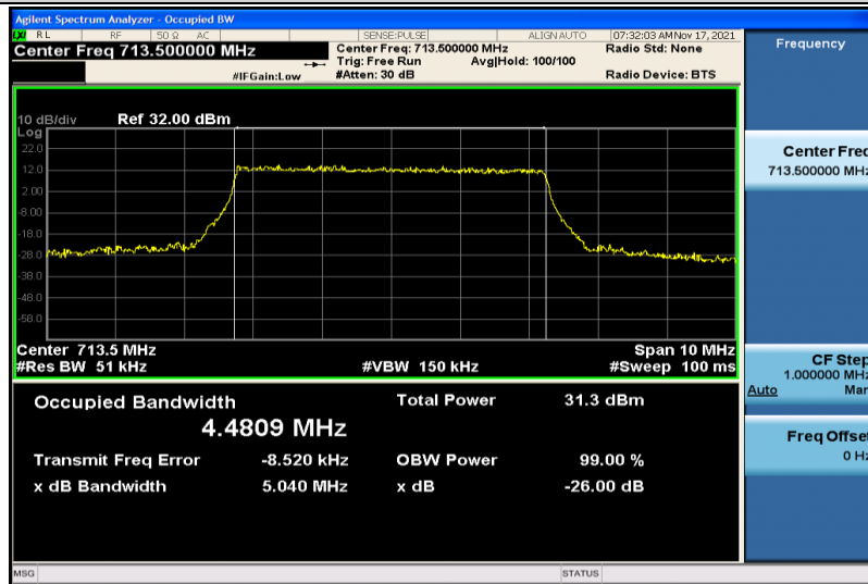
Band12-5MHz-QPSK-23155-25RB#0-4.4809
