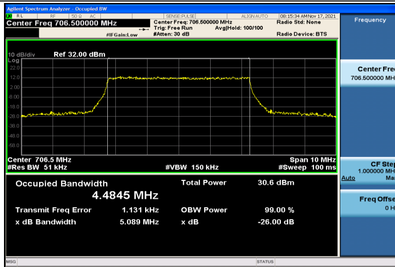
Band17-5MHz-16QAM-23755-25RB#0-4.4845
