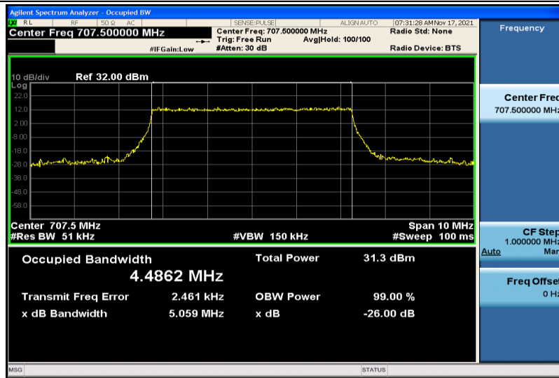
Band12-5MHz-QPSK-23095-25RB#0-4.4862
