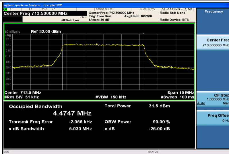
Band17-5MHz-QPSK-23825-25RB#0-4.4747
