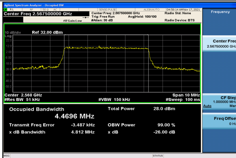
Band7-5MHz-16QAM-21425-25RB#0-4.4696
