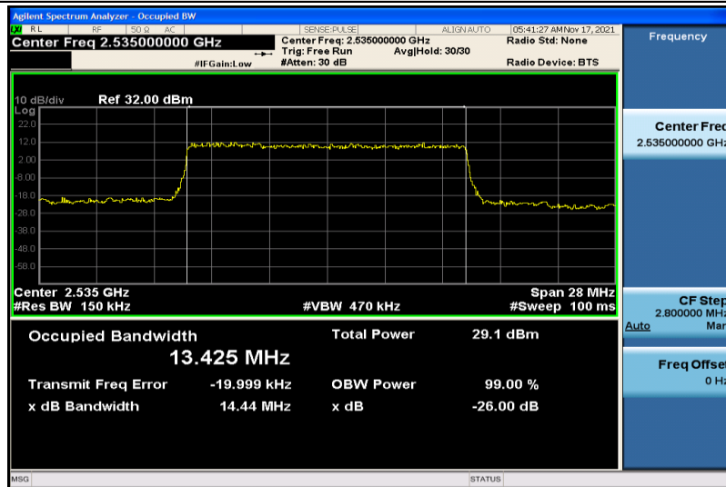
Band7-15MHz-QPSK-21100-75RB#0-13.425
