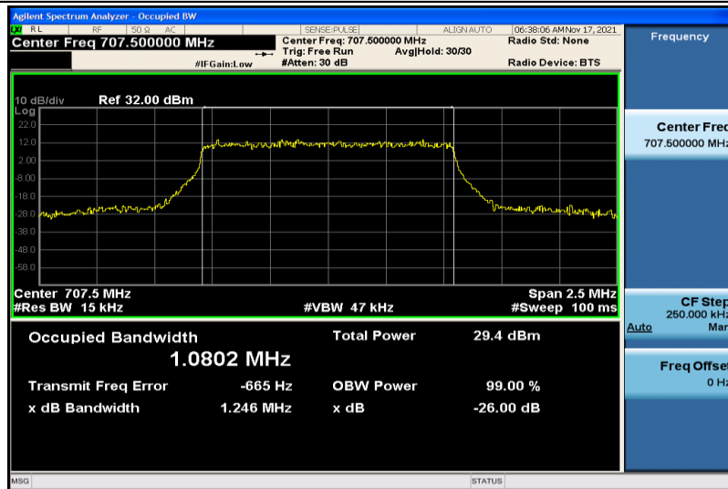
Band12-1.4MHz-16QAM-23095-6RB#0-1.0802
