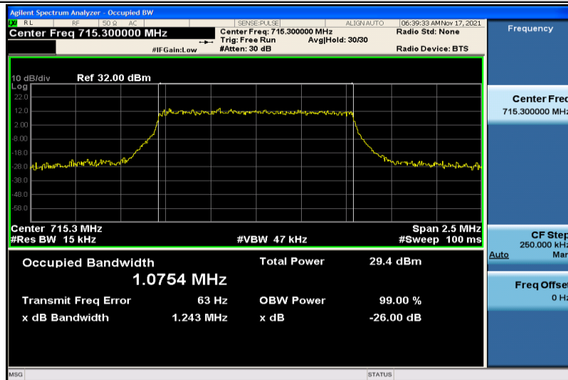
Band12-1.4MHz-16QAM-23173-6RB#0-1.0754
