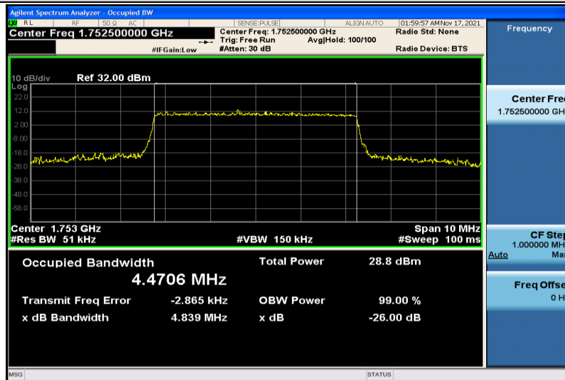
Band4-5MHz-16QAM-20375-25RB#0-4.4706
