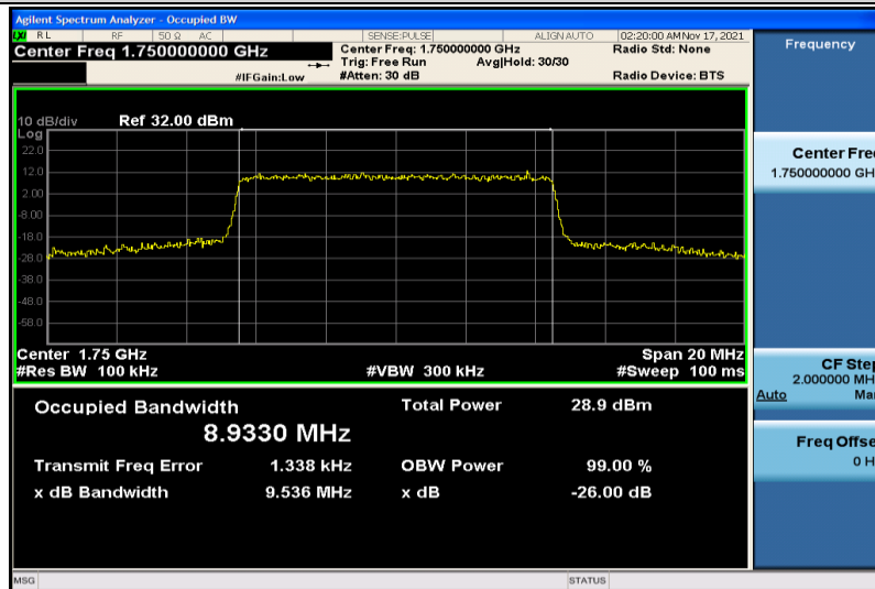
Band4-10MHz-16QAM-20350-50RB#0-8.9330
