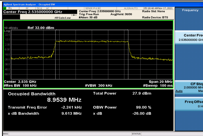
Band7-10MHz-16QAM-21100-50RB#0-8.9539
