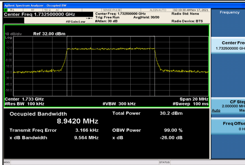
Band4-10MHz-QPSK-20175-50RB#0-8.9420
