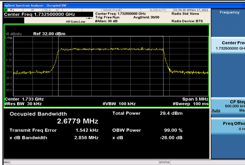
Band4-3MHz-QPSK-20175-15RB#0-2.6779
