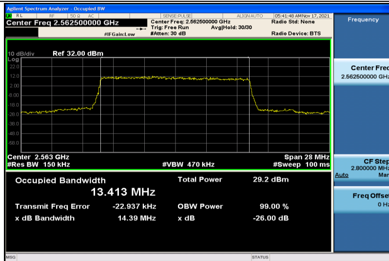
Band7-15MHz-QPSK-21375-75RB#0-13.413
