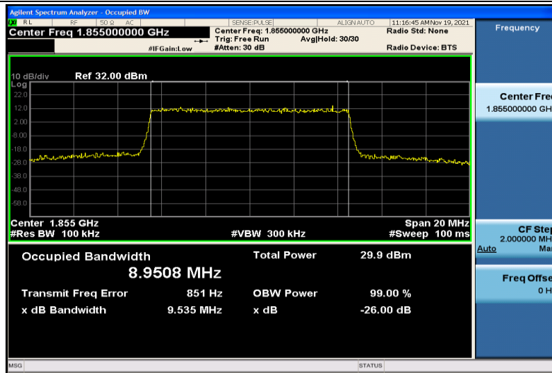
Band2-10MHz-16QAM-18650-50RB#0-8.9508
