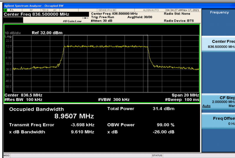
Band5-10MHz-QPSK-20525-50RB#0-8.9507
