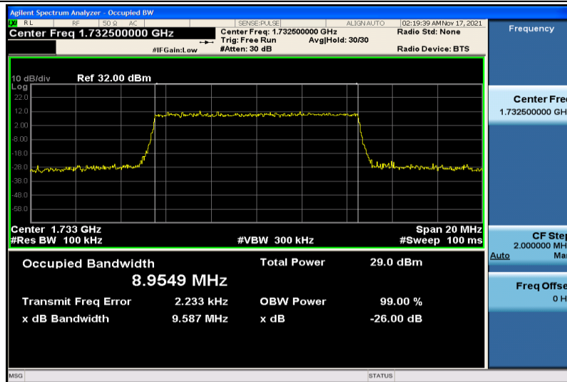
Band4-10MHz-16QAM-20175-50RB#0-8.9549
