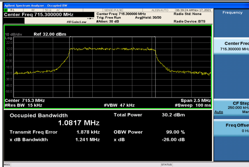
Band12-1.4MHz-QPSK-23173-6RB#0-1.0817
