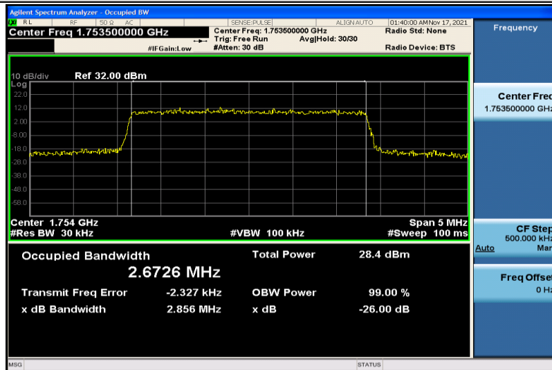
Band4-3MHz-16QAM-20385-15RB#0-2.6726
