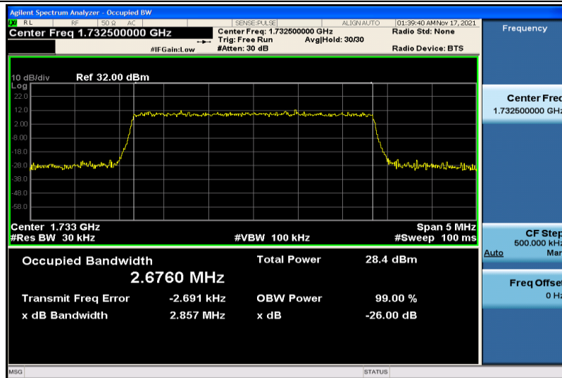
Band4-3MHz-16QAM-20175-15RB#0-2.6760
