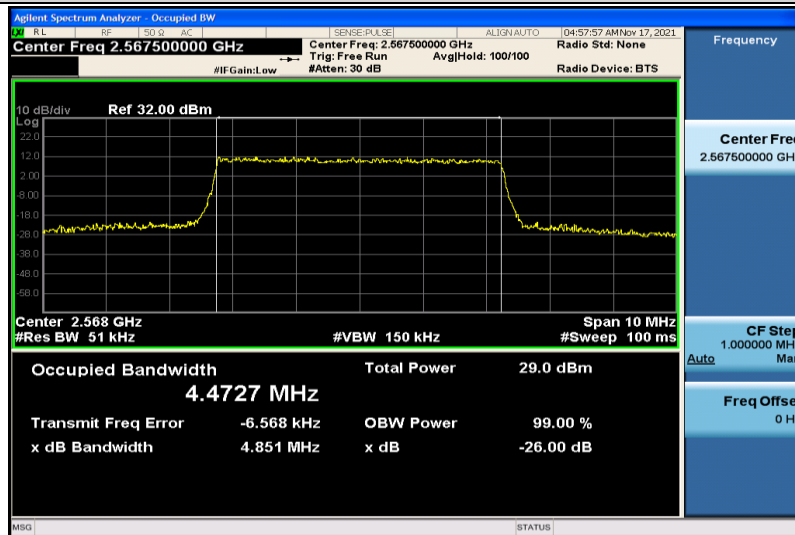
Band7-5MHz-QPSK-21425-25RB#0-4.4727
