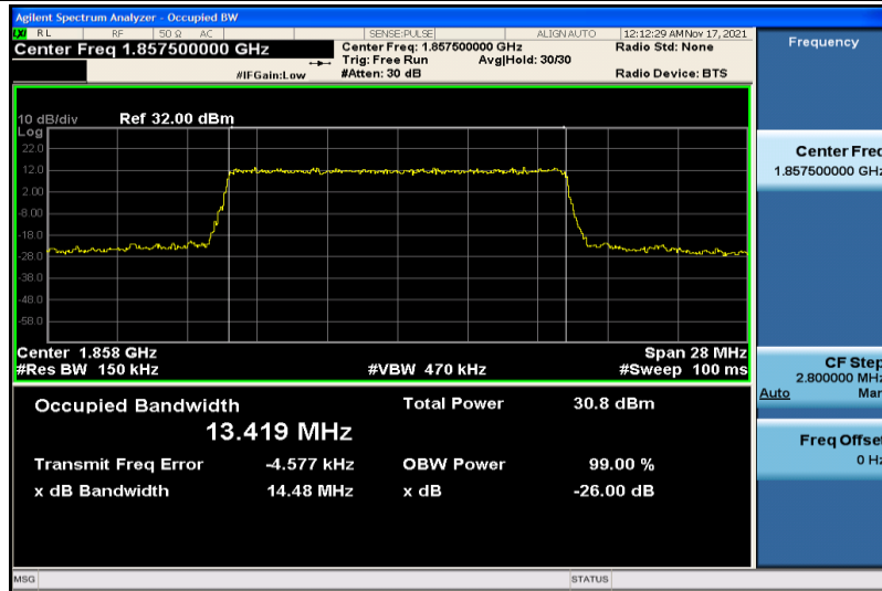
Band2-15MHz-QPSK-18675-75RB#0-13.419
