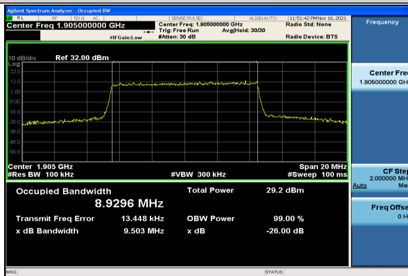
Band2-10MHz-16QAM-19150-50RB#0-8.9296
