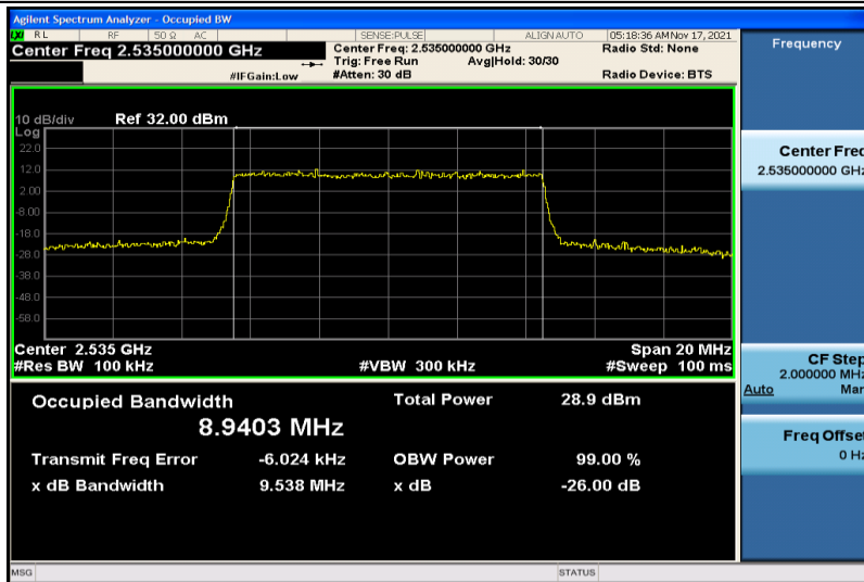
Band7-10MHz-QPSK-21100-50RB#0-8.9403
