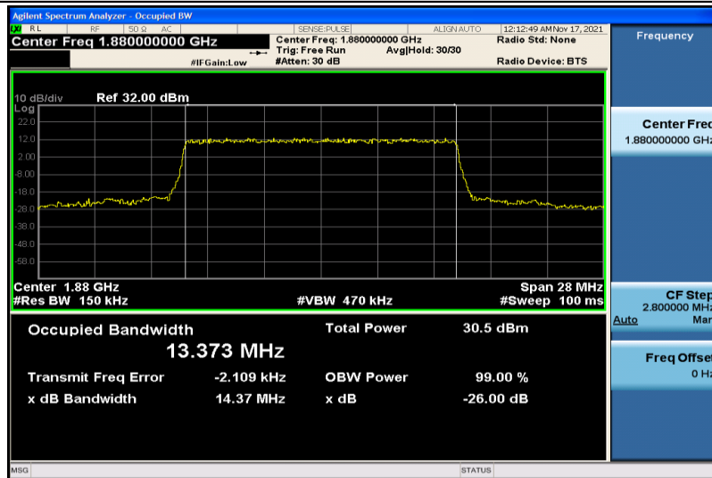
Band2-15MHz-QPSK-18900-75RB#0-13.373
