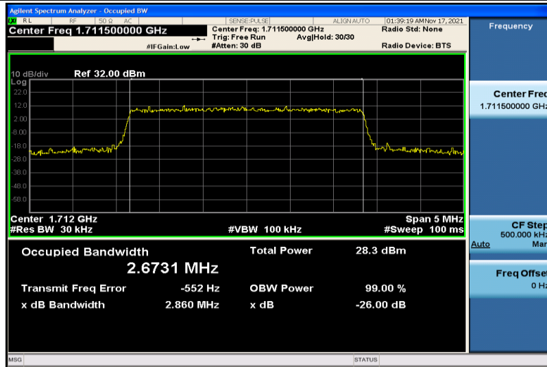
Band4-3MHz-16QAM-19965-15RB#0-2.6731
