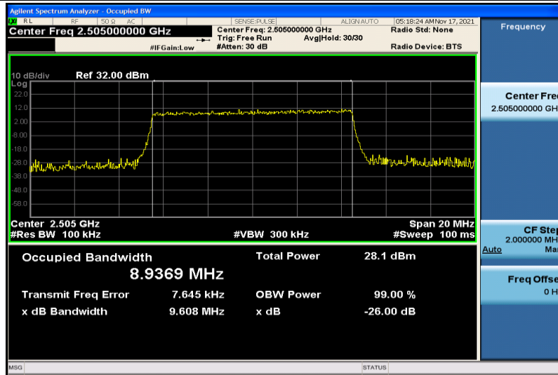
Band7-10MHz-16QAM-20800-50RB#0-8.9369
