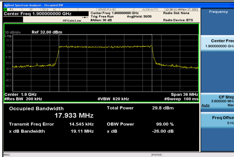
Band2-20MHz-16QAM-19100-100RB#0-17.933
