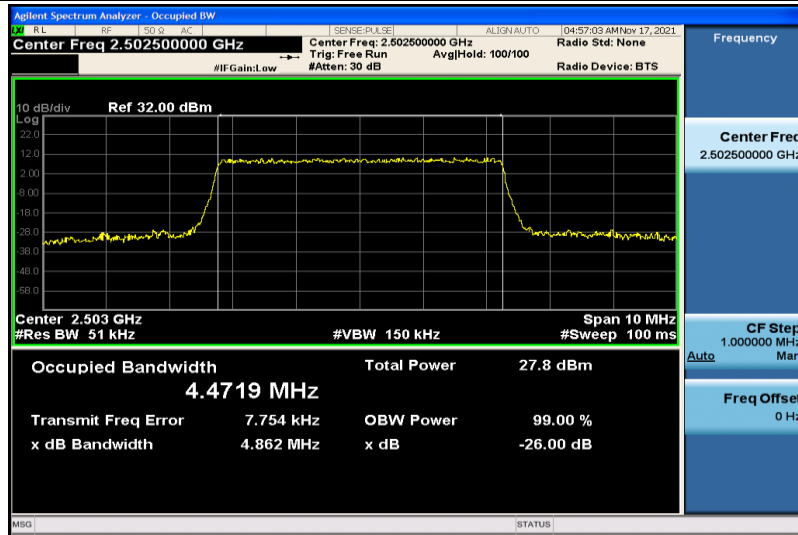
Band7-5MHz-16QAM-20775-25RB#0-4.4719
