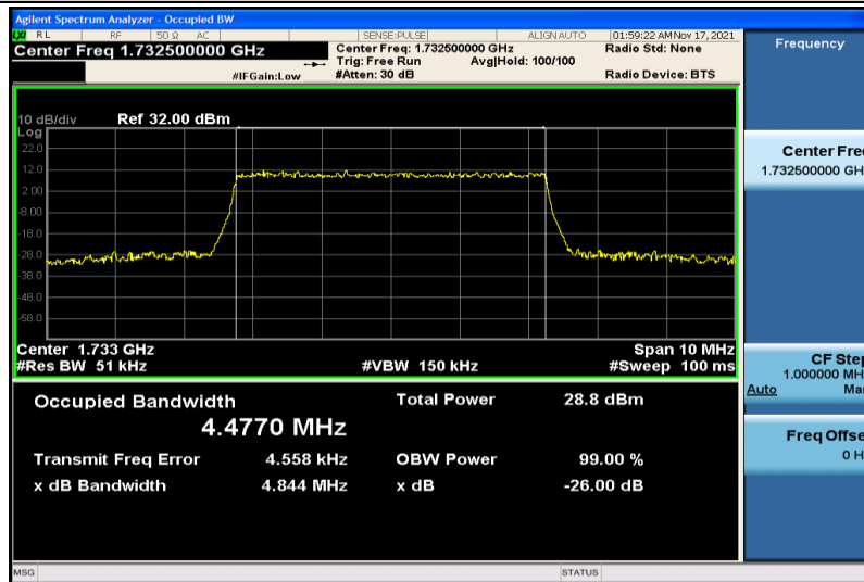
Band4-5MHz-16QAM-20175-25RB#0-4.4770
