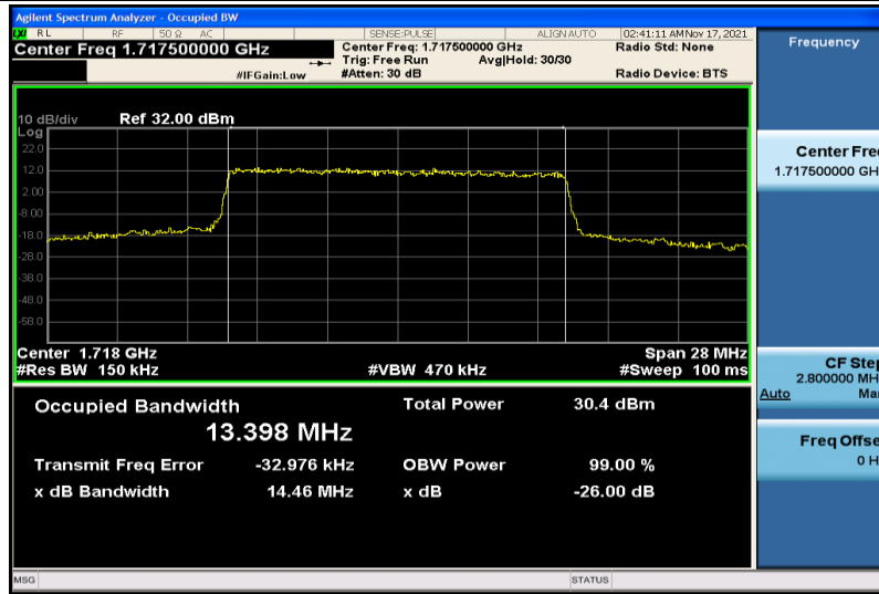
Band4-15MHz-QPSK-20025-75RB#0-13.398
