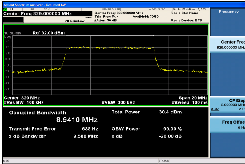
Band5-10MHz-16QAM-20450-50RB#0-8.9410
