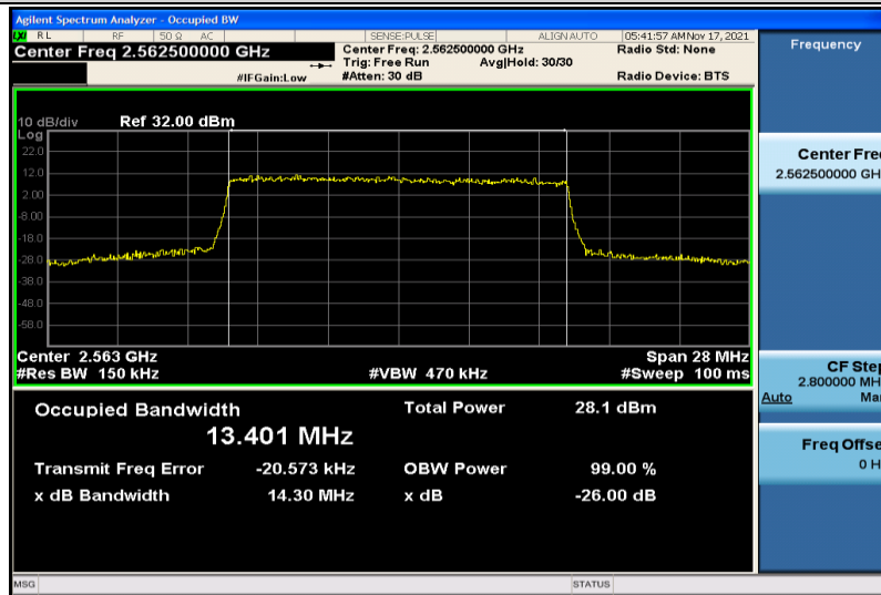
Band7-15MHz-16QAM-21375-75RB#0-13.401
