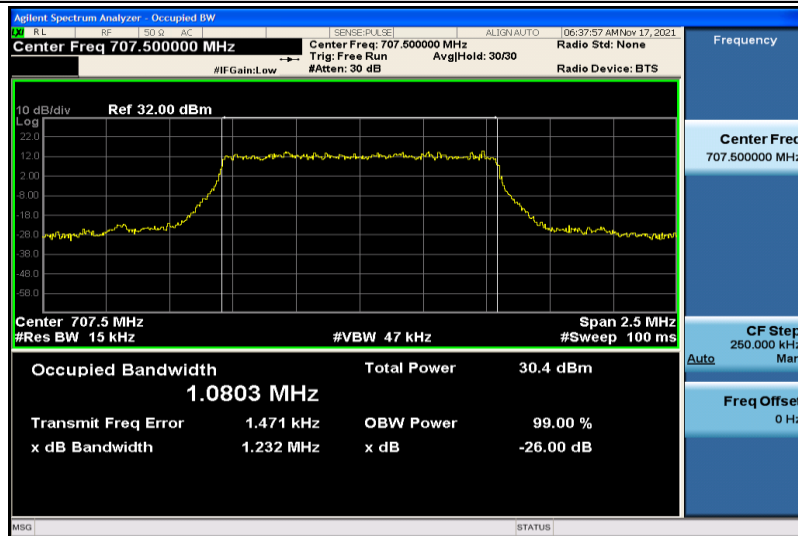
Band12-1.4MHz-QPSK-23095-6RB#0-1.0803
