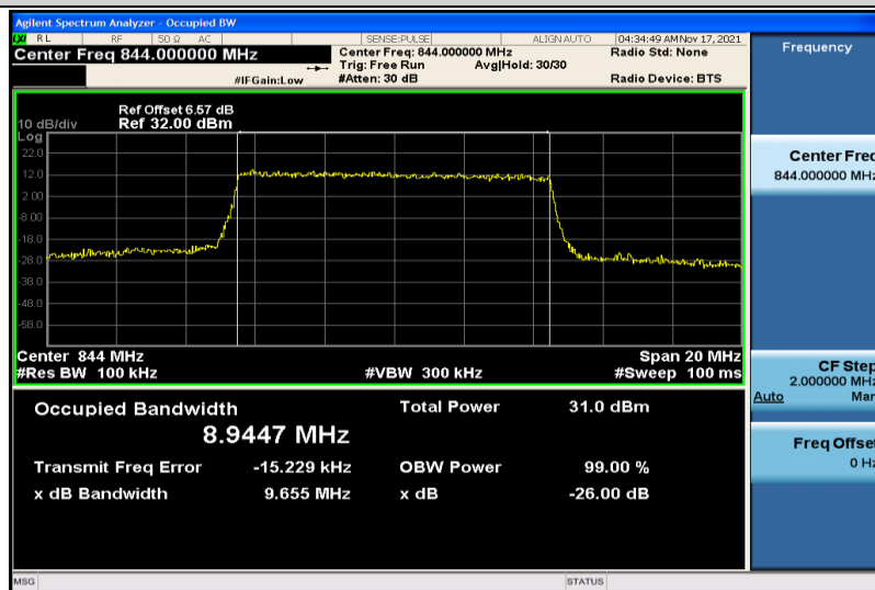
Band5-10MHz-QPSK-20600-50RB#0-8.9447
