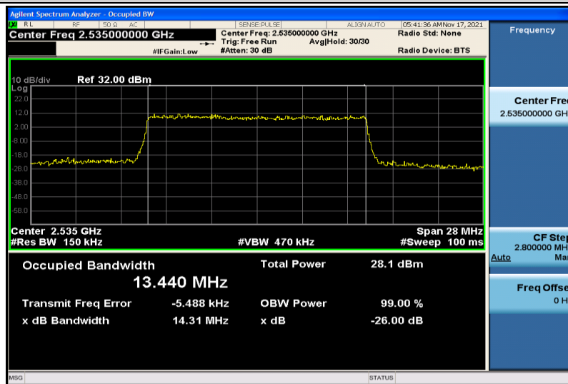
Band7-15MHz-16QAM-21100-75RB#0-13.440
