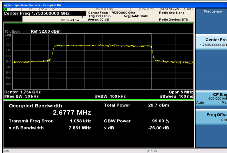
Band4-3MHz-QPSK-20385-15RB#0-2.6777
