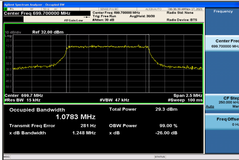
Band12-1.4MHz-16QAM-23017-6RB#0-1.0783
