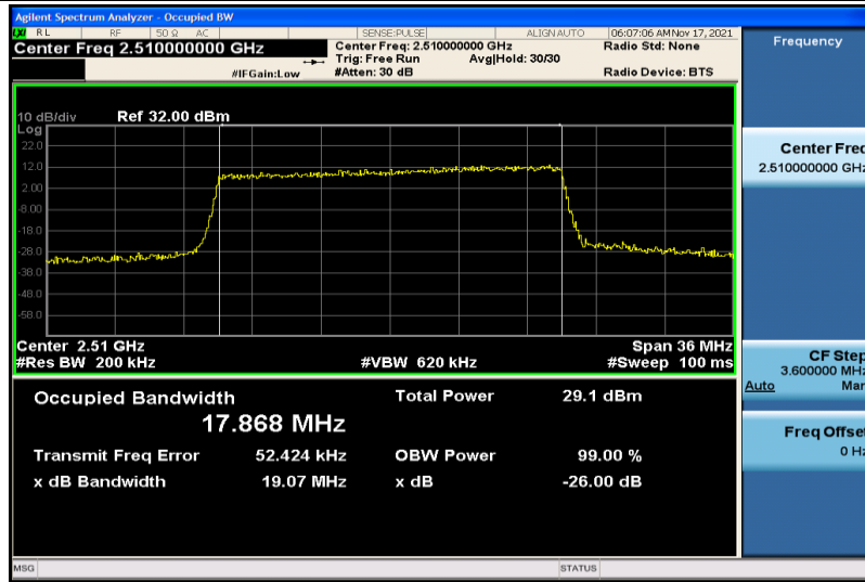
Band7-20MHz-QPSK-20850-100RB#0-17.868
