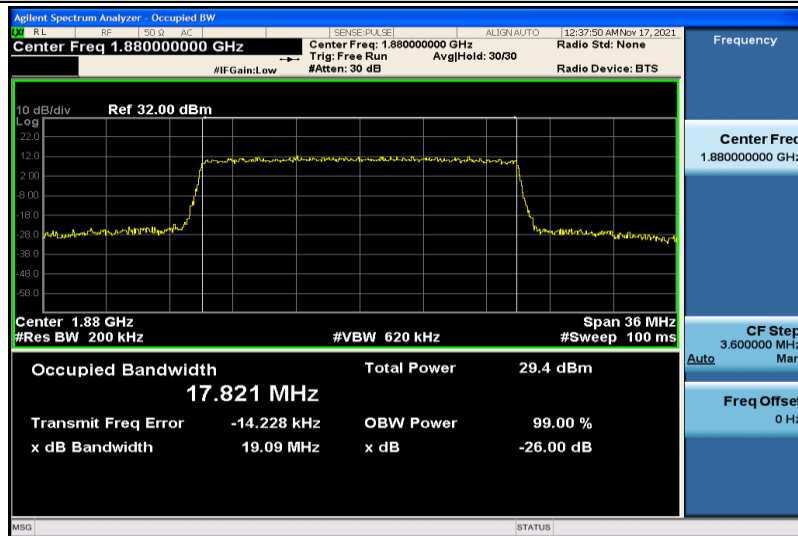
Band2-20MHz-16QAM-18900-100RB#0-17.821
