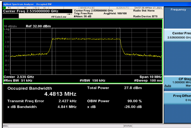
Band7-5MHz-16QAM-21100-25RB#0-4.4813
