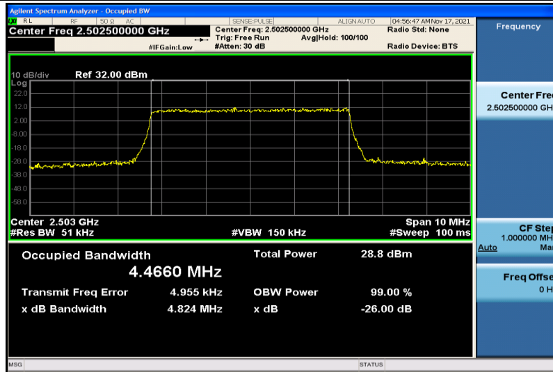
Band7-5MHz-QPSK-20775-25RB#0-4.4660
