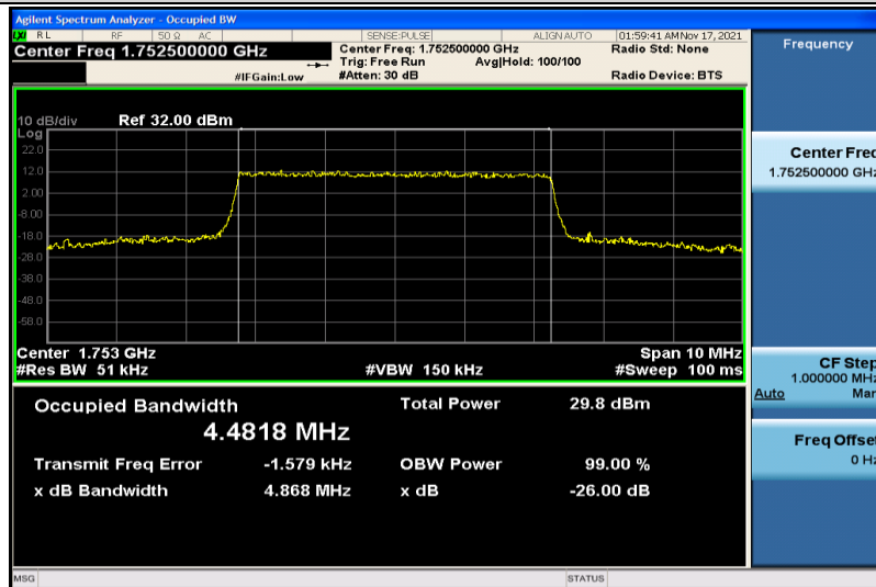
Band4-5MHz-QPSK-20375-25RB#0-4.4818
