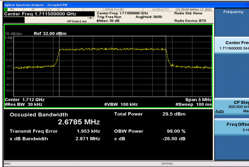
Band4-3MHz-QPSK-19965-15RB#0-2.6785
