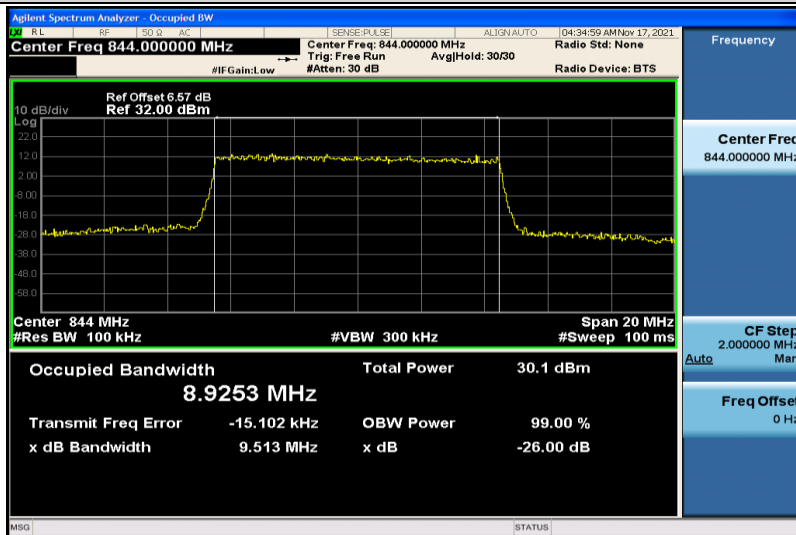
Band5-10MHz-16QAM-20600-50RB#0-8.9253
