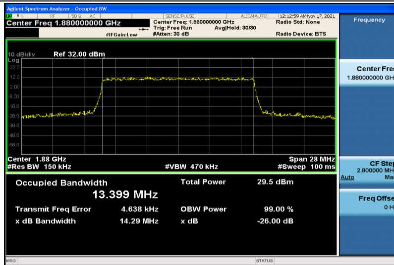
Band2-15MHz-16QAM-18900-75RB#0-13.399
