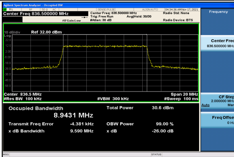
Band5-10MHz-16QAM-20525-50RB#0-8.9431
