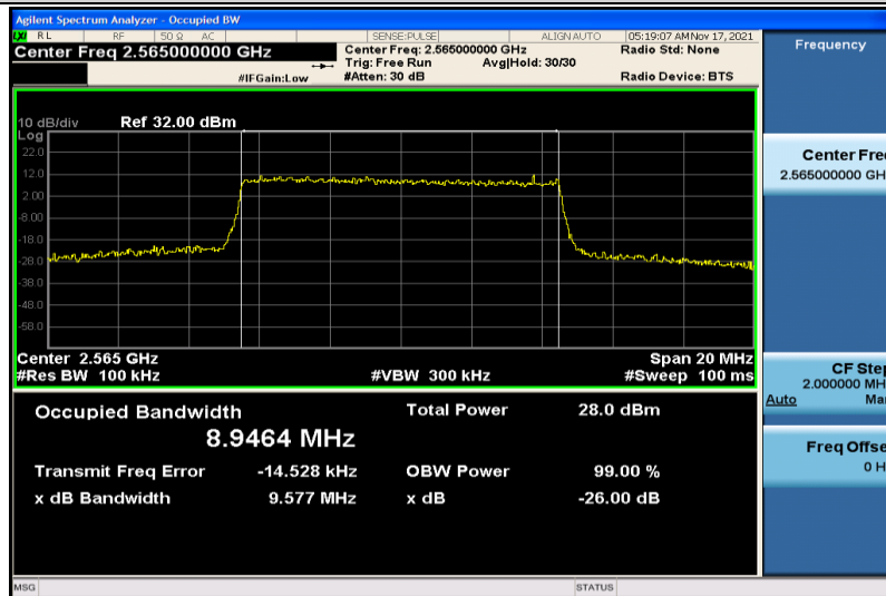
Band7-10MHz-16QAM-21400-50RB#0-8.9464
