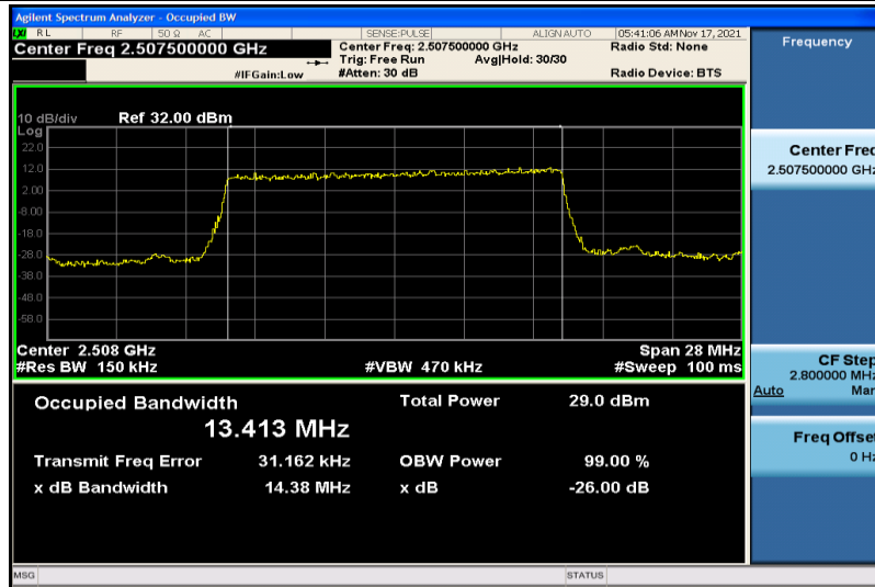
Band7-15MHz-QPSK-20825-75RB#0-13.413
