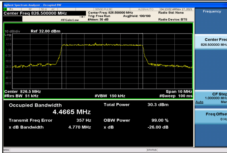
Band5-5MHz-16QAM-20425-25RB#0-4.4665
