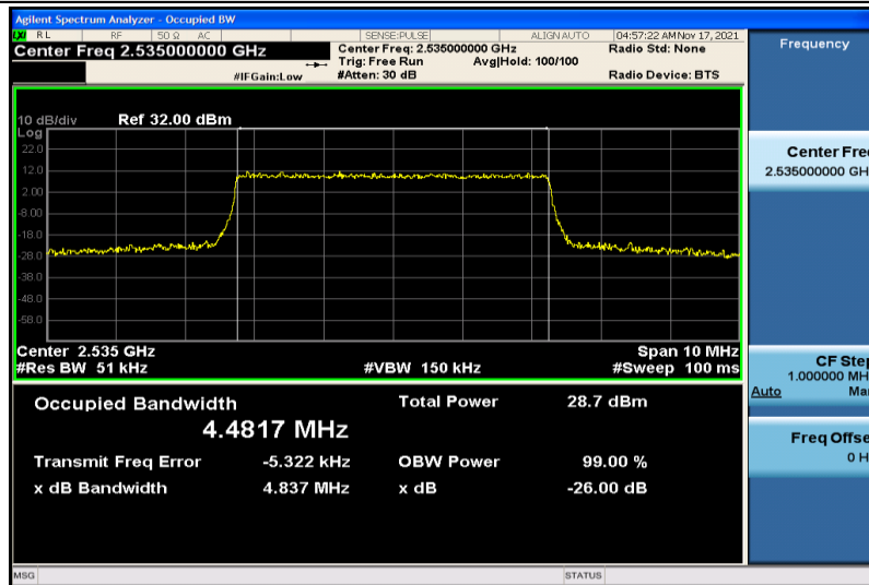
Band7-5MHz-QPSK-21100-25RB#0-4.4817
