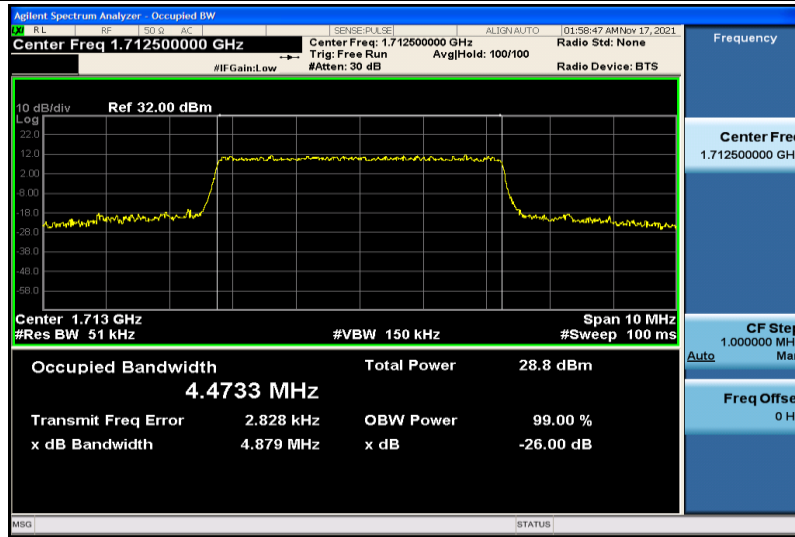
Band4-5MHz-16QAM-19975-25RB#0-4.4733
