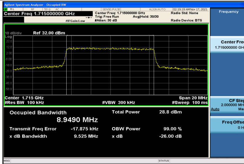
Band4-10MHz-16QAM-20000-50RB#0-8.9490
