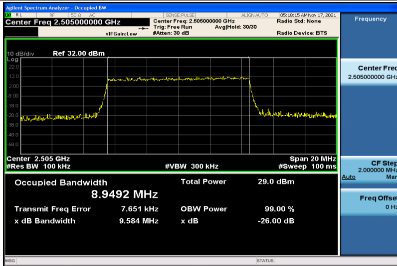
Band7-10MHz-QPSK-20800-50RB#0-8.9492
