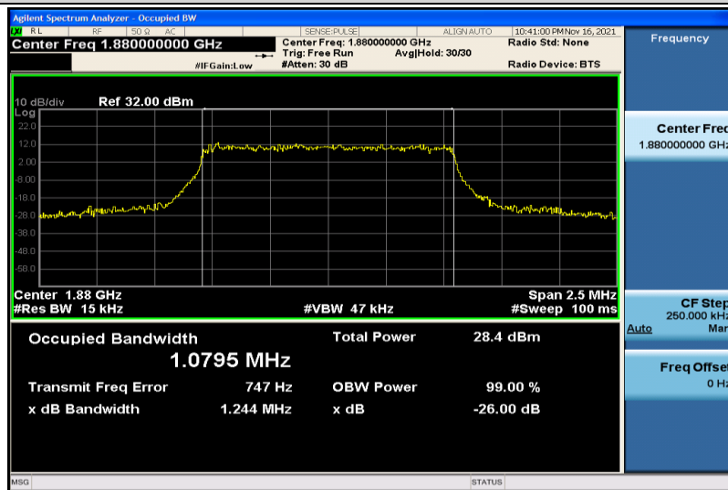
Band2-1.4MHz-16QAM-18900-6RB#0-1.0795
