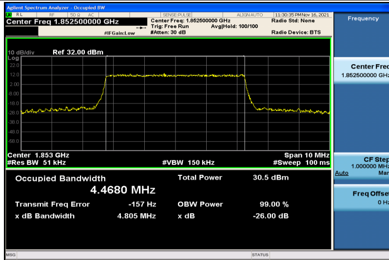
Band2-5MHz-QPSK-18625-25RB#0-4.4680
