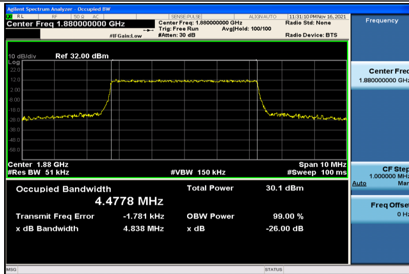
Band2-5MHz-QPSK-18900-25RB#0-4.4778
