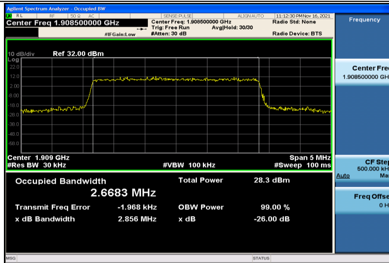
Band2-3MHz-16QAM-19185-15RB#0-2.6683
