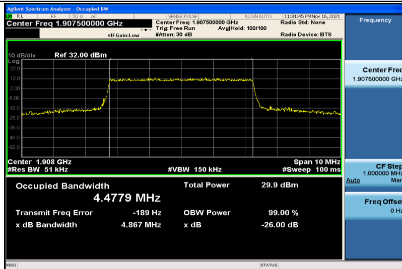
Band2-5MHz-QPSK-19175-25RB#0-4.4779
