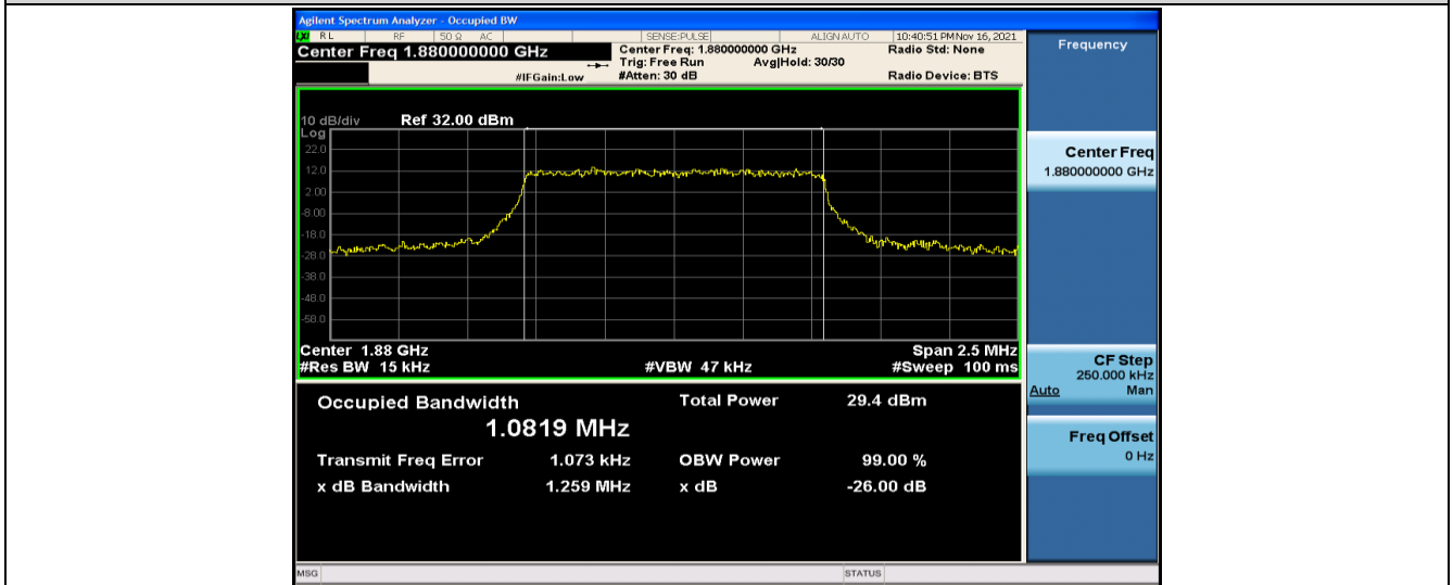
Band2-1.4MHz-QPSK-18900-6RB#0-1.0819
