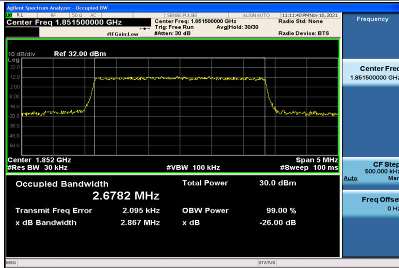
Band2-3MHz-QPSK-18615-15RB#0-2.6782
