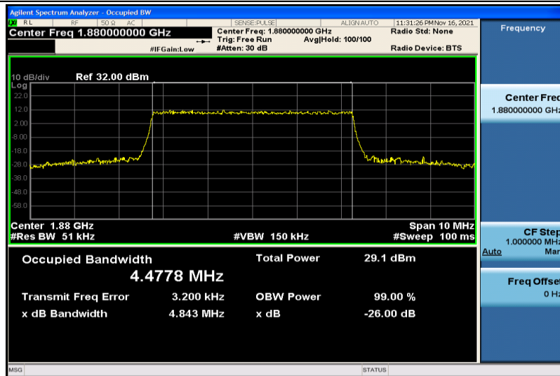
Band2-5MHz-16QAM-18900-25RB#0-4.4778
