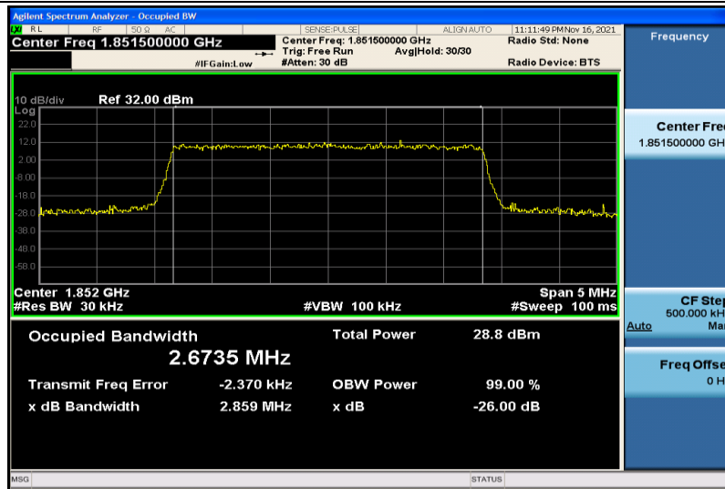
Band2-3MHz-16QAM-18615-15RB#0-2.6735
