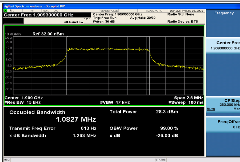
Band2-1.4MHz-16QAM-19193-6RB#0-1.0827
