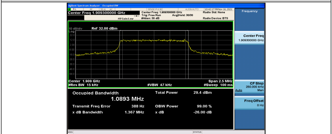
Band2-1.4MHz-QPSK-19193-6RB#0-1.0893
