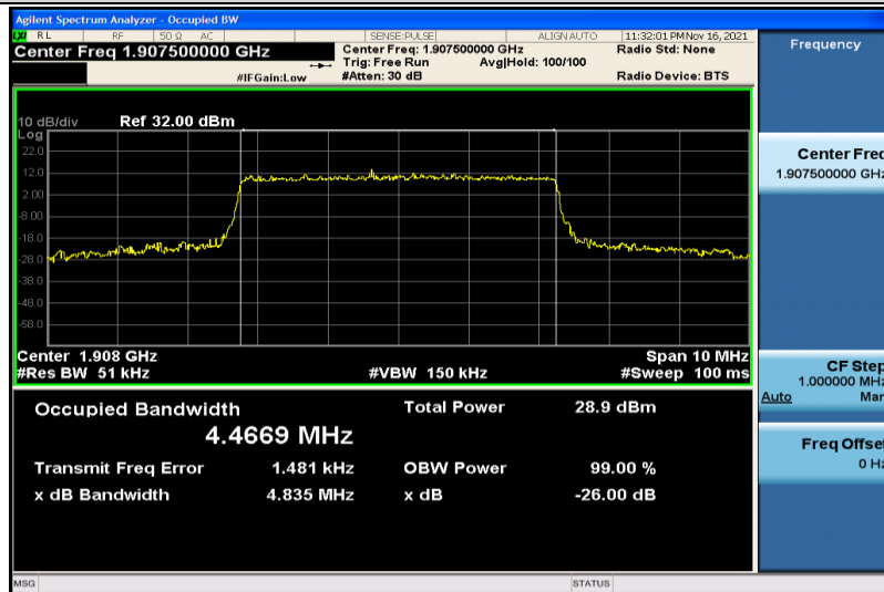
Band2-5MHz-16QAM-19175-25RB#0-4.4669
