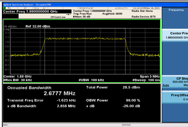
Band2-3MHz-16QAM-18900-15RB#0-2.6777
