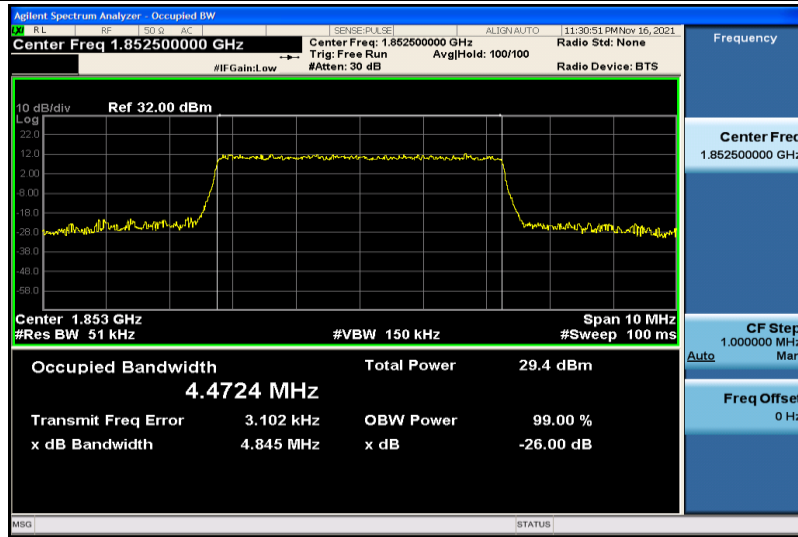
Band2-5MHz-16QAM-18525-25RB#0-4.4724
