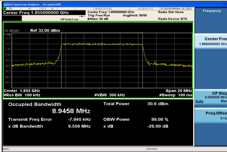
Band2-10MHz-QPSK-18650-50RB#0-8.9458
