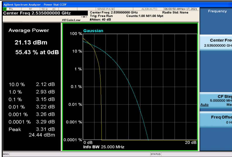
Band7-15MHz-QPSK-21100-1RB#0
