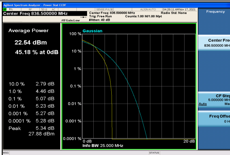
Band5-5MHz-16QAM-20525-1RB#0
