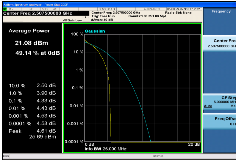
Band7-15MHz-QPSK-20825-1RB#0
