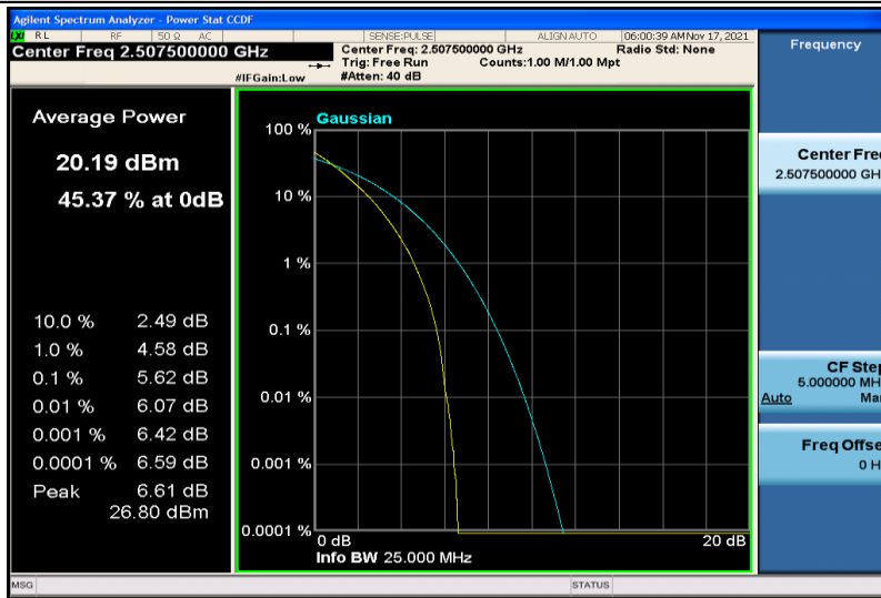
Band7-15MHz-QPSK-20825-75RB#0
