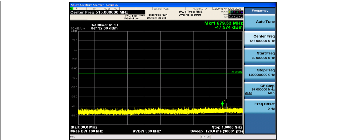
Band2-1.4MHz-QPSK-18607-1RB#0-30~1000MHz
