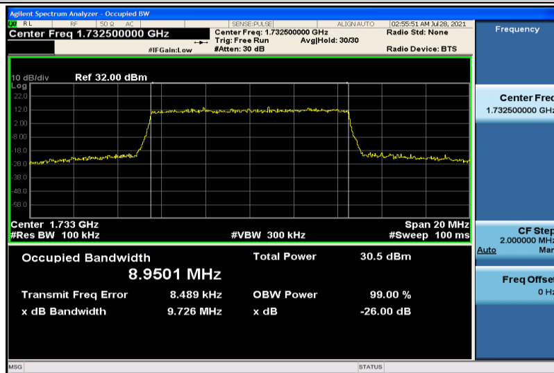
Band4-10MHz-QPSK-20175-50RB#0-8.9501
