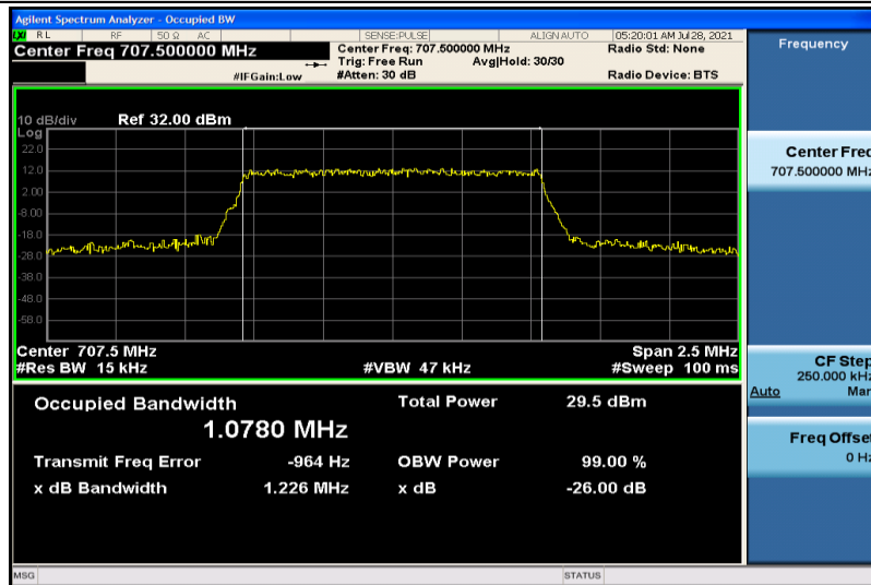
Band12-1.4MHz-QPSK-23095-6RB#0-1.0780
