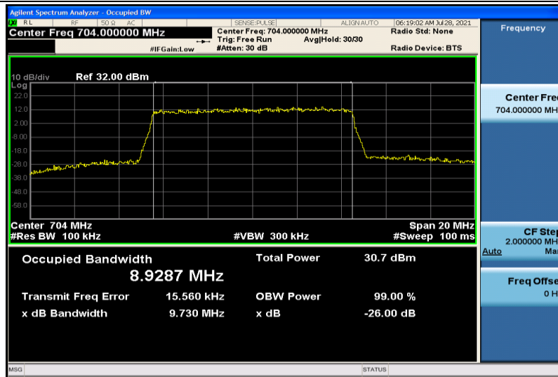
Band12-10MHz-QPSK-23060-50RB#0-8.9287
