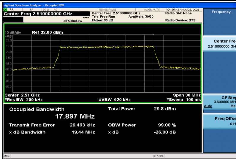
Band7-20MHz-16QAM-20850-100RB#0-17.897
