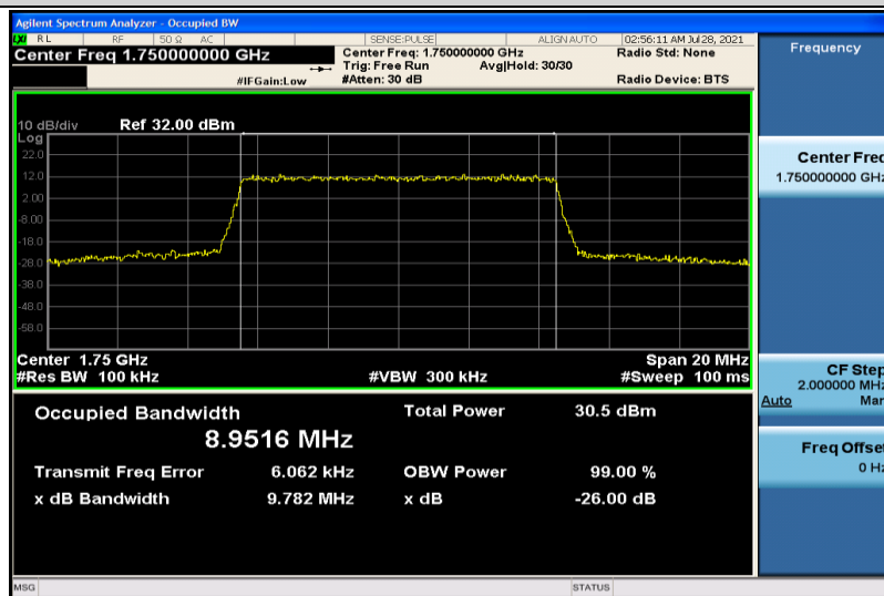
Band4-10MHz-QPSK-20350-50RB#0-8.9516
