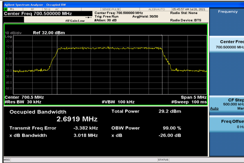
Band12-3MHz-16QAM-23025-15RB#0-2.6919
