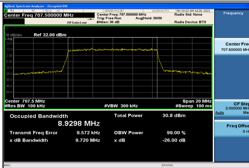
Band12-10MHz-QPSK-23095-50RB#0-8.9298
