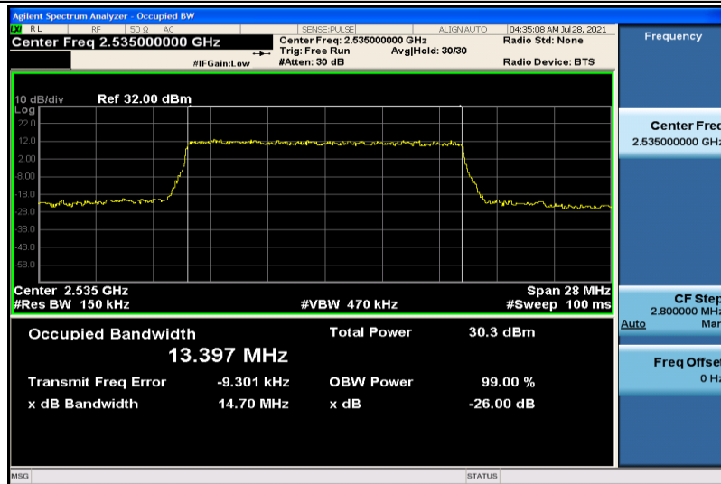
Band7-15MHz-QPSK-21100-75RB#0-13.397
