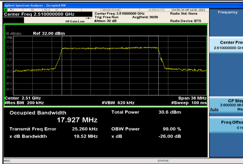
Band7-20MHz-QPSK-20850-100RB#0-17.927
