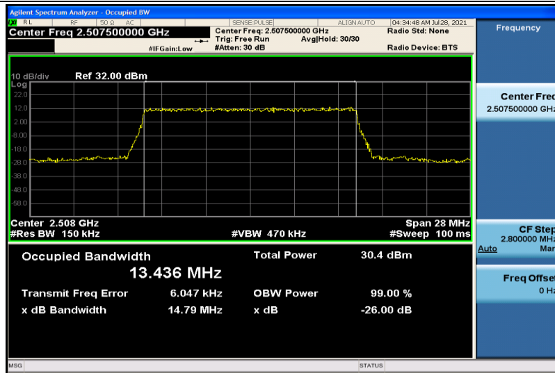
Band7-15MHz-QPSK-20825-75RB#0-13.436
