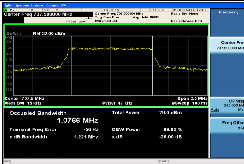
Band12-1.4MHz-16QAM-23095-6RB#0-1.0766
