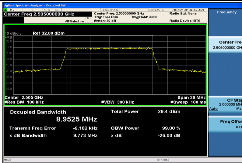
Band7-10MHz-16QAM-20800-50RB#0-8.9525
