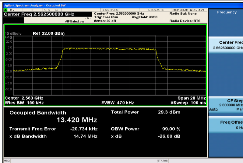
Band7-15MHz-16QAM-21375-75RB#0-13.420
