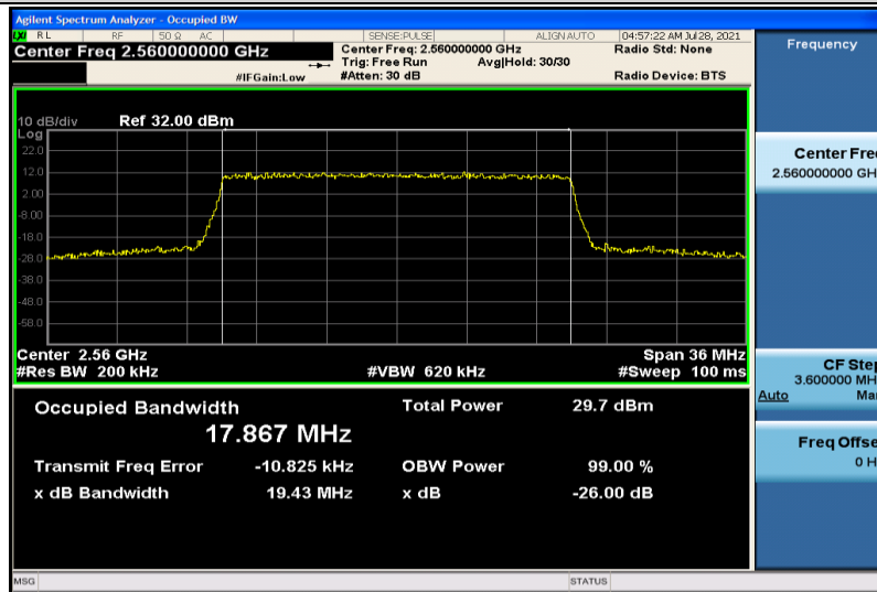
Band7-20MHz-16QAM-21350-100RB#0-17.867
