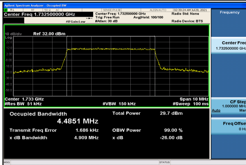
Band4-5MHz-16QAM-20175-25RB#0-4.4851
