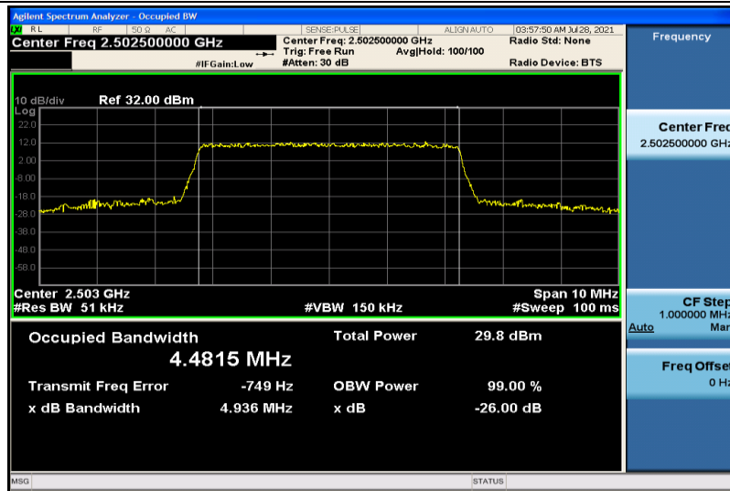
Band7-5MHz-16QAM-20775-25RB#0-4.4815
