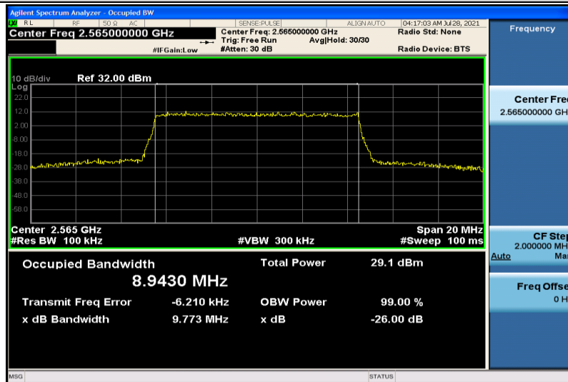
Band7-10MHz-16QAM-21400-50RB#0-8.9430
