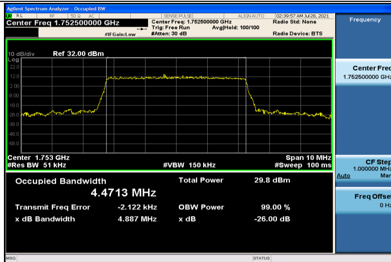
Band4-5MHz-16QAM-20375-25RB#0-4.4713
