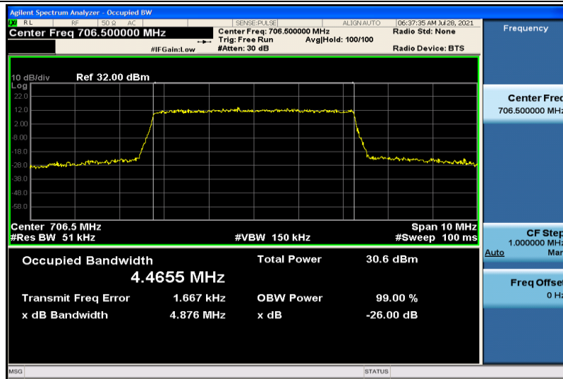
Band17-5MHz-QPSK-23755-25RB#0-4.4655
