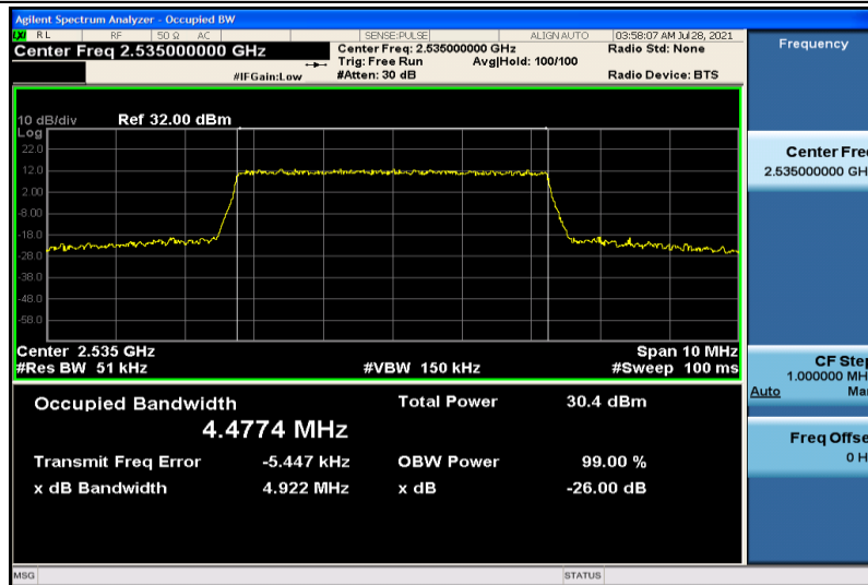
Band7-5MHz-QPSK-21100-25RB#0-4.4774
