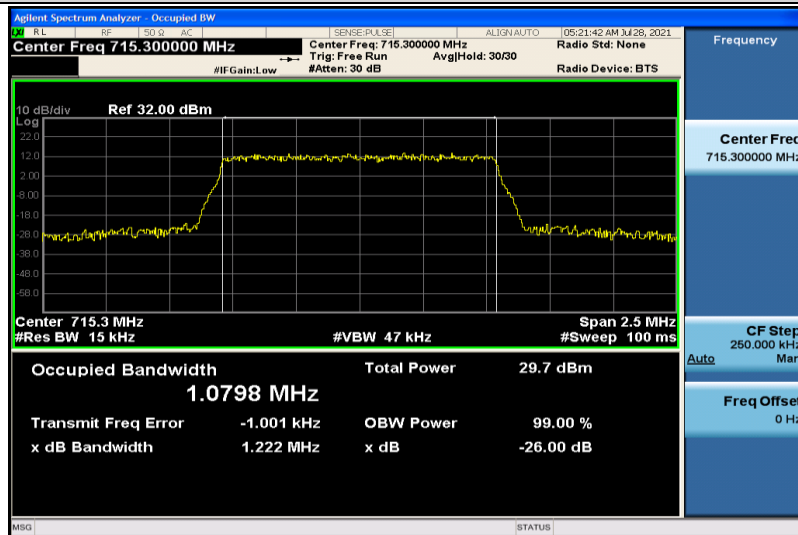
Band12-1.4MHz-QPSK-23173-6RB#0-1.0798
