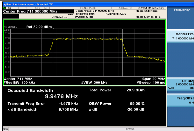
Band12-10MHz-16QAM-23130-50RB#0-8.9476
