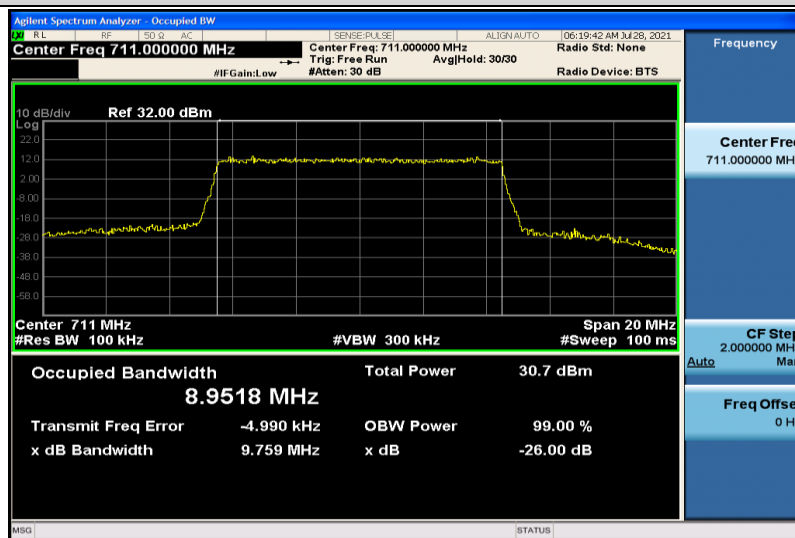
Band12-10MHz-QPSK-23130-50RB#0-8.9518
