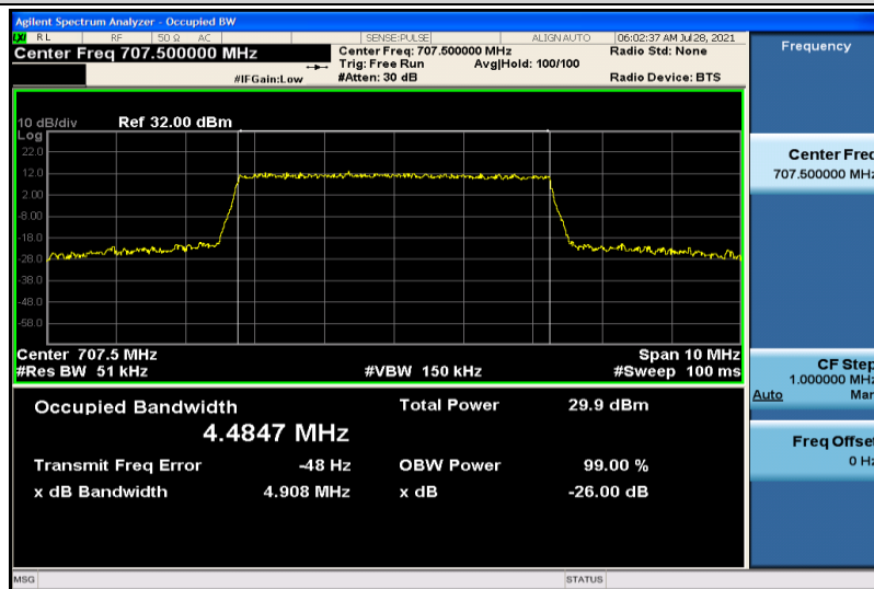
Band12-5MHz-16QAM-23095-25RB#0-4.4847
