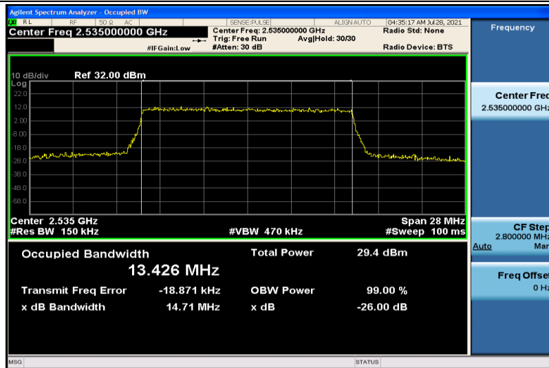
Band7-15MHz-16QAM-21100-75RB#0-13.426
