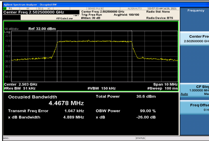
Band7-5MHz-QPSK-20775-25RB#0-4.4678
