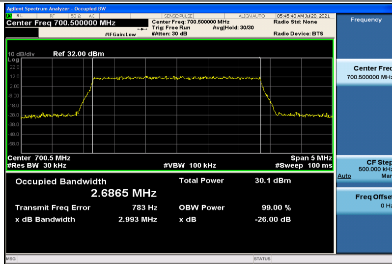
Band12-3MHz-QPSK-23025-15RB#0-2.6865
