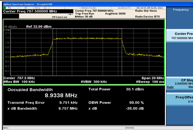
Band12-10MHz-16QAM-23095-50RB#0-8.9338
