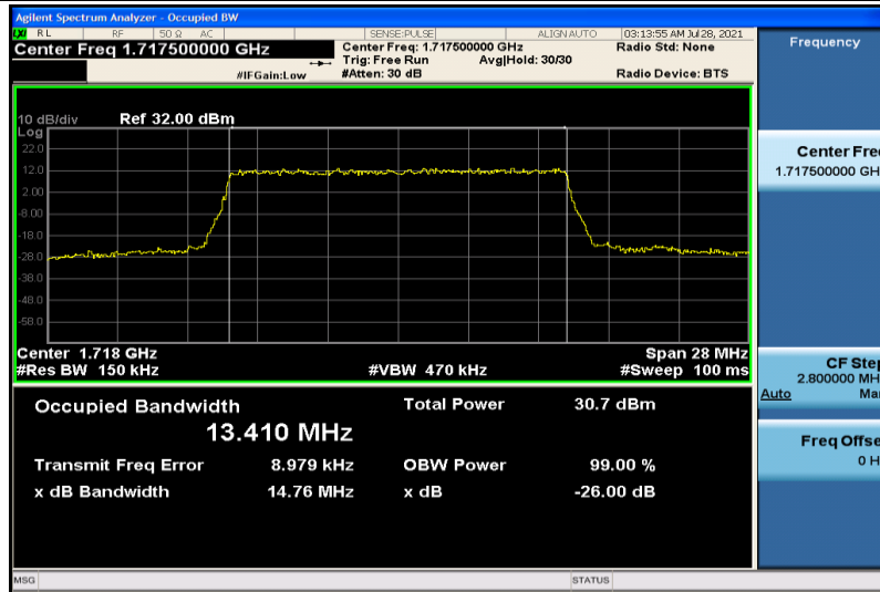
Band4-15MHz-QPSK-20025-75RB#0-13.410
