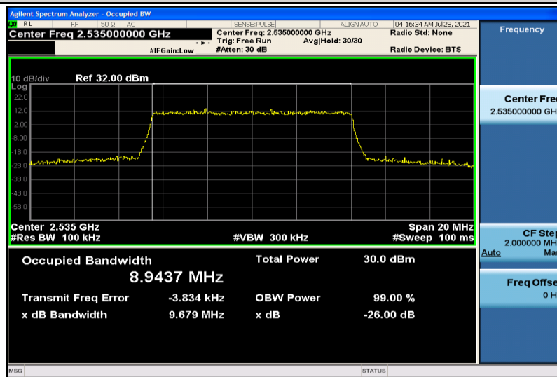
Band7-10MHz-QPSK-21100-50RB#0-8.9437
