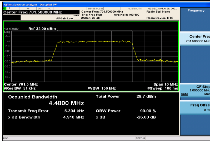
Band12-5MHz-16QAM-23035-25RB#0-4.4800
