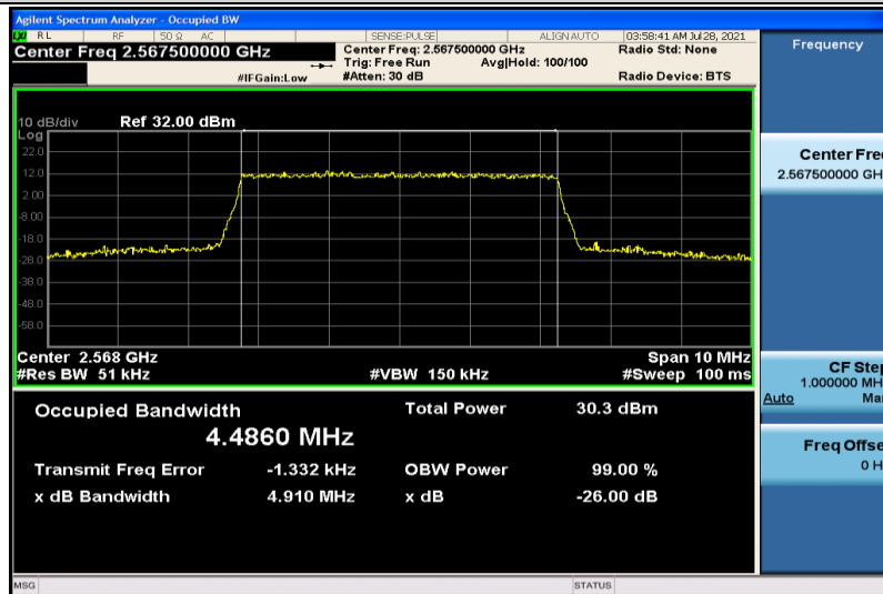
Band7-5MHz-QPSK-21425-25RB#0-4.4860
