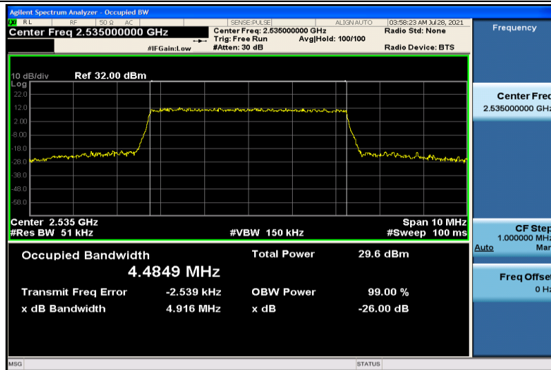
Band7-5MHz-16QAM-21100-25RB#0-4.4849
