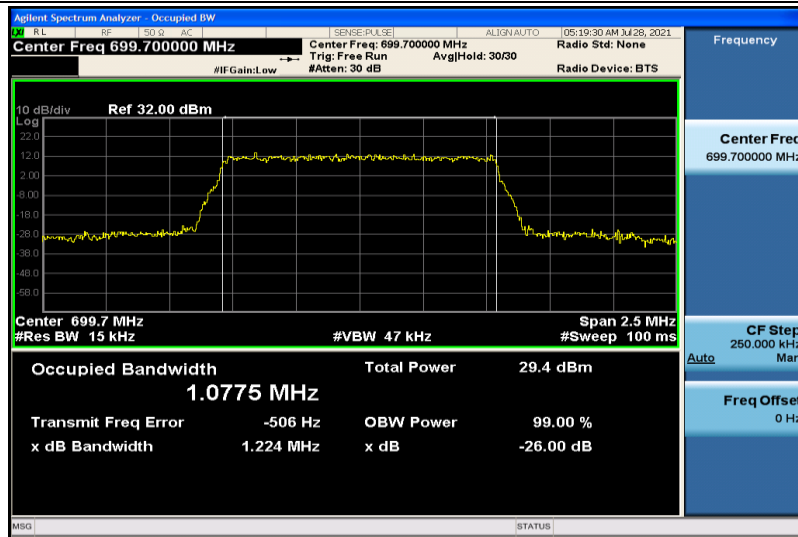
Band12-1.4MHz-QPSK-23017-6RB#0-1.0775
