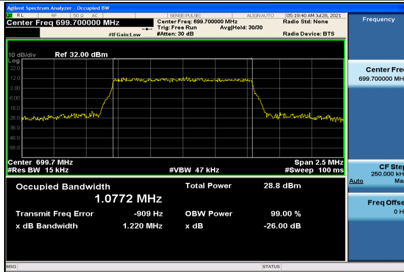
Band12-1.4MHz-16QAM-23017-6RB#0-1.0772
