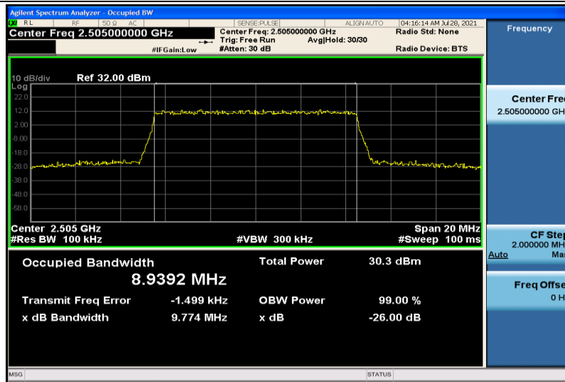
Band7-10MHz-QPSK-20800-50RB#0-8.9392
