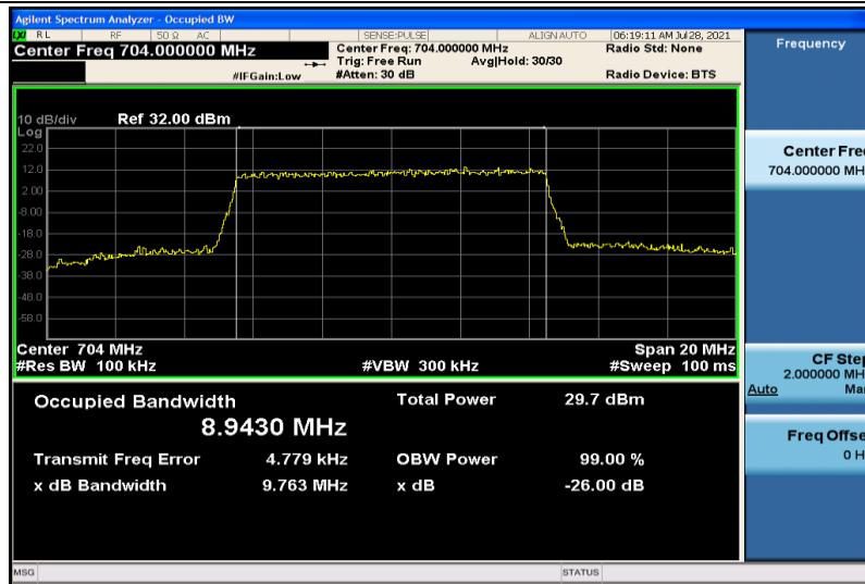
Band12-10MHz-16QAM-23060-50RB#0-8.9430
