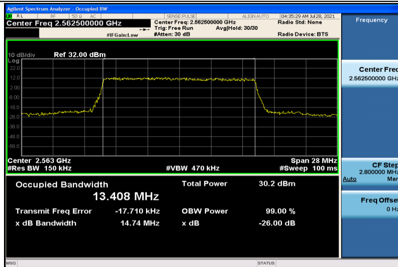
Band7-15MHz-QPSK-21375-75RB#0-13.408
