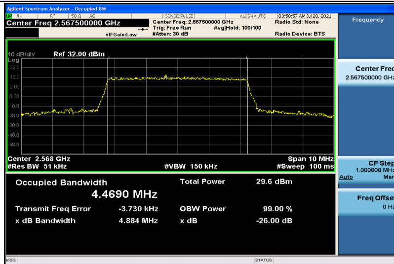
Band7-5MHz-16QAM-21425-25RB#0-4.4690
