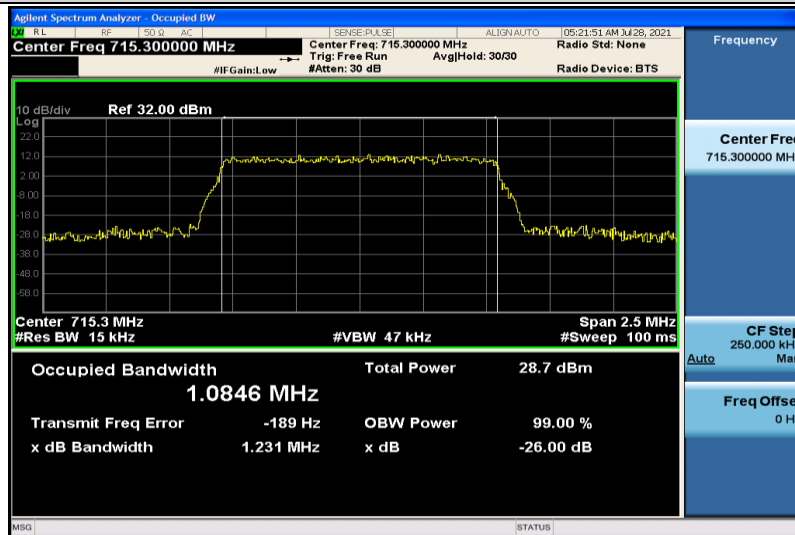
Band12-1.4MHz-16QAM-23173-6RB#0-1.0846
