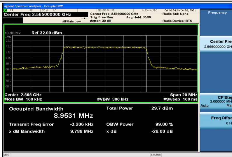
Band7-10MHz-QPSK-21400-50RB#0-8.9531
