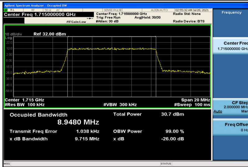
Band4-10MHz-QPSK-20000-50RB#0-8.9480
