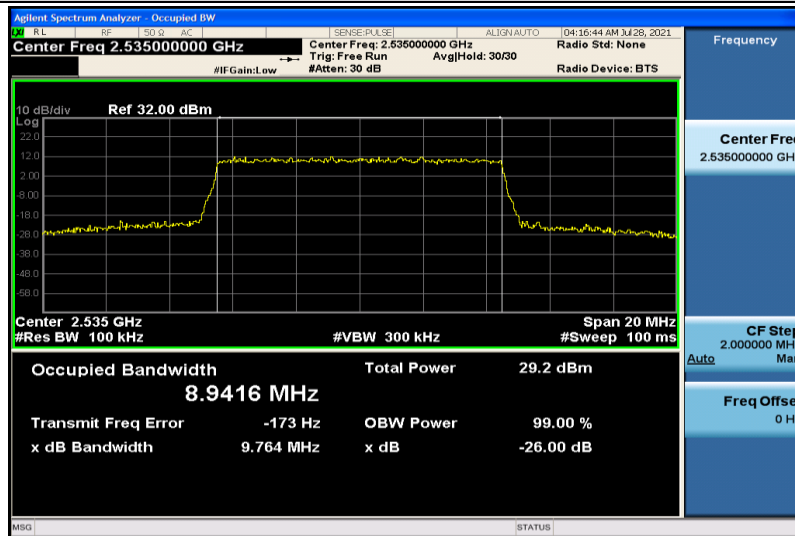
Band7-10MHz-16QAM-21100-50RB#0-8.9416
